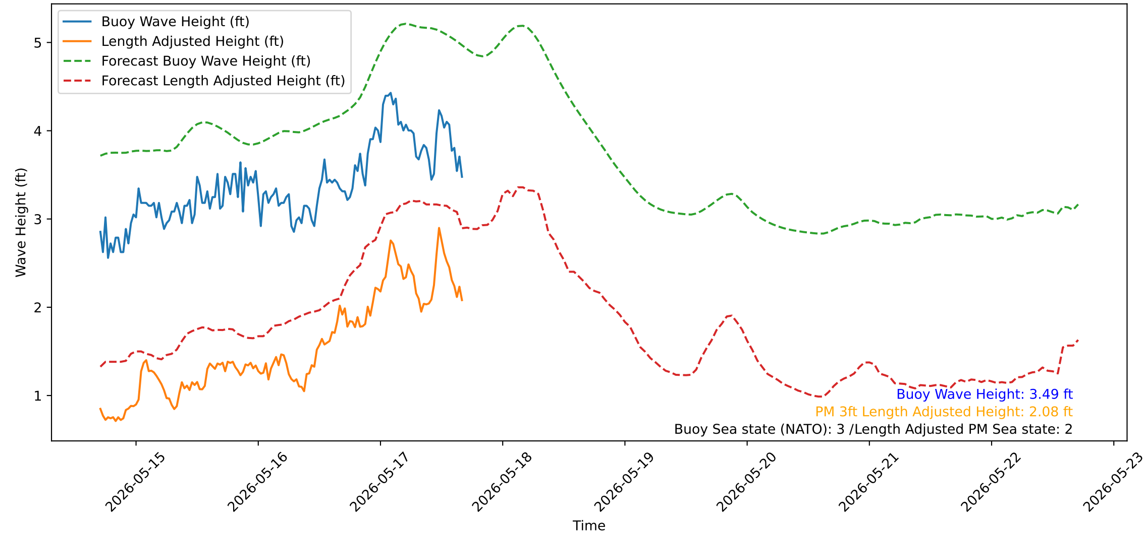
Wave Heights over Time for Green Beach at 2026-05-17 17:01:13
