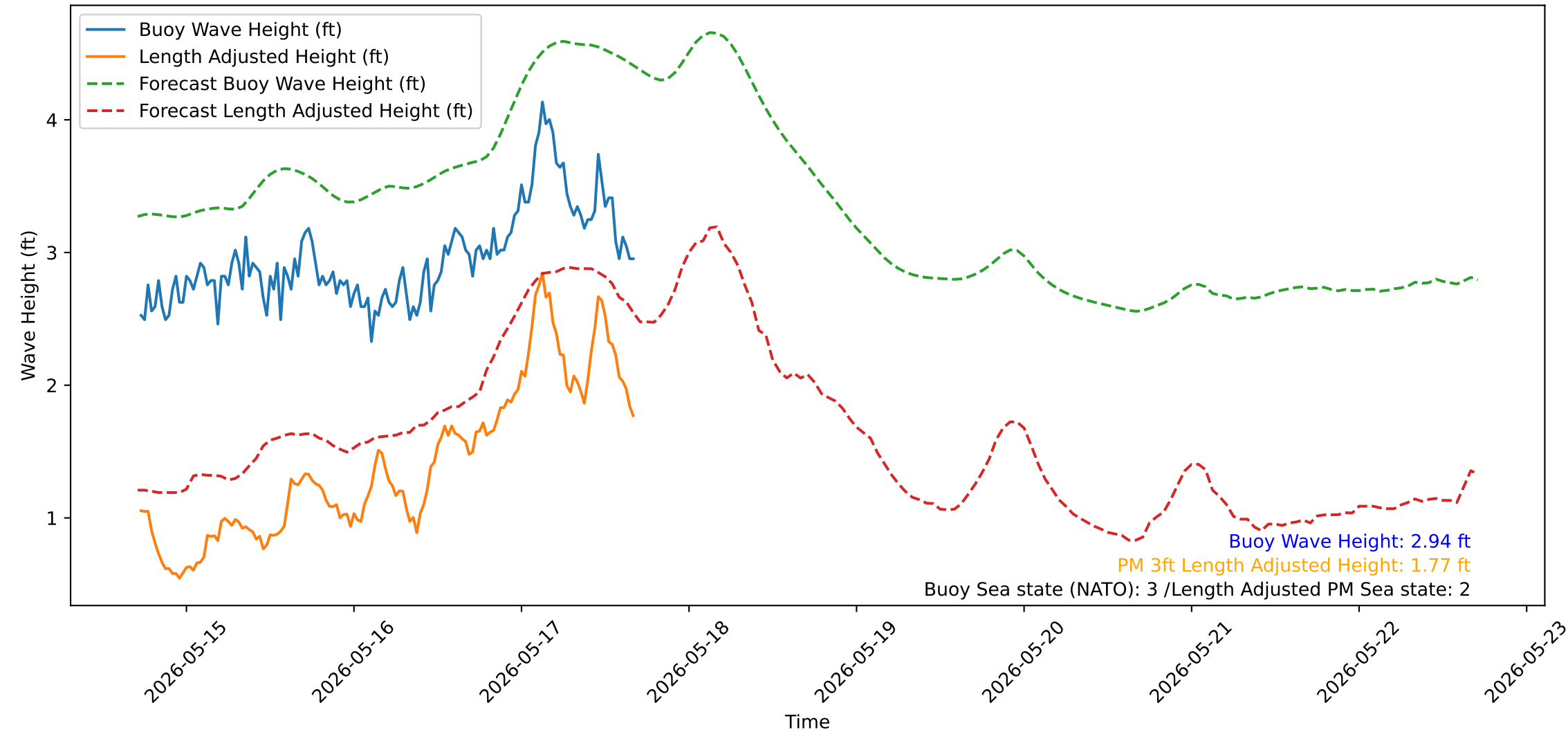
Wave Heights over Time for Red Beach at 2026-05-17 17:00:51
