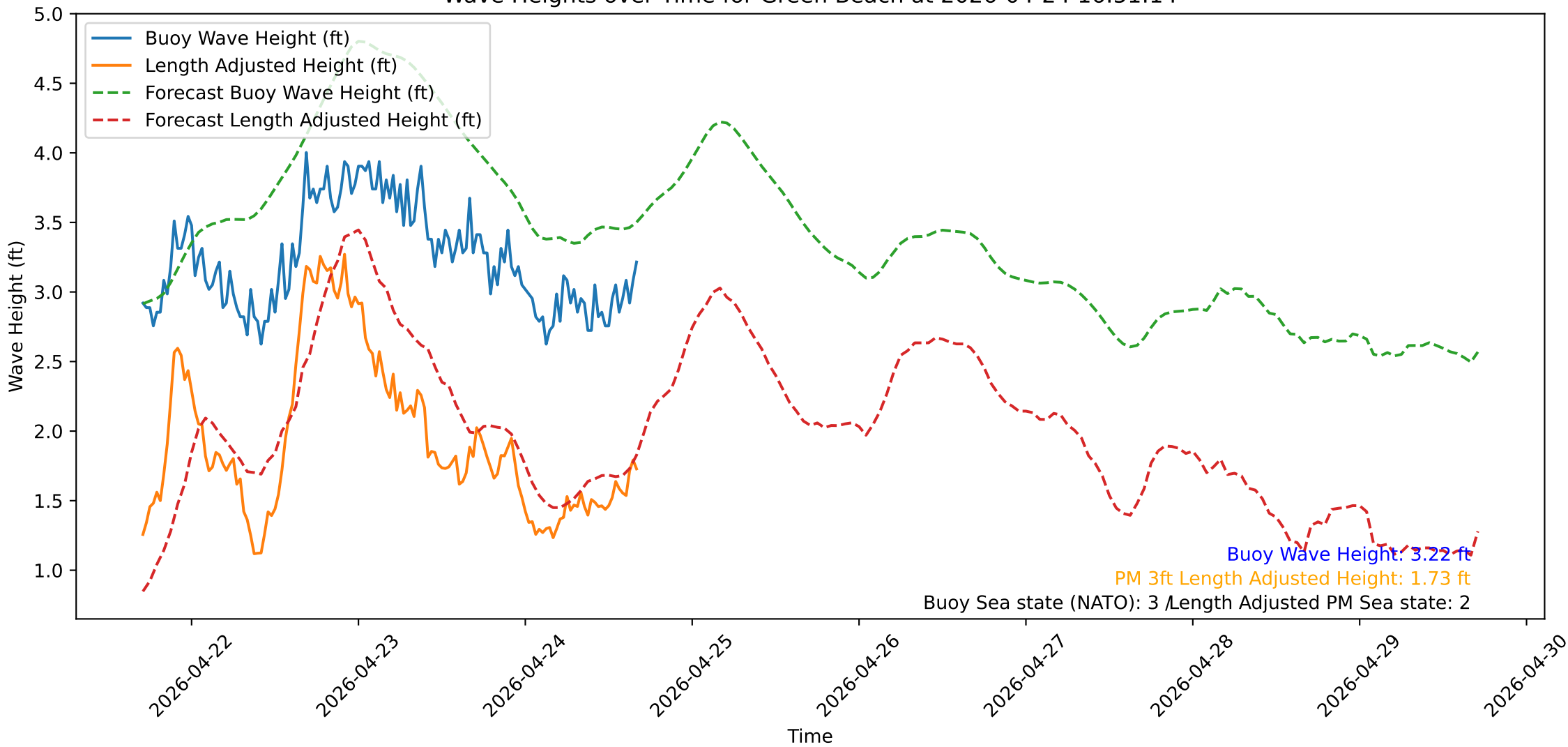
Wave Heights over Time for Green Beach at 2026-04-24 16:51:14
