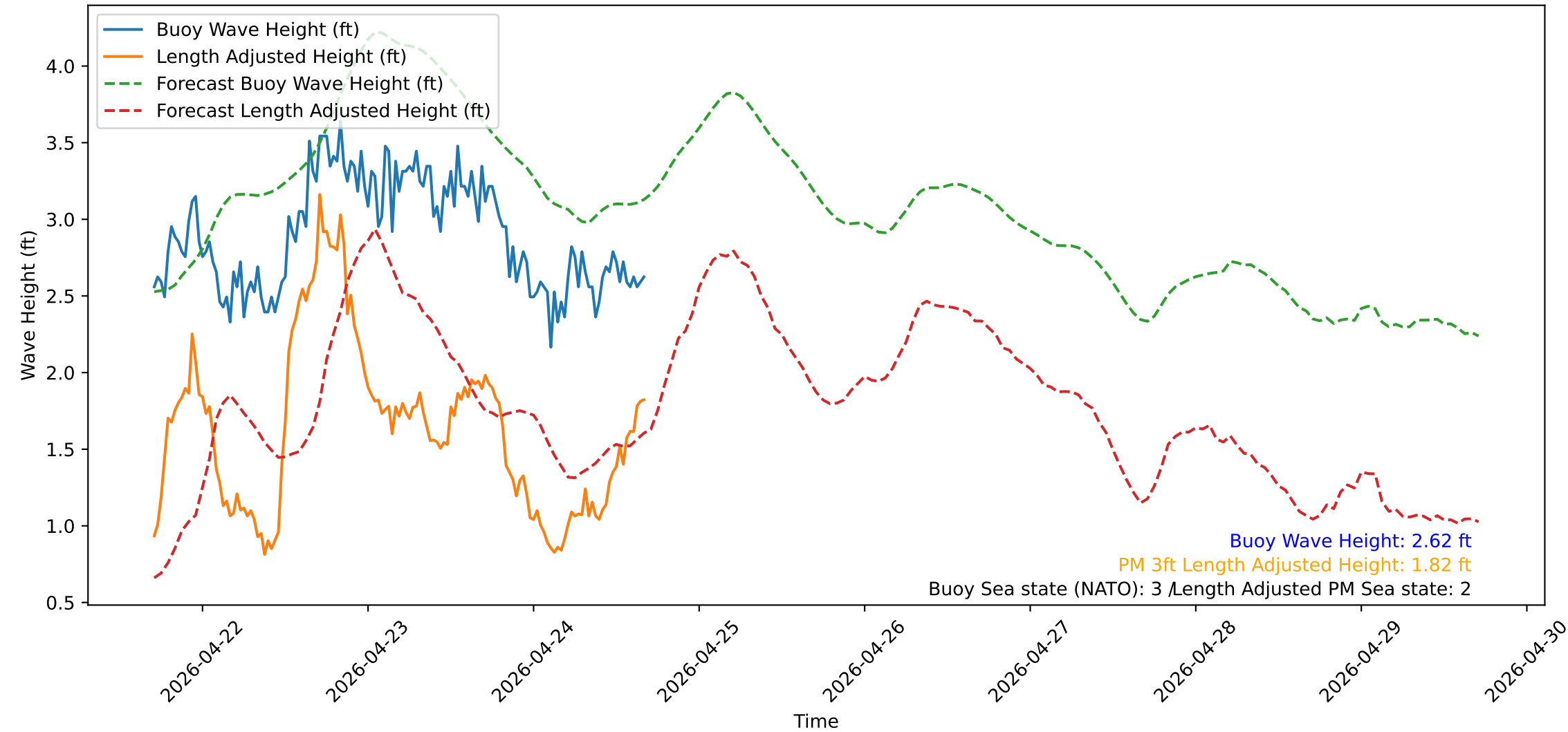
Wave Heights over Time for Red Beach at 2026-04-24 16:50:52
