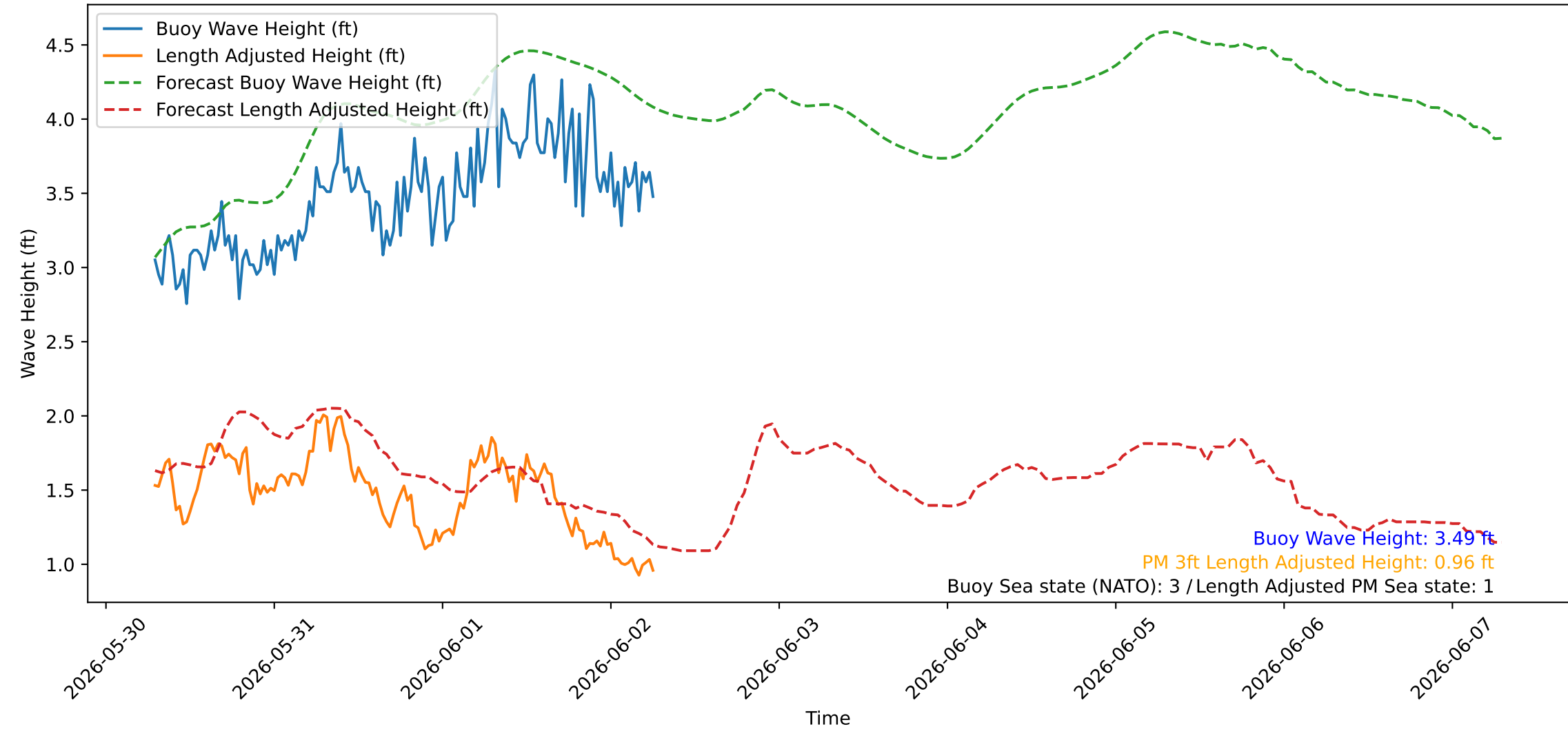
Wave Heights over Time for Green Beach at 2026-06-02 07:01:08
