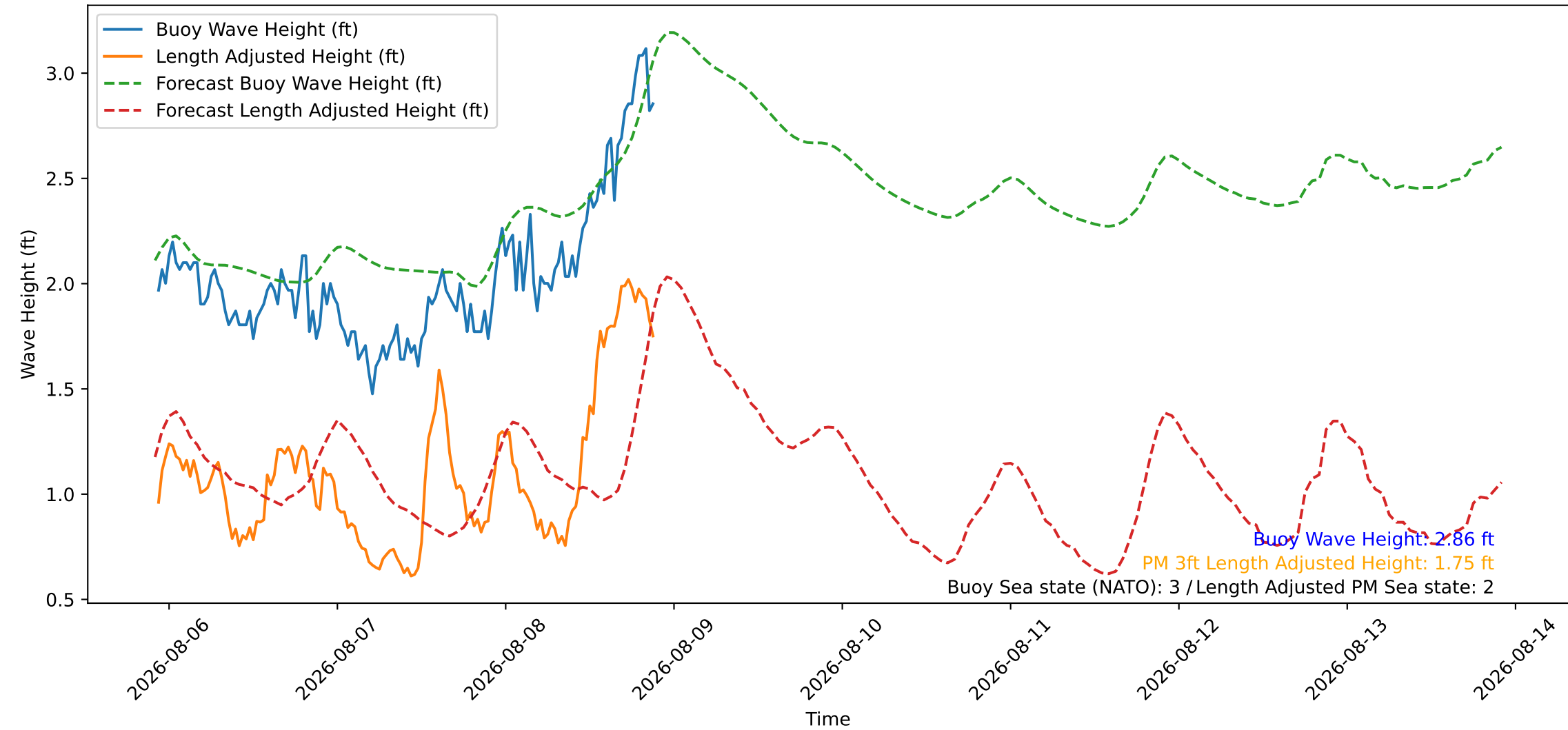
Wave Heights over Time for Red Beach at 2026-08-08 22:00:46
