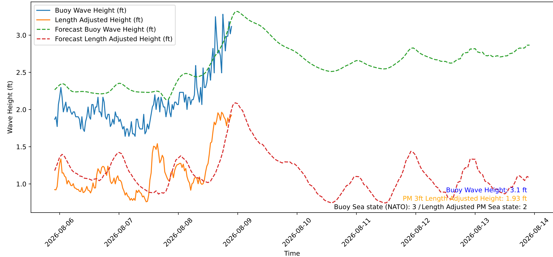
Wave Heights over Time for Oceanside Harbor at 2026-08-08 22:00:26
