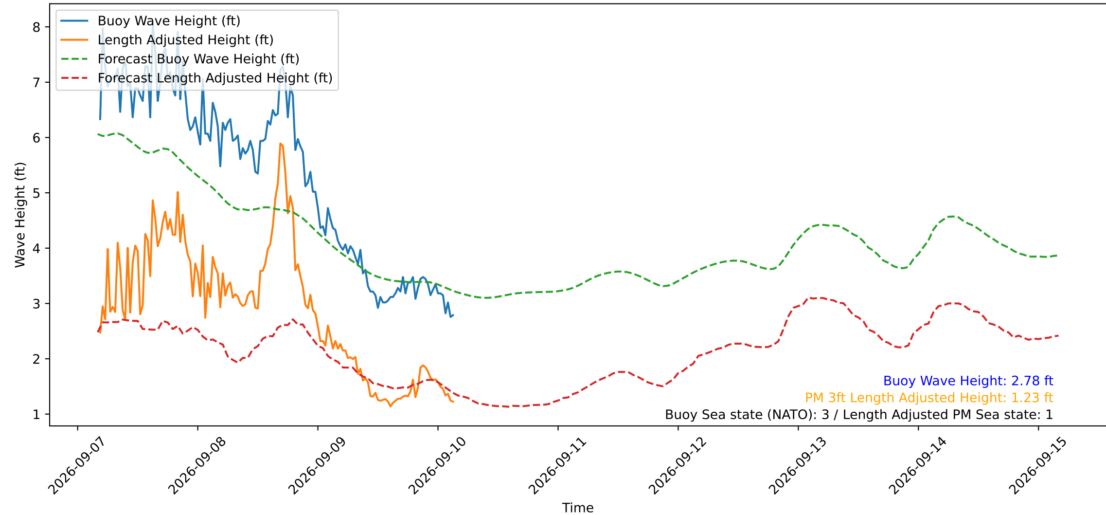
Wave Heights over Time for Green Beach at 2026-09-10 04:01:11
