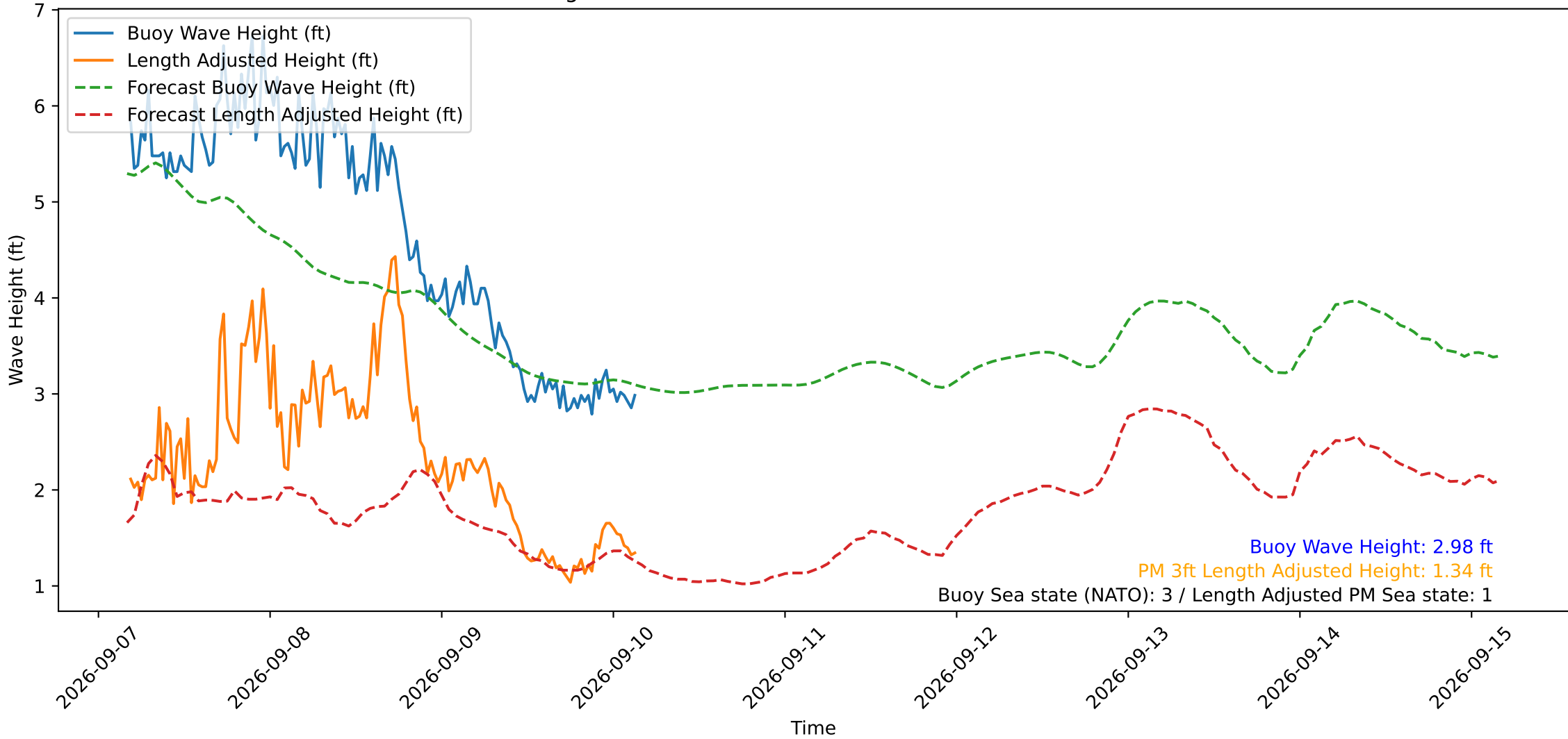
Wave Heights over Time for Red Beach at 2026-09-10 04:00:49
