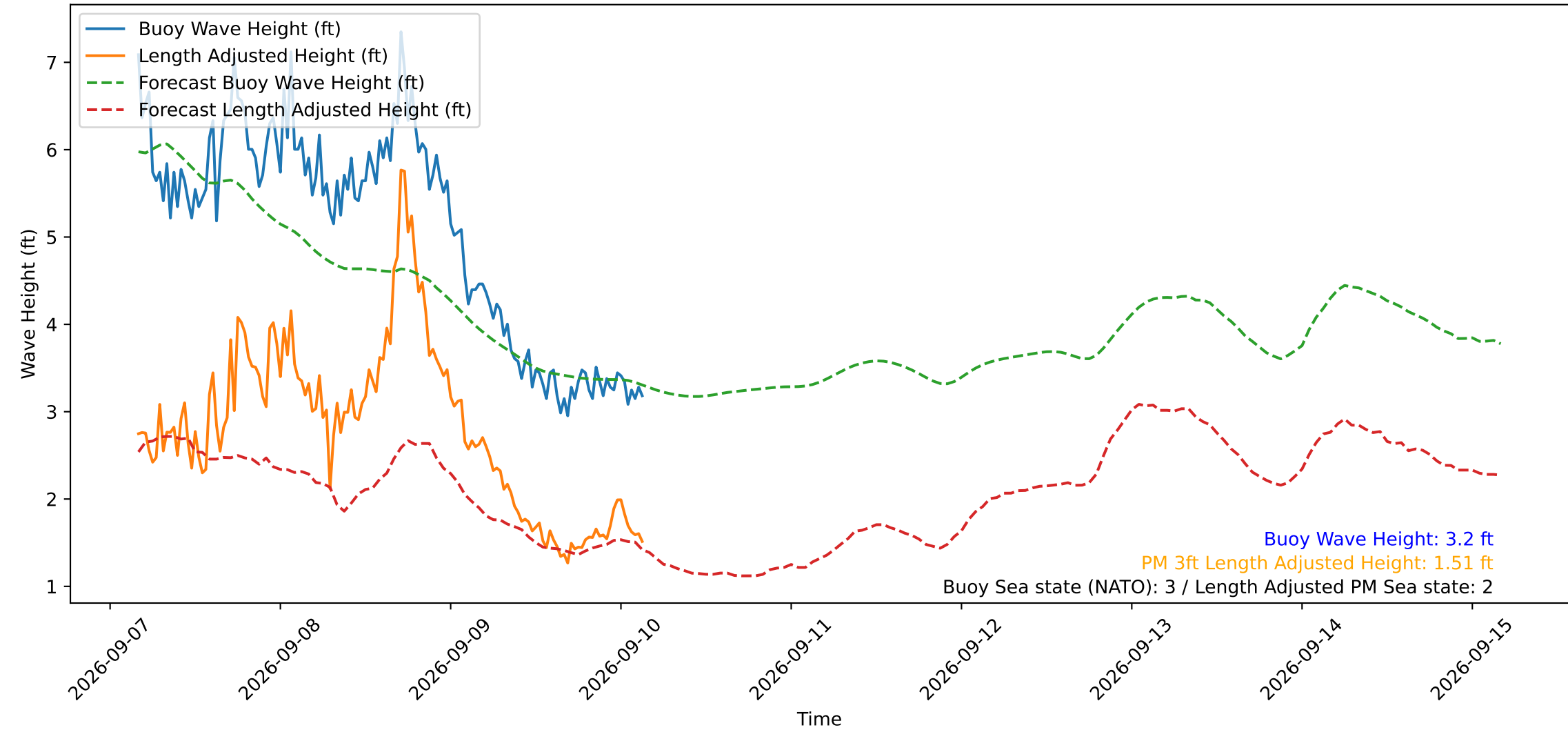
Wave Heights over Time for Oceanside Harbor at 2026-09-10 04:00:30
