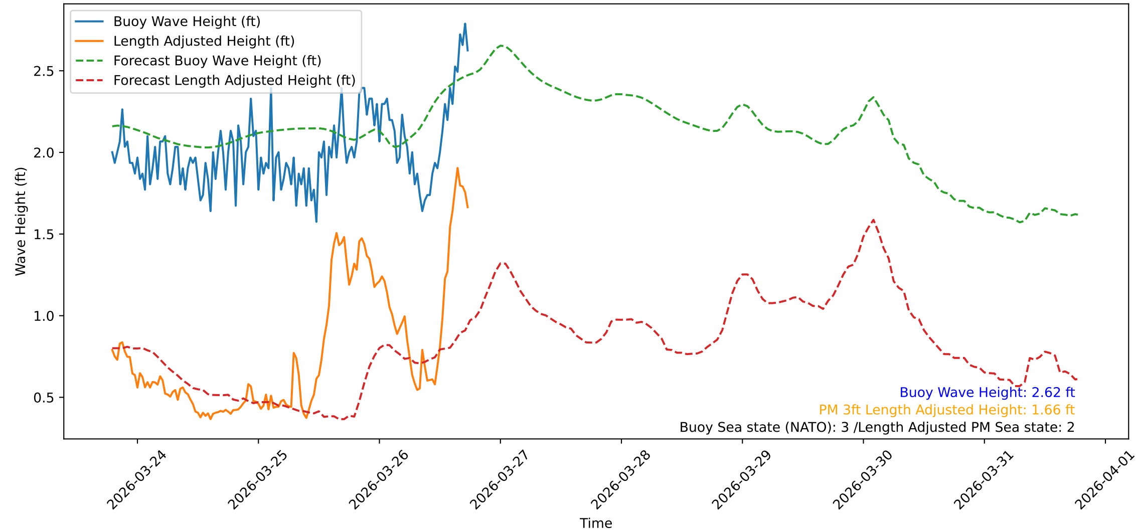
Wave Heights over Time for Red Beach at 2026-03-26 18:30:48
