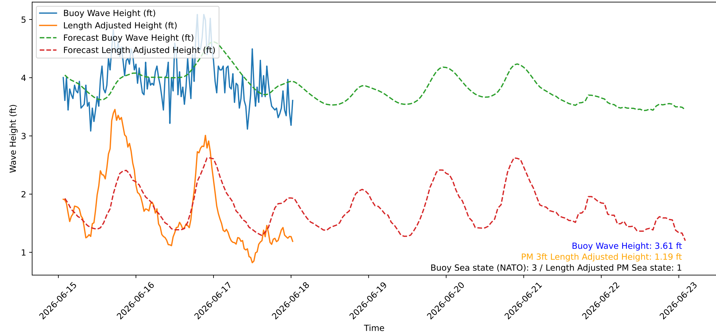
Wave Heights over Time for Green Beach at 2026-06-18 01:31:08
