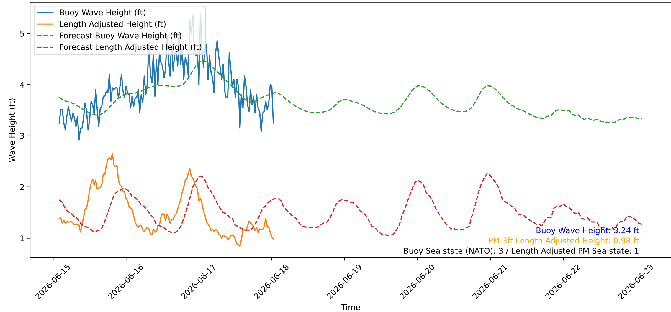
Wave Heights over Time for Red Beach at 2026-06-18 01:30:46
