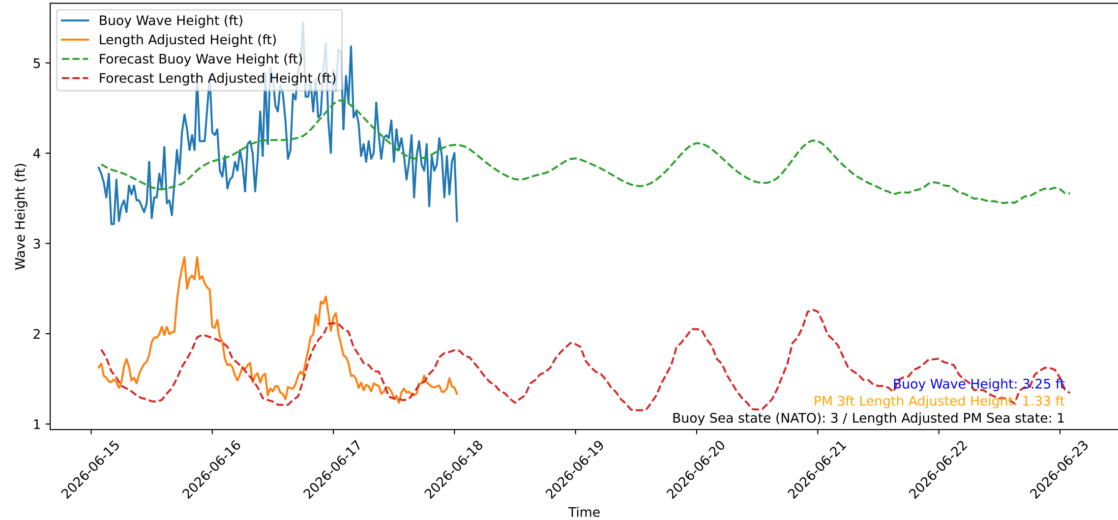
Wave Heights over Time for Oceanside Harbor at 2026-06-18 01:30:26
