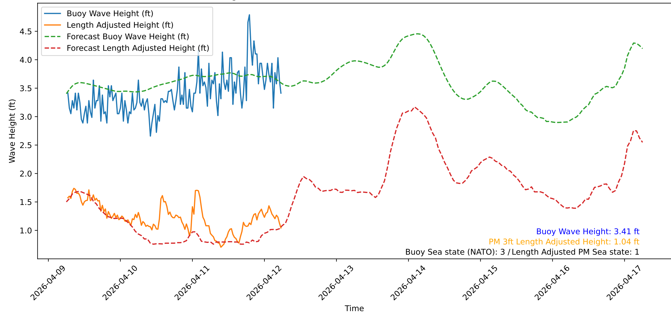
Wave Heights over Time for Oceanside Harbor at 2026-04-12 06:20:32
