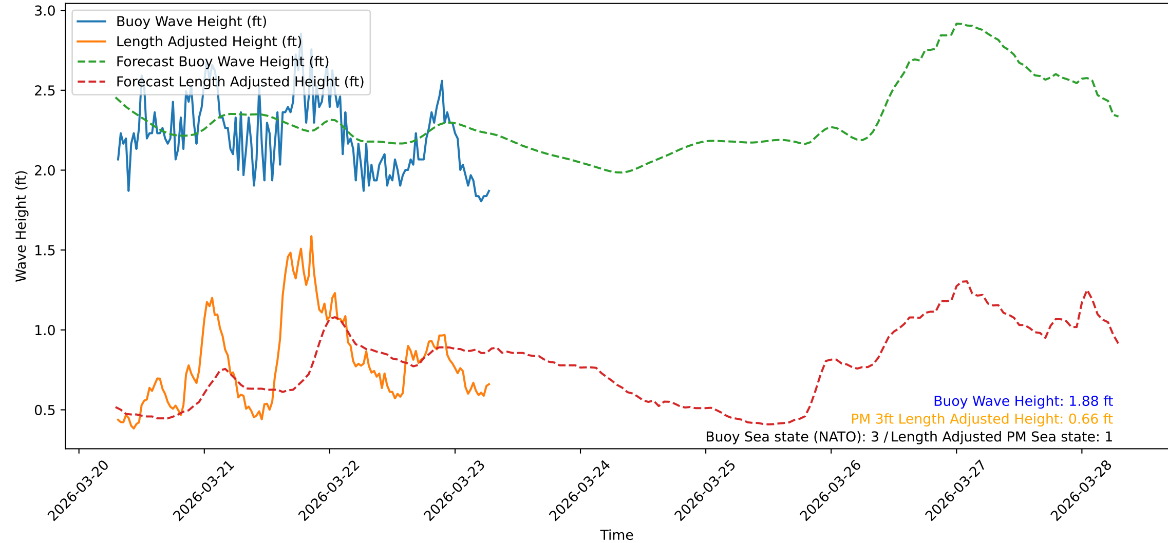
Wave Heights over Time for Red Beach at 2026-03-23 07:10:47
