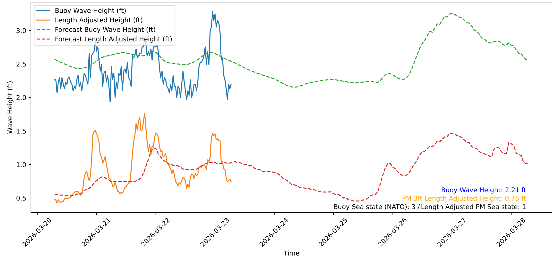
Wave Heights over Time for Green Beach at 2026-03-23 07:11:09
