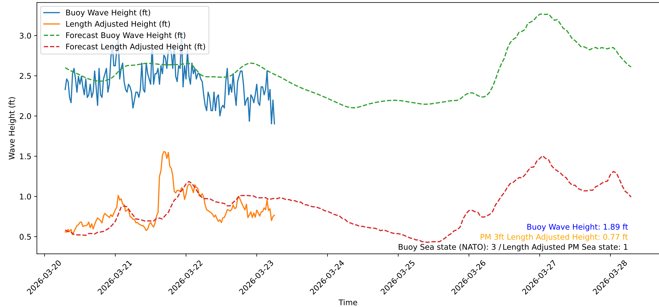
Wave Heights over Time for Oceanside Harbor at 2026-03-23 07:10:31
