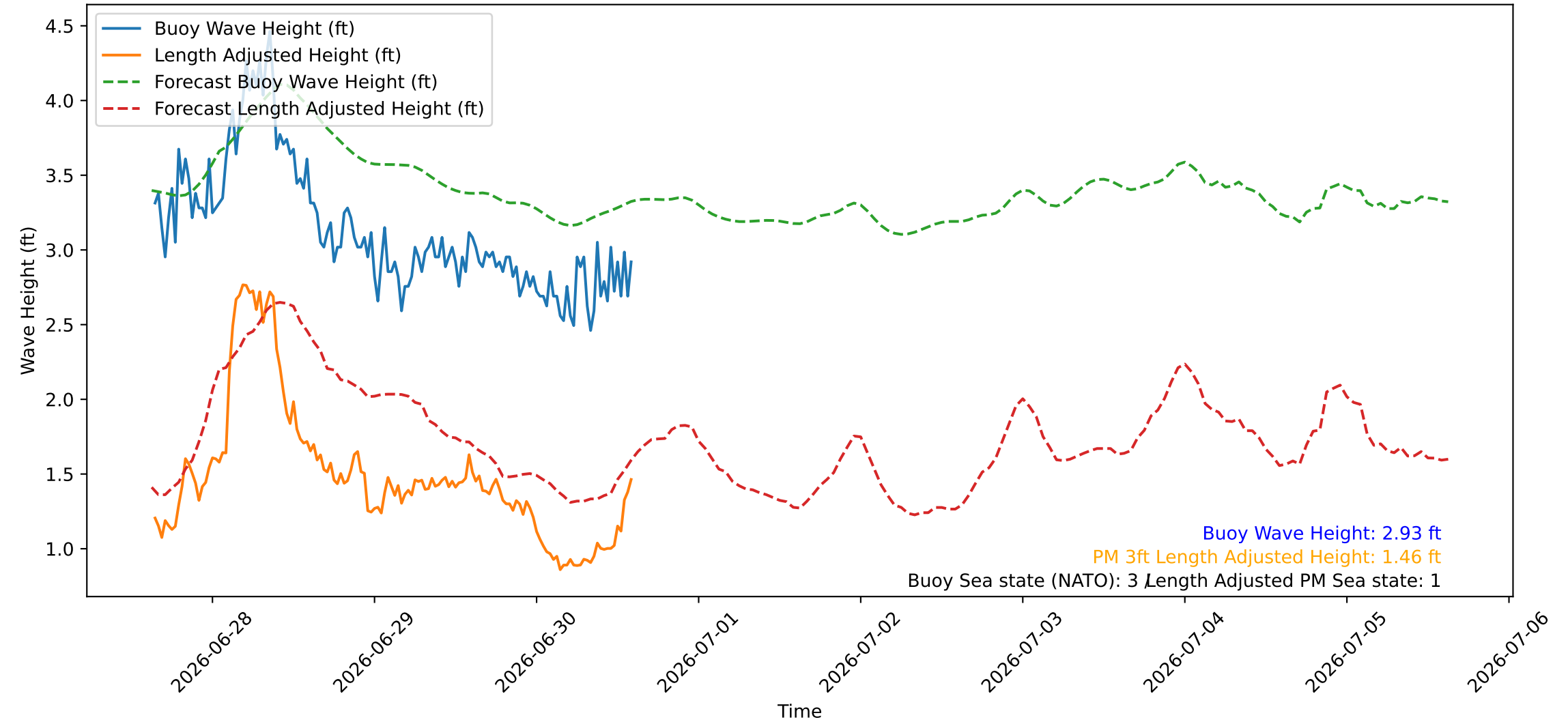
Wave Heights over Time for Red Beach at 2026-06-30 15:10:45
