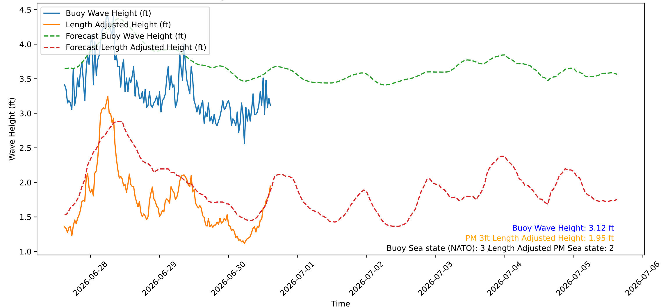
Wave Heights over Time for Oceanside Harbor at 2026-06-30 15:10:26
