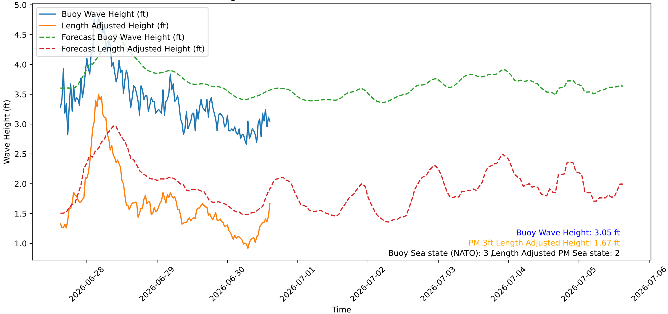
Wave Heights over Time for Green Beach at 2026-06-30 15:11:07
