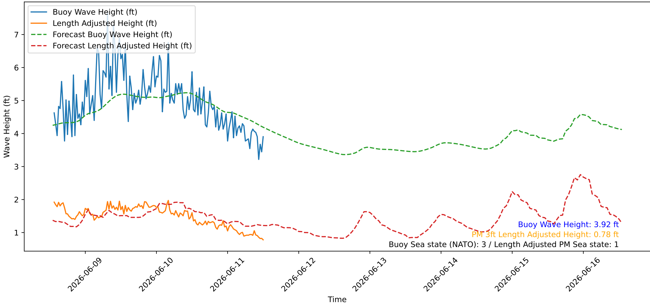
Wave Heights over Time for Red Beach at 2026-06-11 13:00:45
