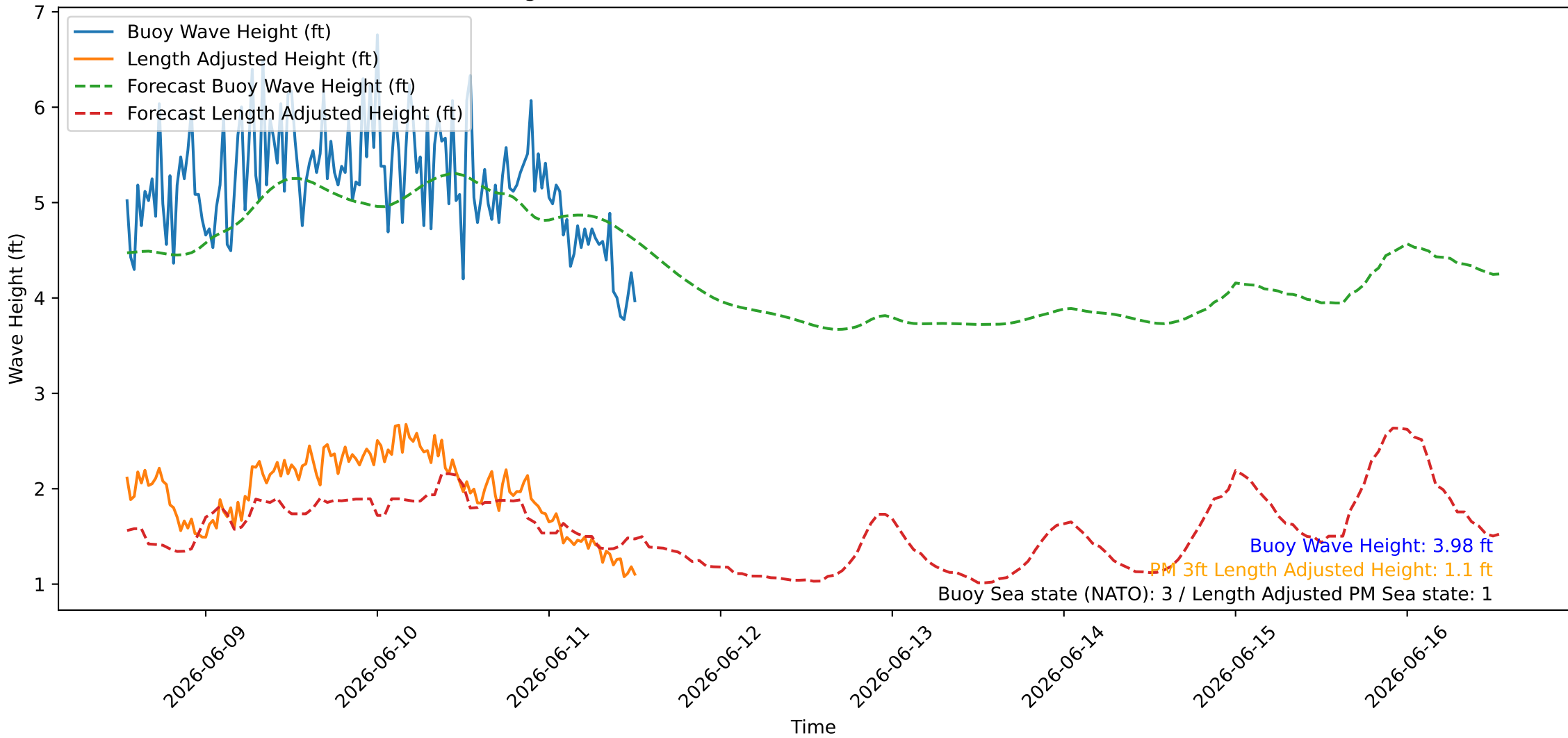
Wave Heights over Time for Oceanside Harbor at 2026-06-11 13:00:26
