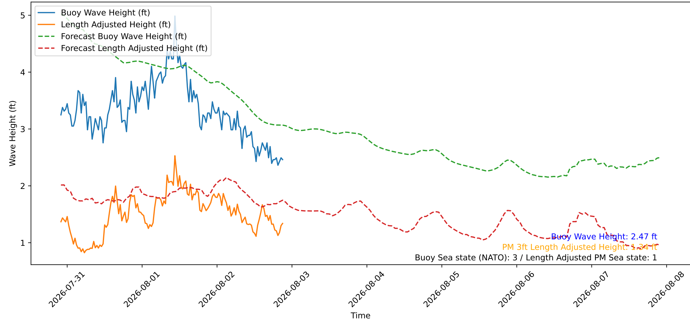
Wave Heights over Time for Green Beach at 2026-08-02 22:01:07
