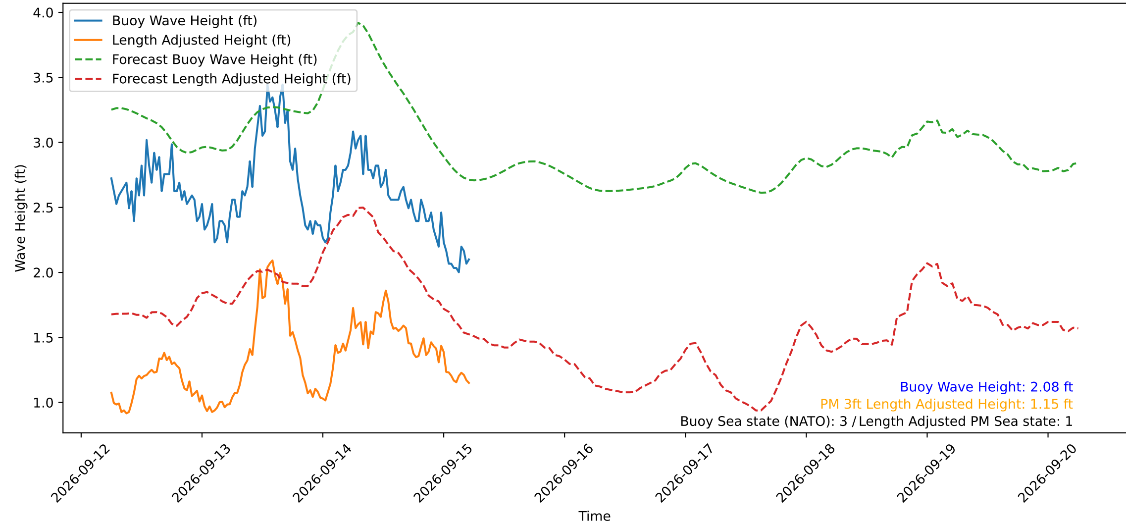
Wave Heights over Time for Red Beach at 2026-09-15 05:40:49
