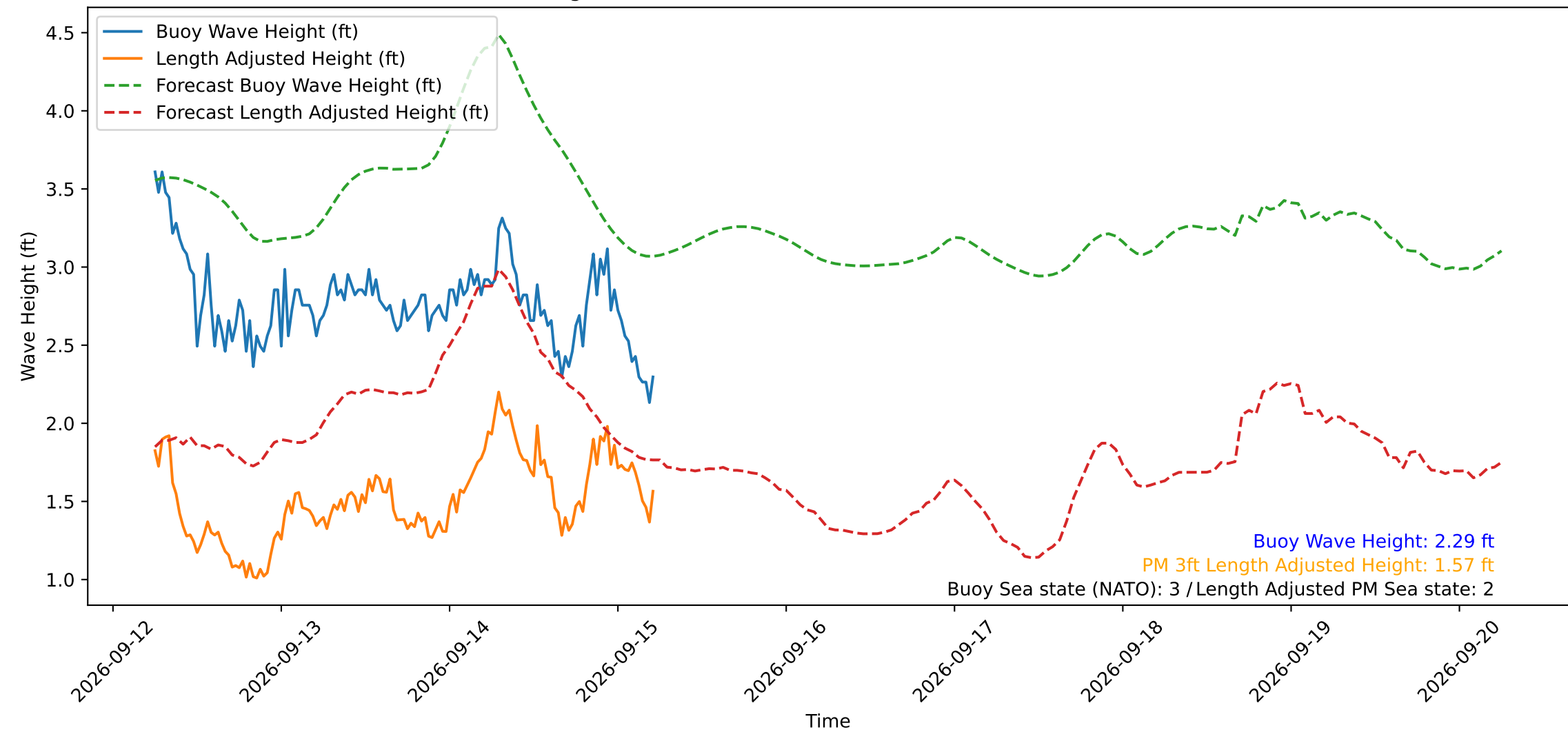
Wave Heights over Time for Green Beach at 2026-09-15 05:41:12
