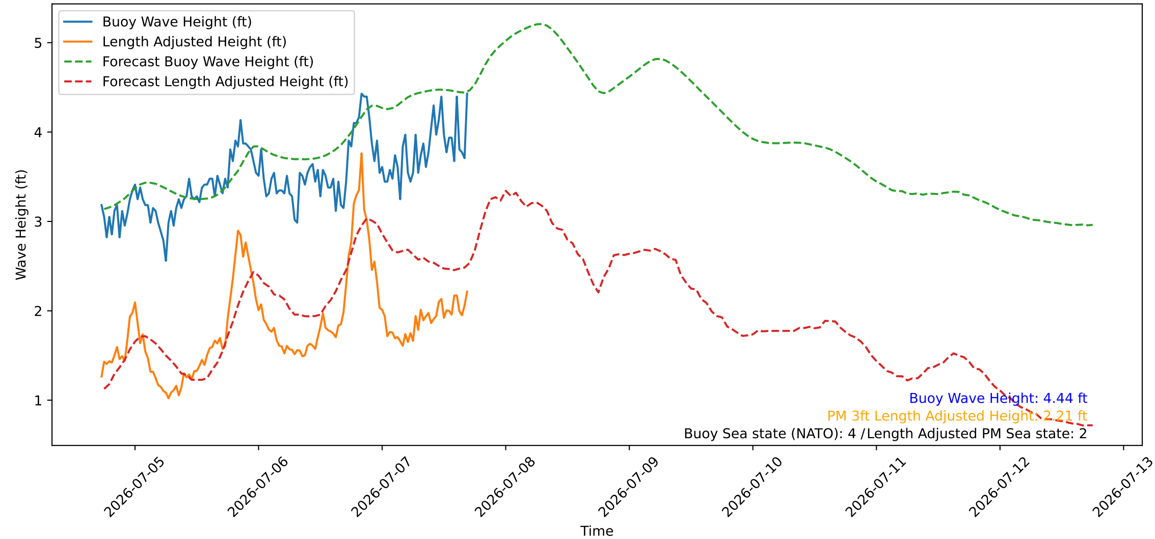
Wave Heights over Time for Green Beach at 2026-07-07 17:31:08
