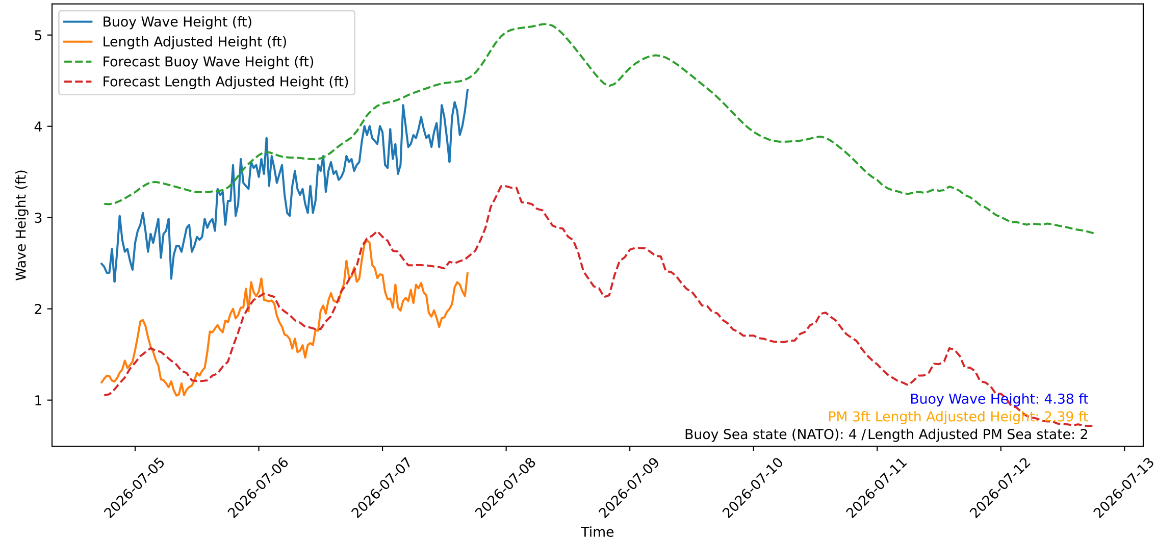
Wave Heights over Time for Oceanside Harbor at 2026-07-07 17:30:26
