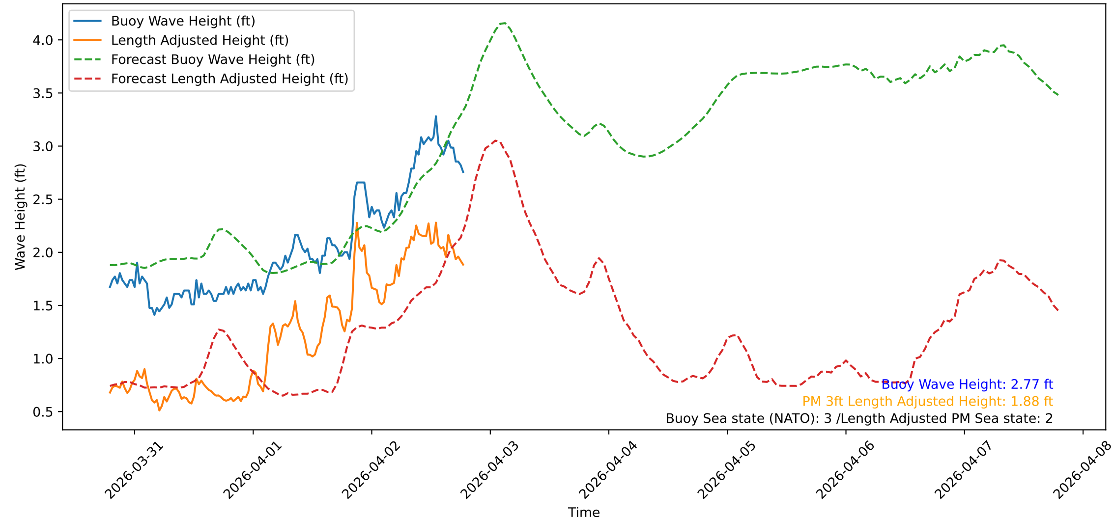
Wave Heights over Time for Green Beach at 2026-04-02 19:11:09
