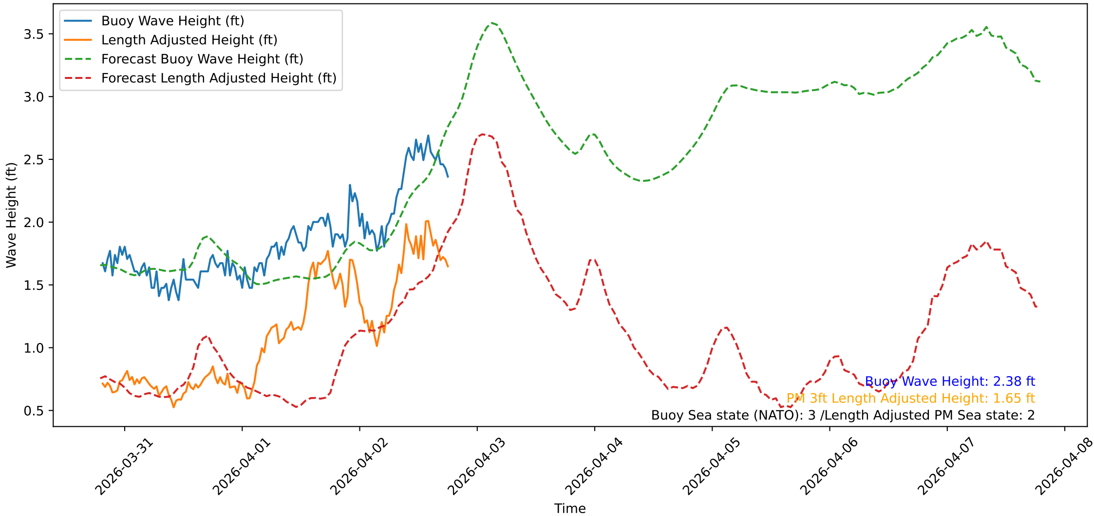
Wave Heights over Time for Red Beach at 2026-04-02 19:10:46
