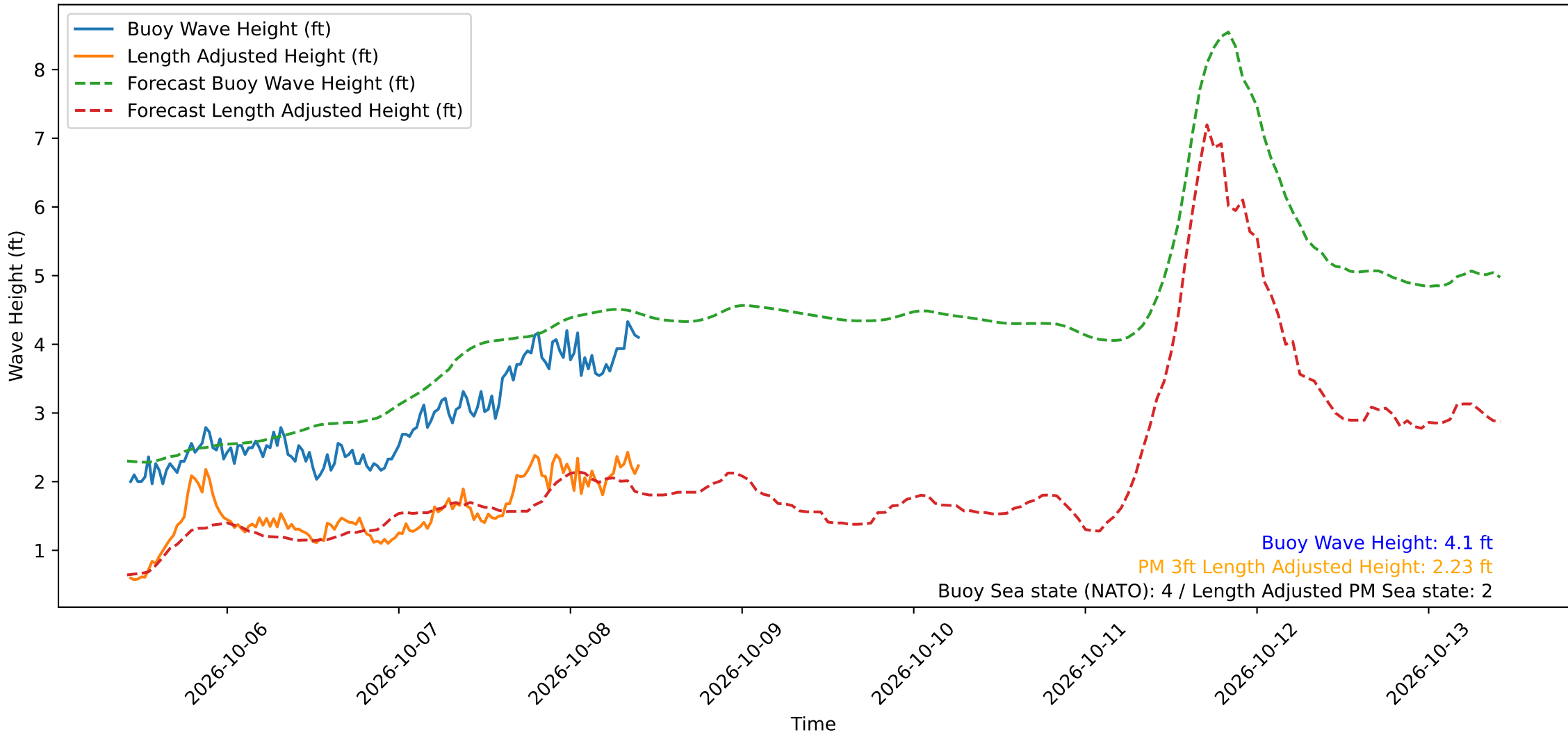
Wave Heights over Time for Oceanside Harbor at 2026-10-08 10:20:29
