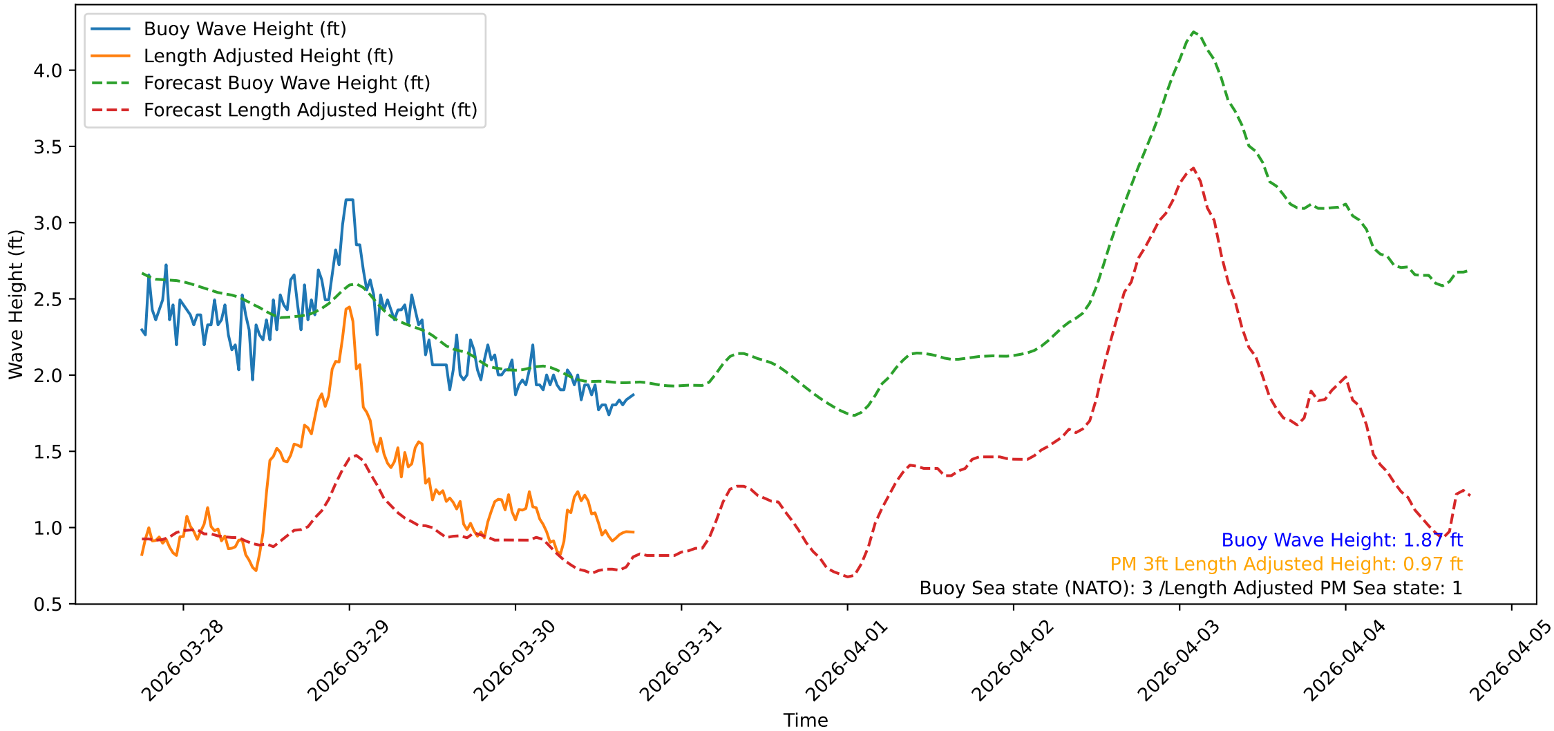
Wave Heights over Time for Oceanside Harbor at 2026-03-30 17:50:31
