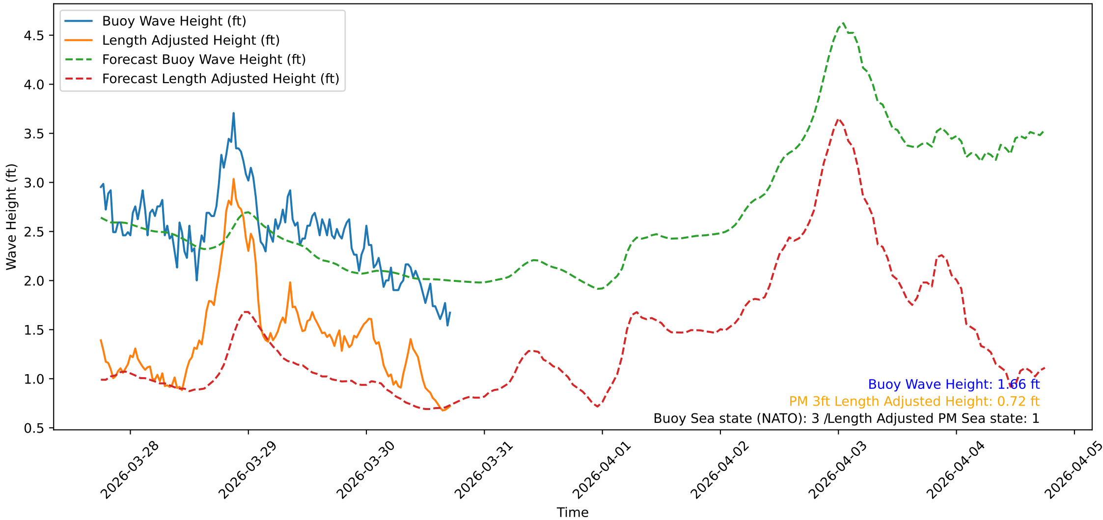
Wave Heights over Time for Green Beach at 2026-03-30 17:51:09
