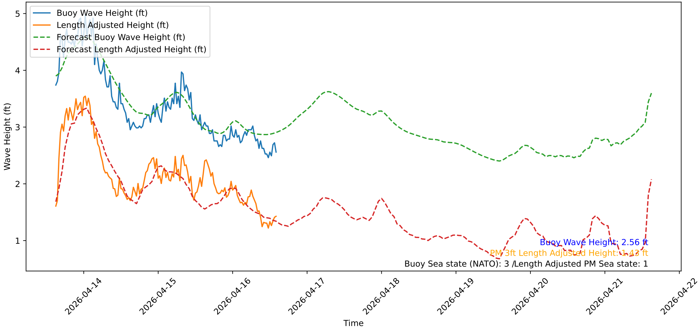
Wave Heights over Time for Green Beach at 2026-04-16 15:01:13
