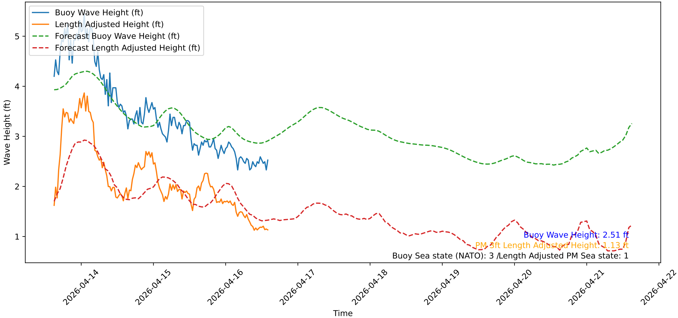
Wave Heights over Time for Oceanside Harbor at 2026-04-16 15:00:31
