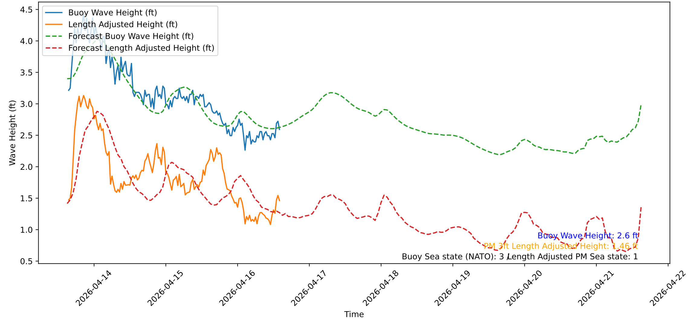
Wave Heights over Time for Red Beach at 2026-04-16 15:00:50
