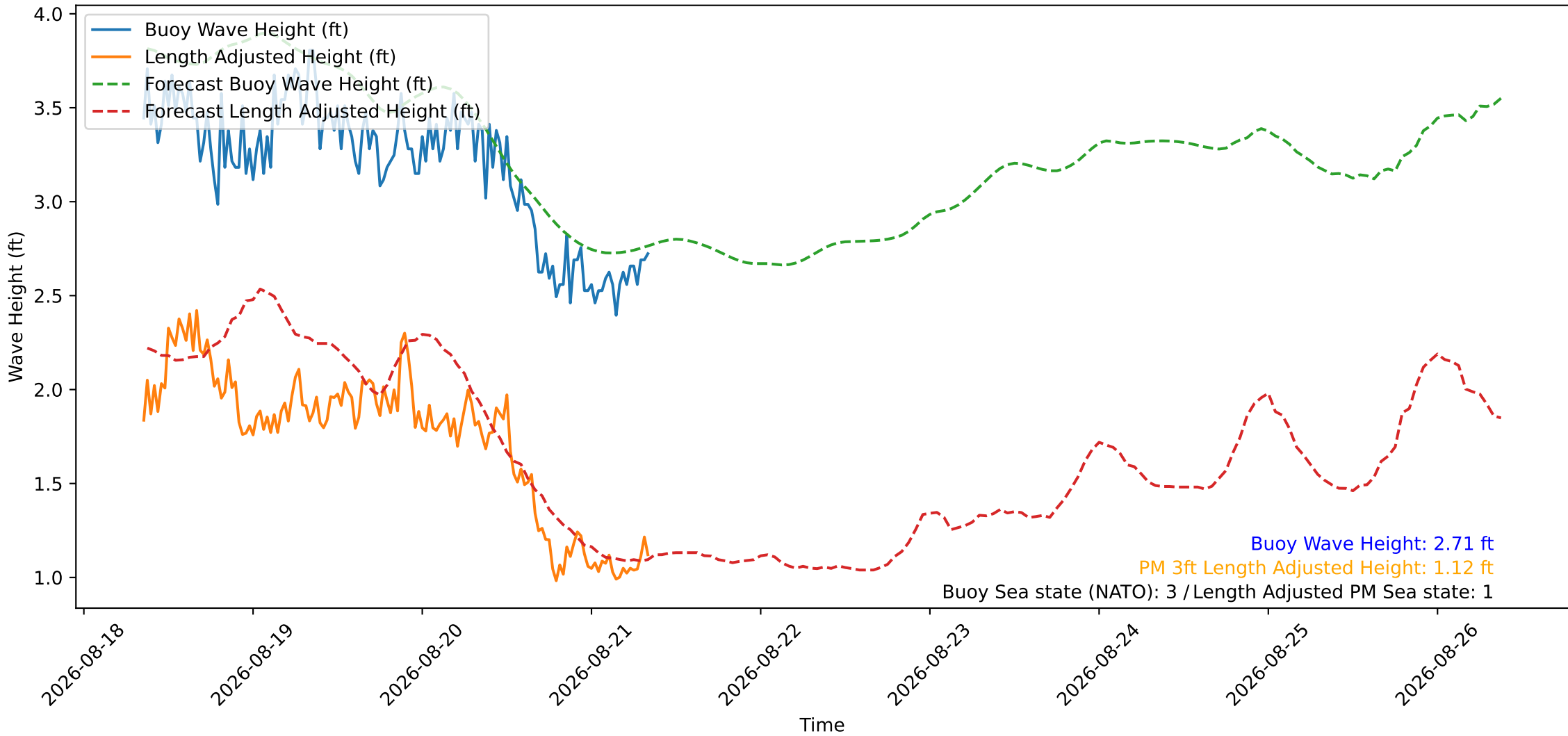
Wave Heights over Time for Oceanside Harbor at 2026-08-21 08:40:27
