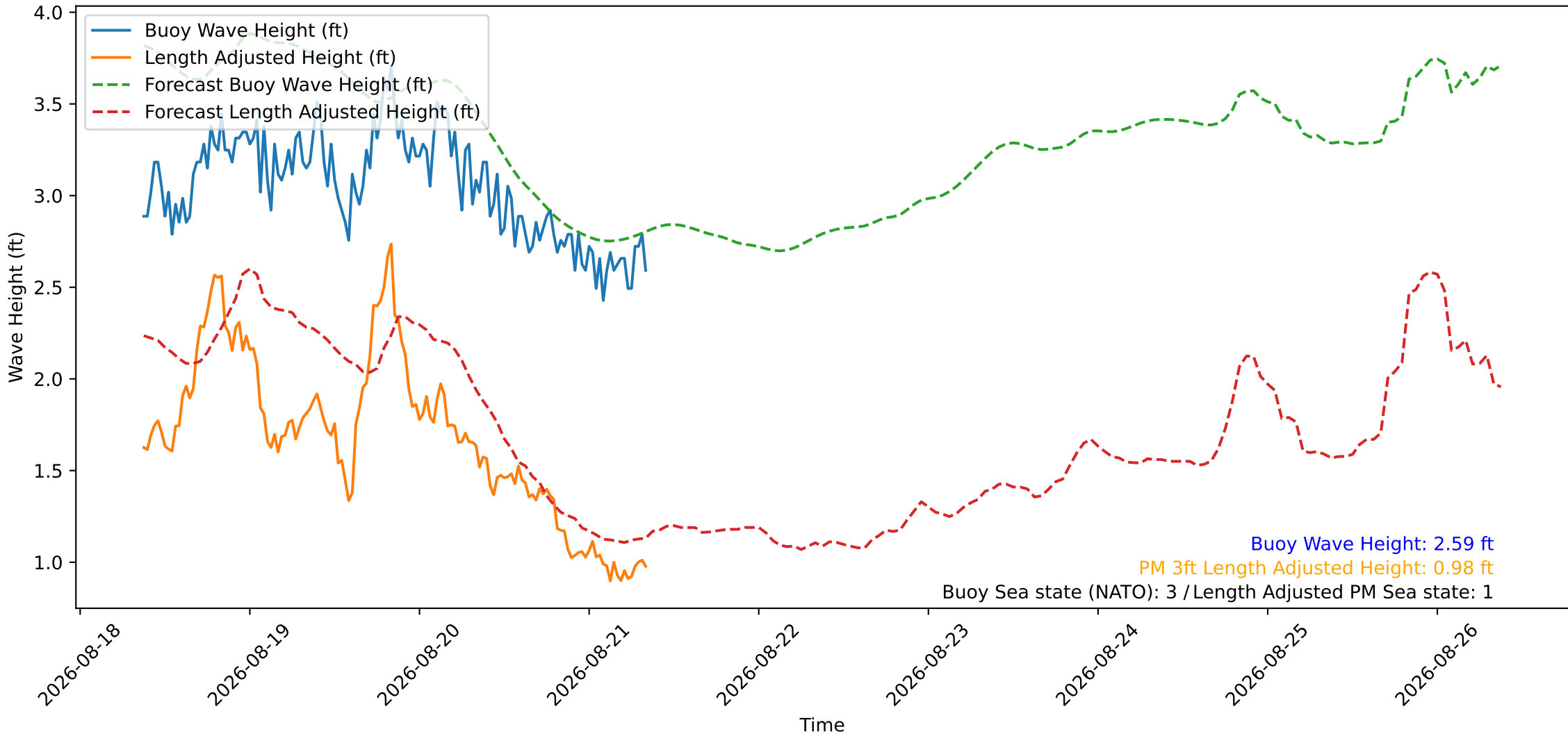
Wave Heights over Time for Green Beach at 2026-08-21 08:41:09
