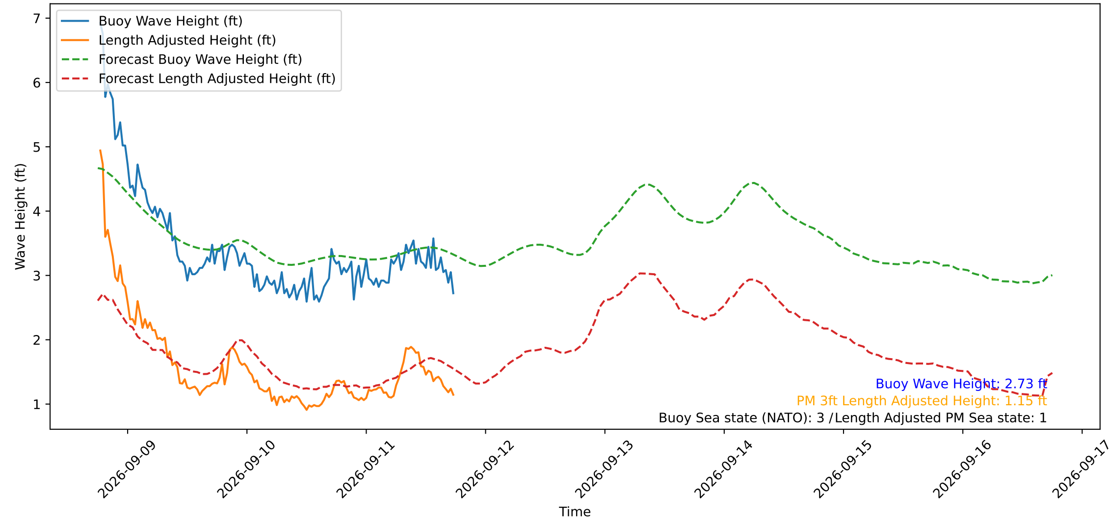
Wave Heights over Time for Green Beach at 2026-09-11 18:11:12
