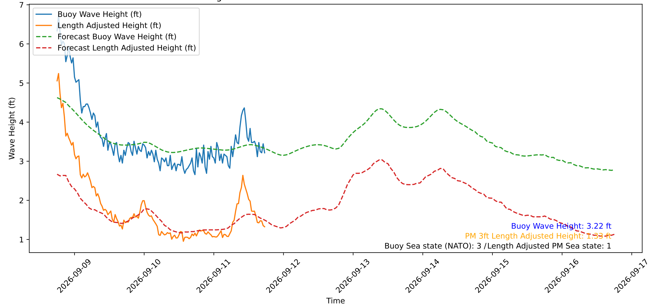
Wave Heights over Time for Oceanside Harbor at 2026-09-11 18:10:30
