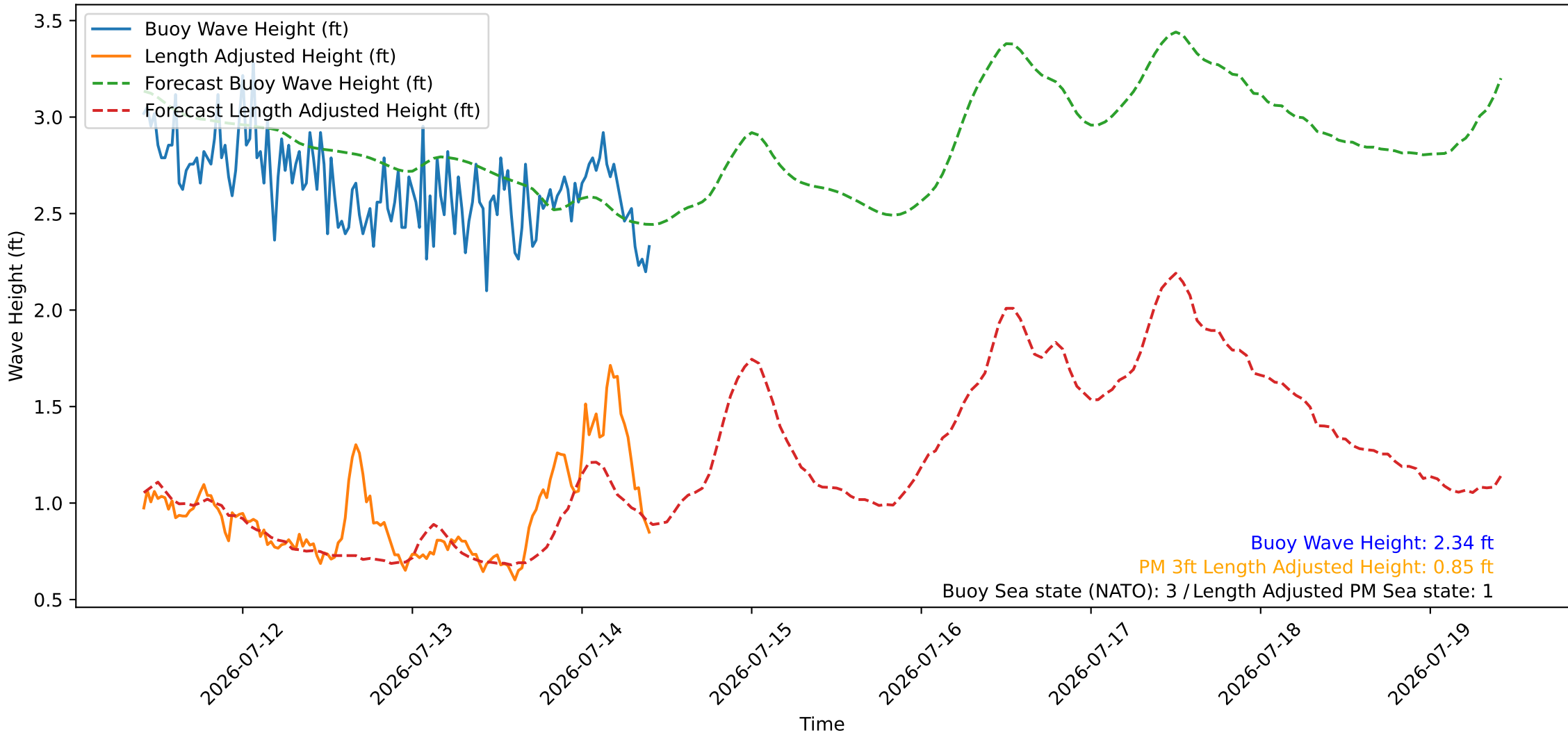
Wave Heights over Time for Oceanside Harbor at 2026-07-14 10:10:27
