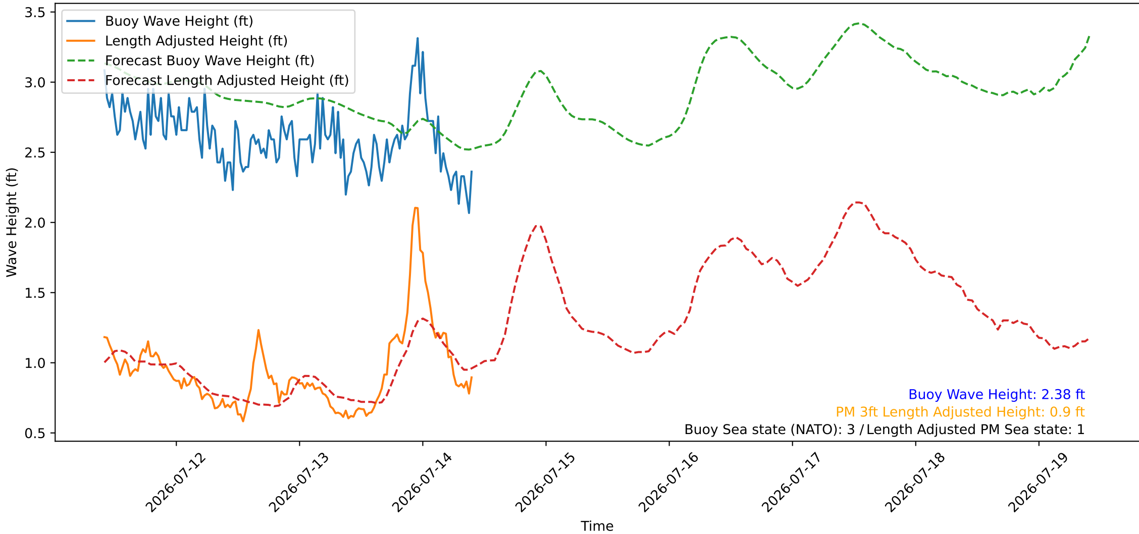
Wave Heights over Time for Green Beach at 2026-07-14 10:11:10
