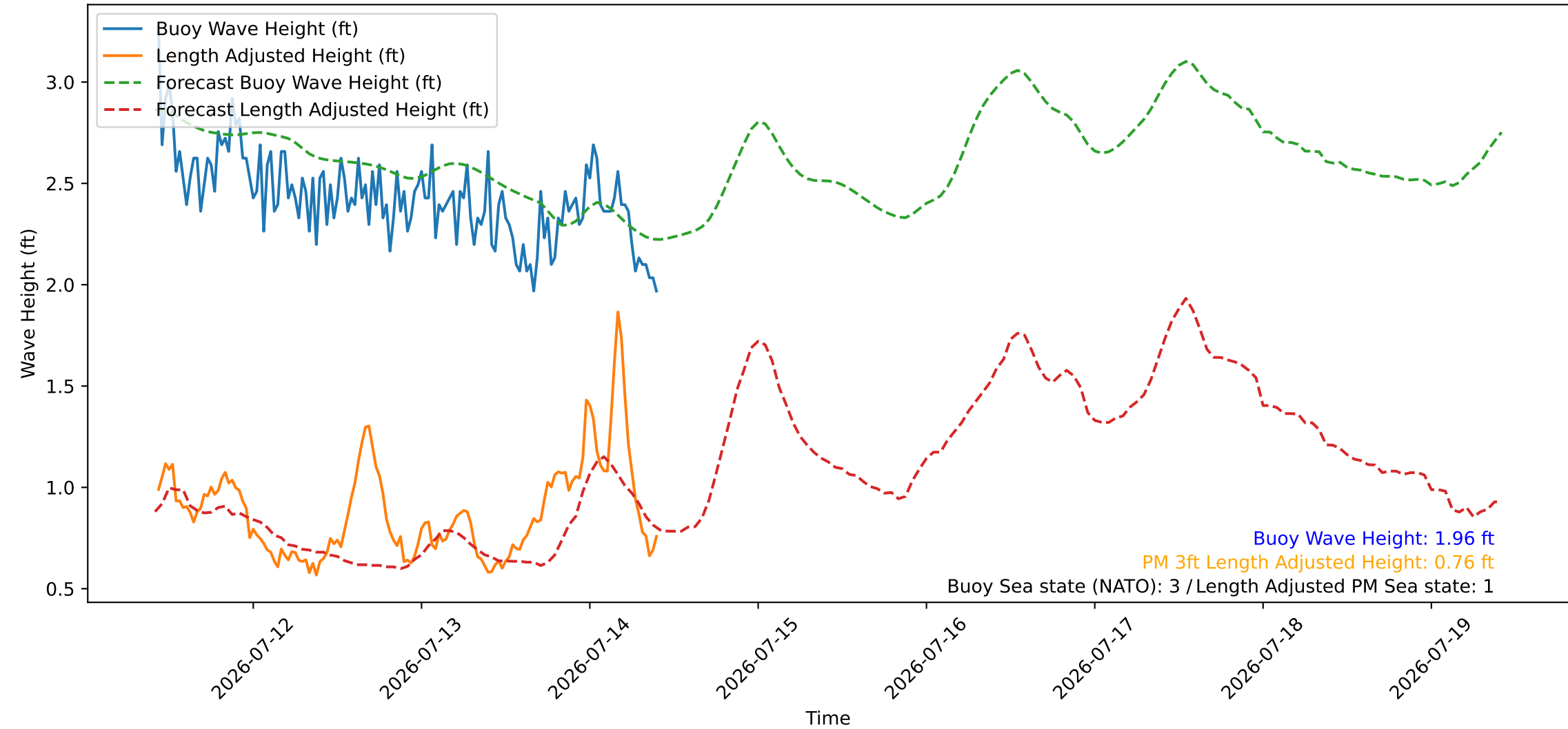
Wave Heights over Time for Red Beach at 2026-07-14 10:10:47
