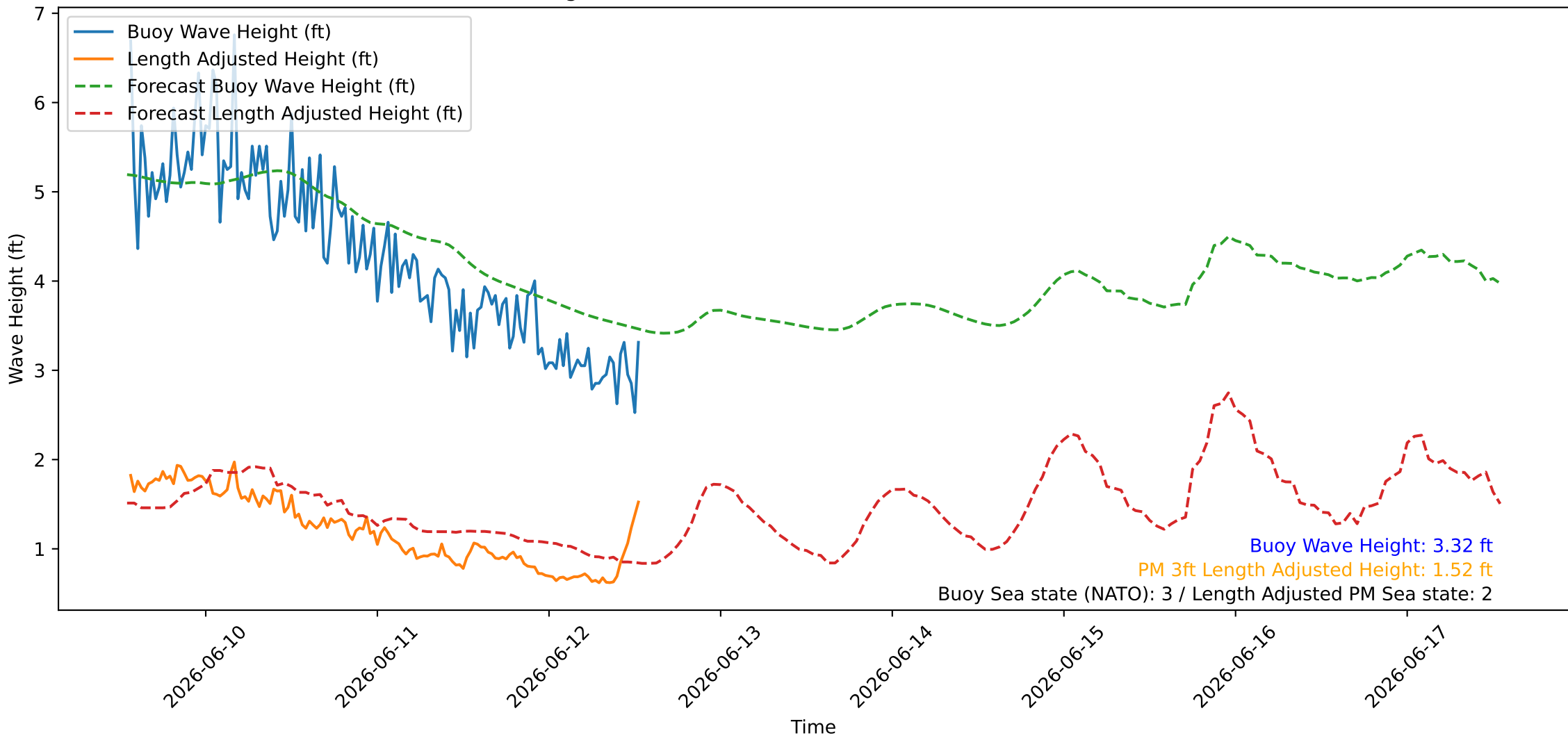
Wave Heights over Time for Red Beach at 2026-06-12 13:10:47
