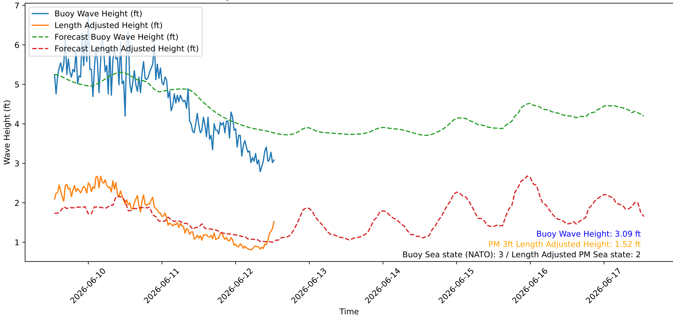
Wave Heights over Time for Oceanside Harbor at 2026-06-12 13:10:26
