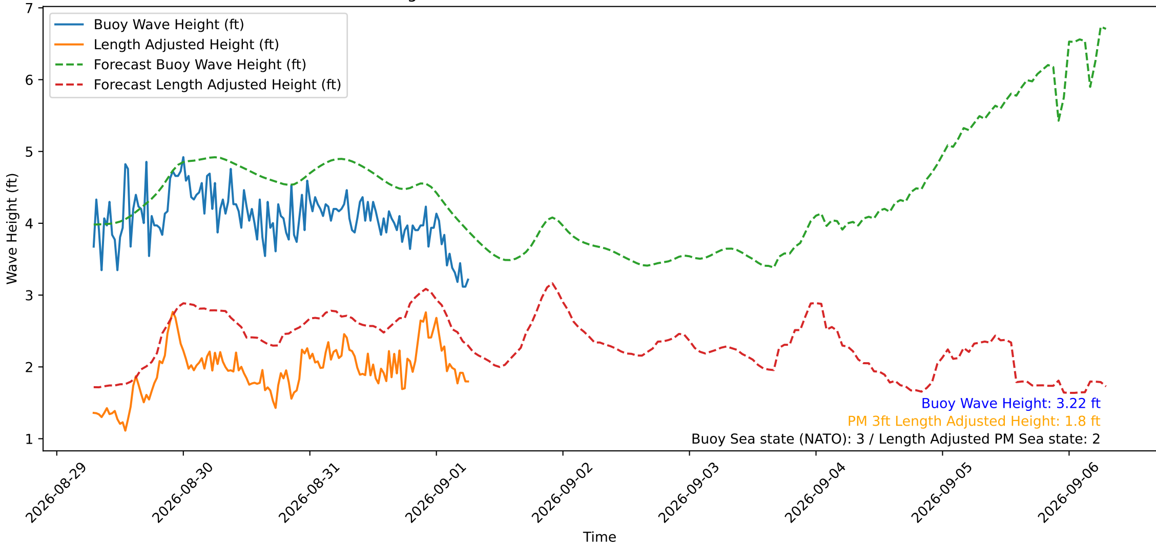
Wave Heights over Time for Green Beach at 2026-09-01 06:41:11
