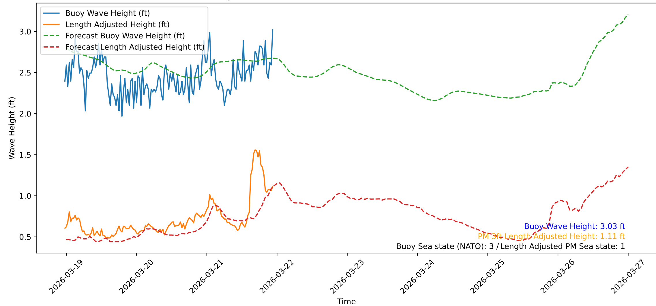
Wave Heights over Time for Oceanside Harbor at 2026-03-21 23:30:32
