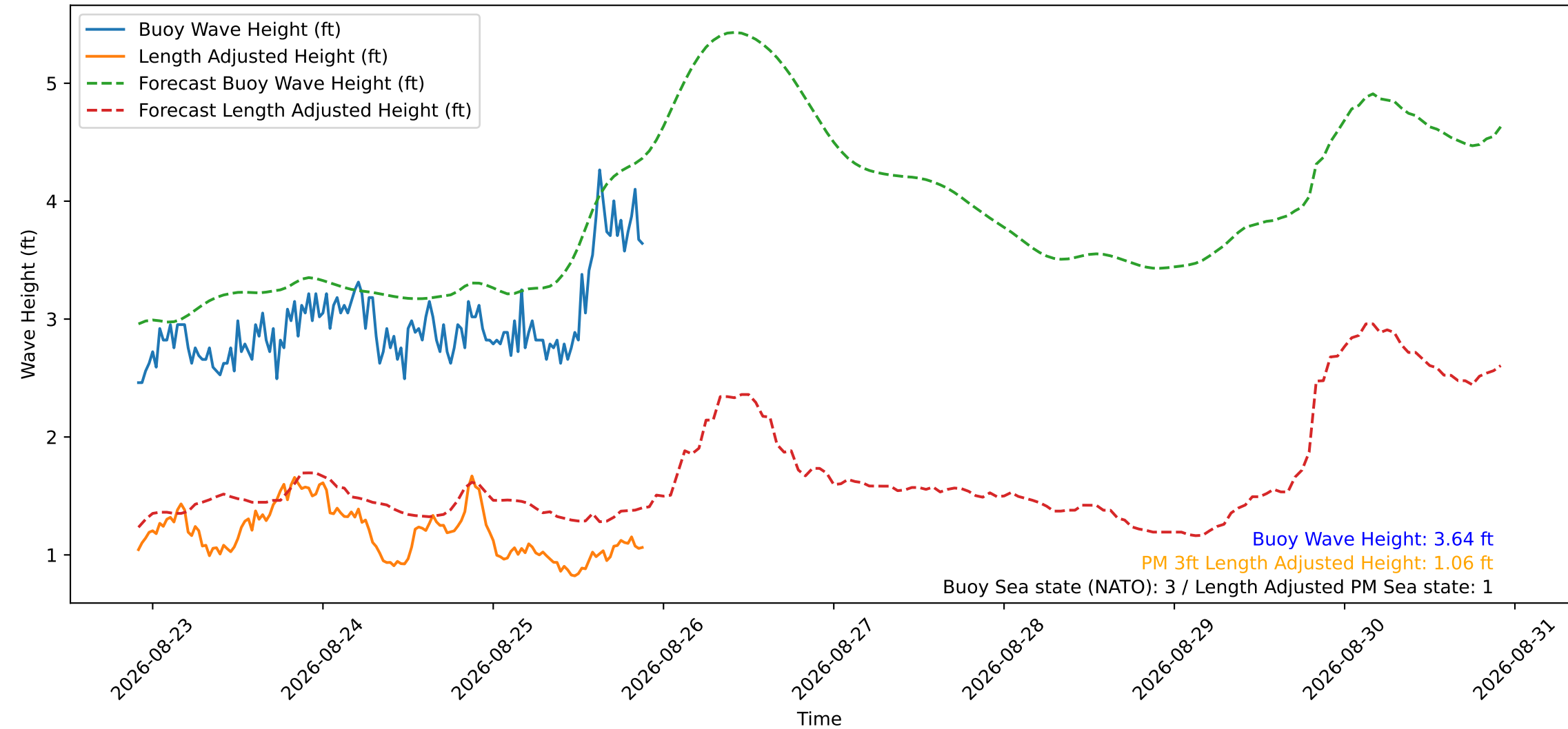
Wave Heights over Time for Green Beach at 2026-08-25 21:41:11
