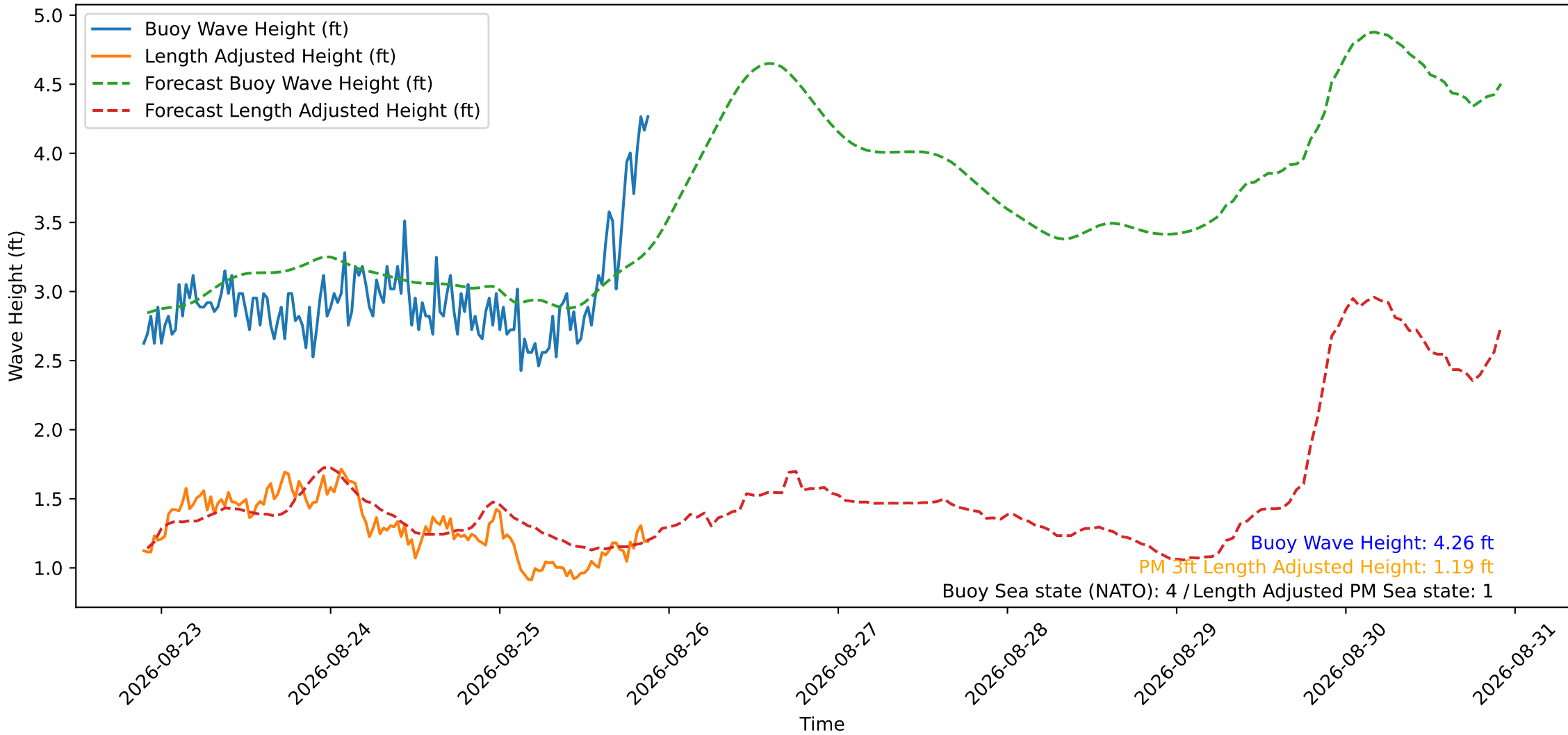
Wave Heights over Time for Oceanside Harbor at 2026-08-25 21:40:29
