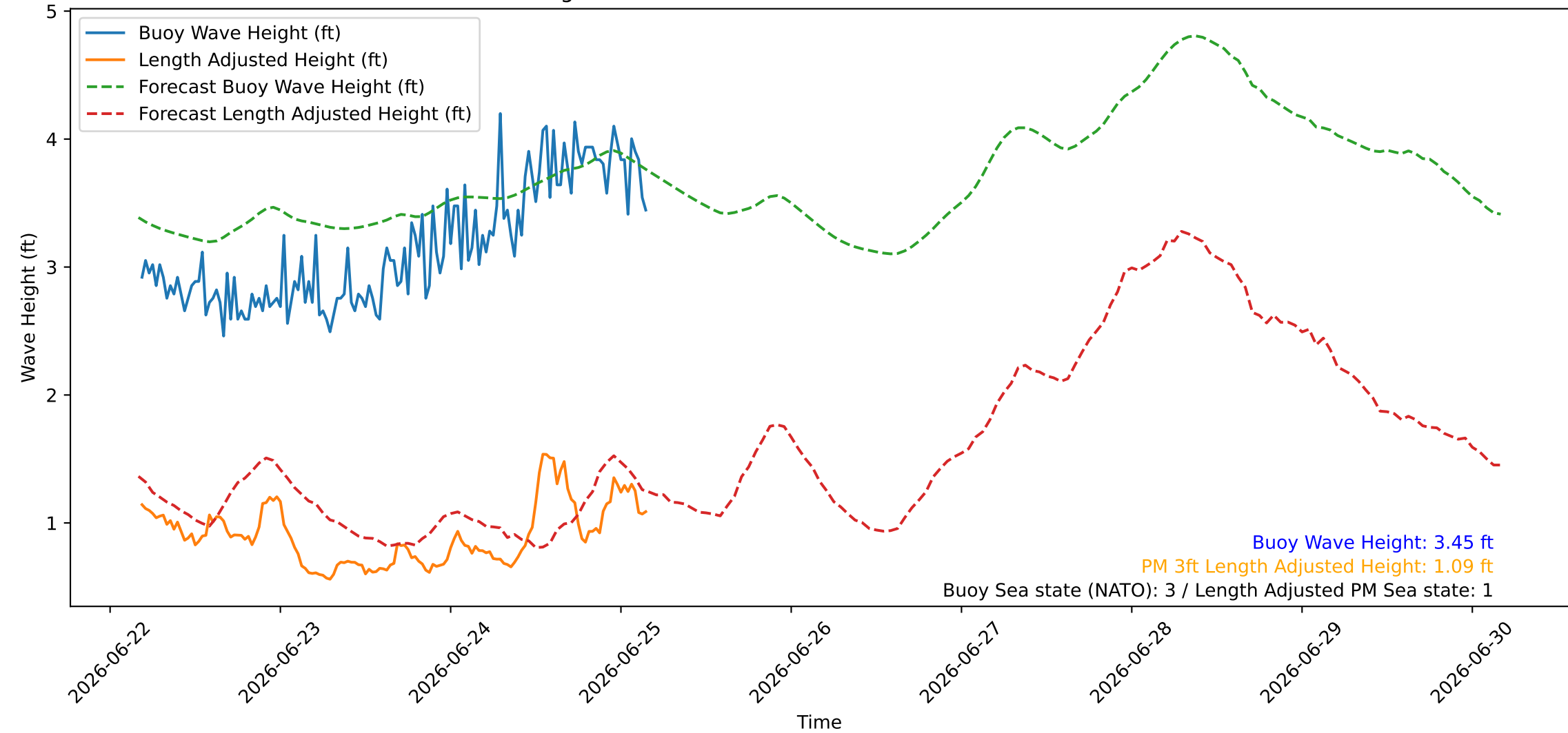
Wave Heights over Time for Green Beach at 2026-06-25 04:21:09
