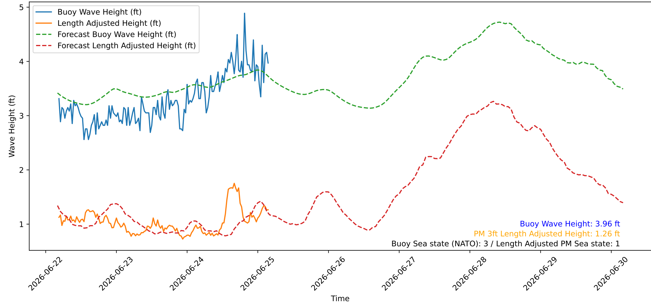
Wave Heights over Time for Oceanside Harbor at 2026-06-25 04:20:26
