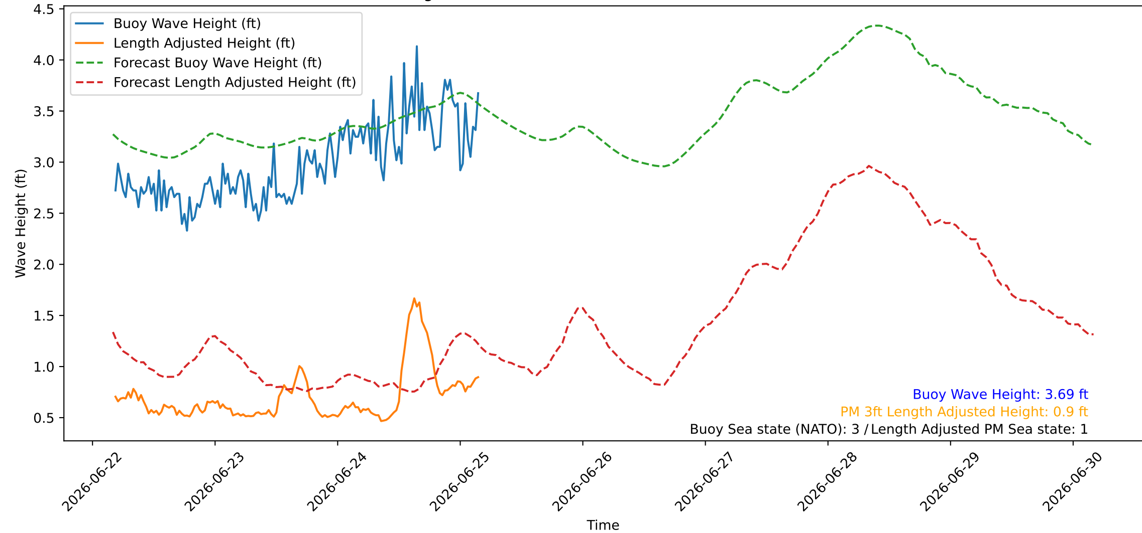
Wave Heights over Time for Red Beach at 2026-06-25 04:20:46
