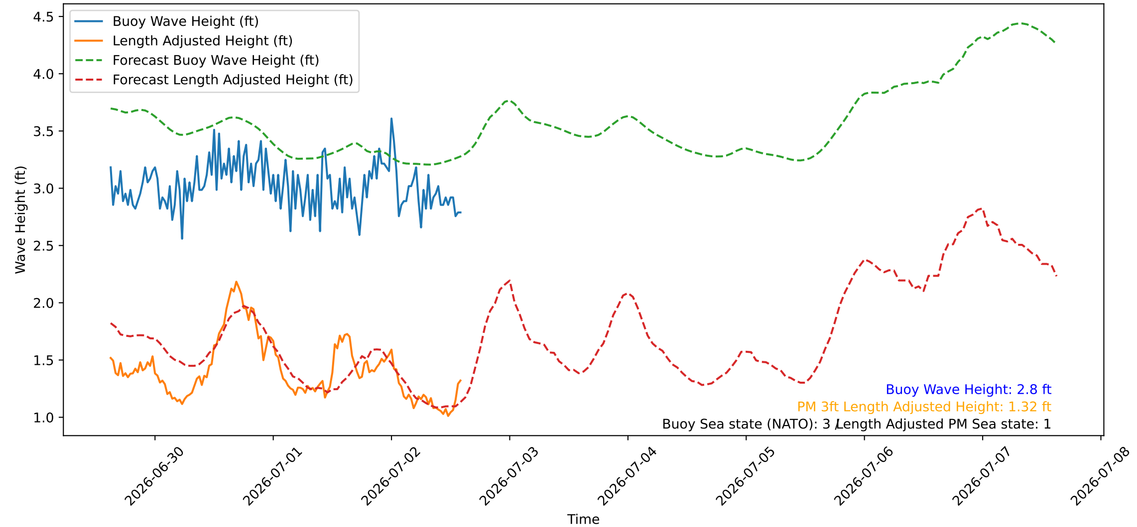
Wave Heights over Time for Oceanside Harbor at 2026-07-02 15:00:26
