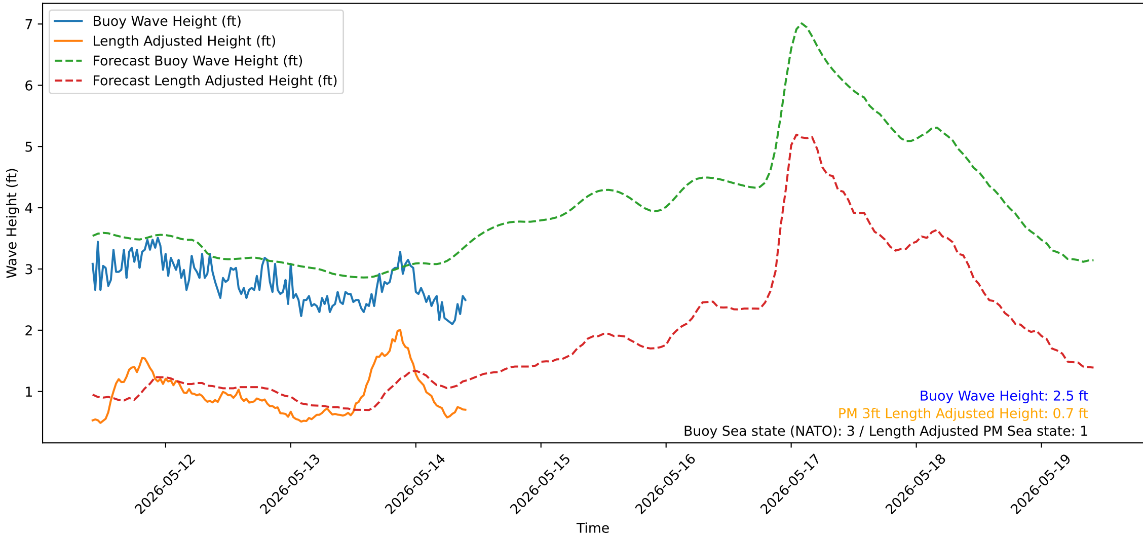
Wave Heights over Time for Green Beach at 2026-05-14 10:11:13
