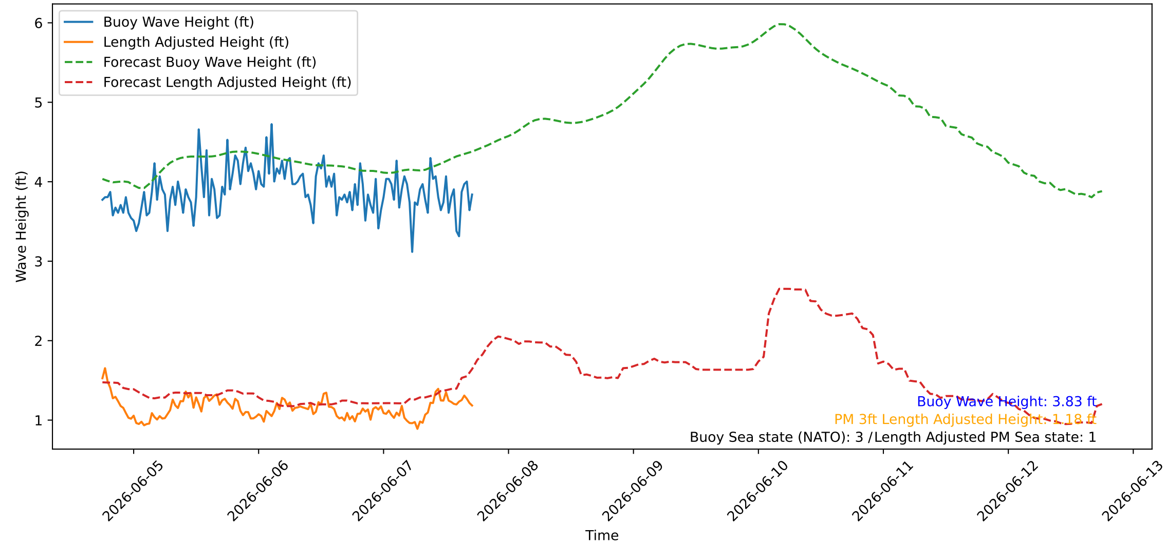
Wave Heights over Time for Green Beach at 2026-06-07 18:01:07
