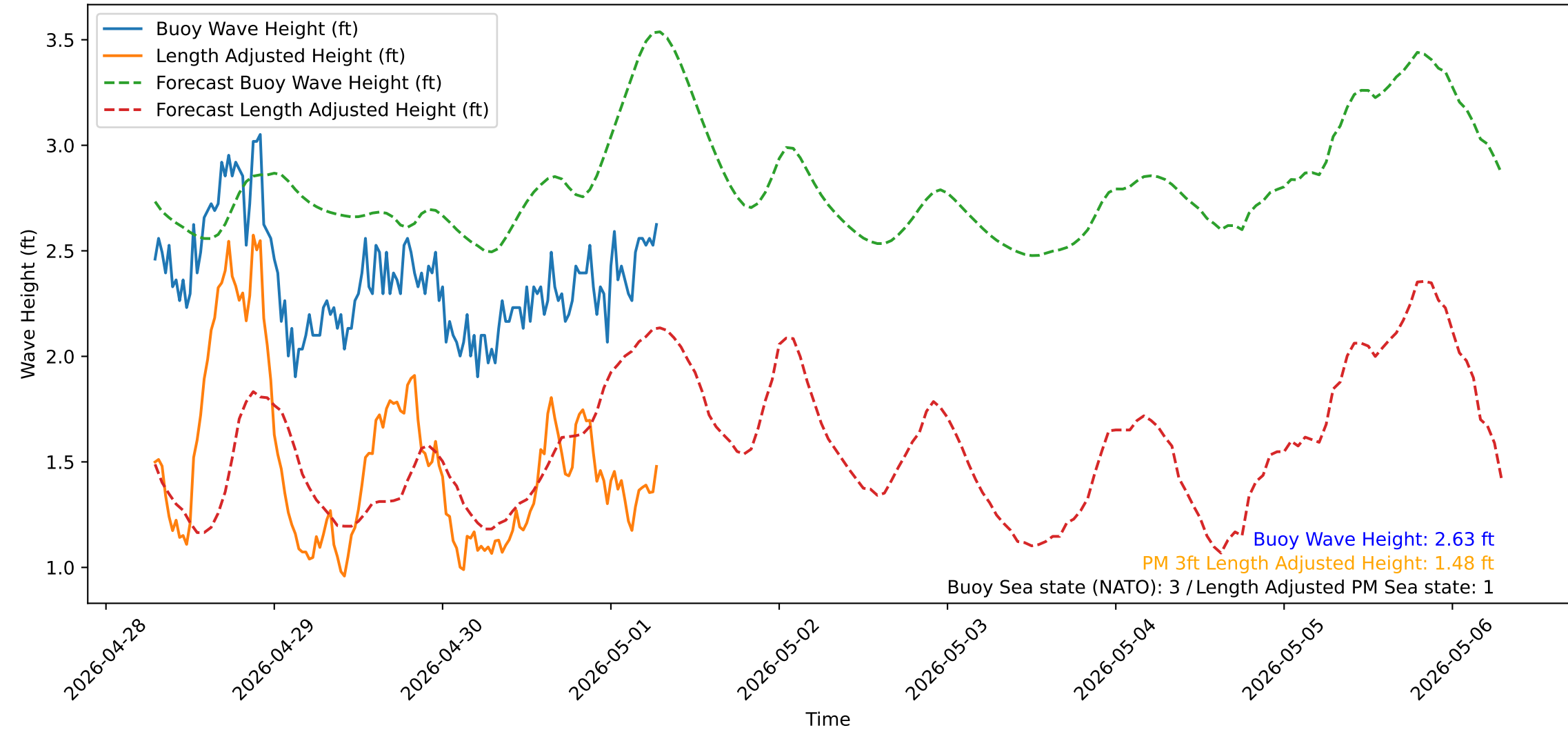
Wave Heights over Time for Oceanside Harbor at 2026-05-01 07:00:31
