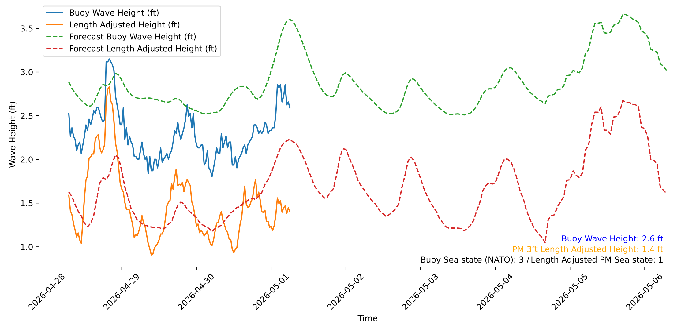
Wave Heights over Time for Green Beach at 2026-05-01 07:01:12
