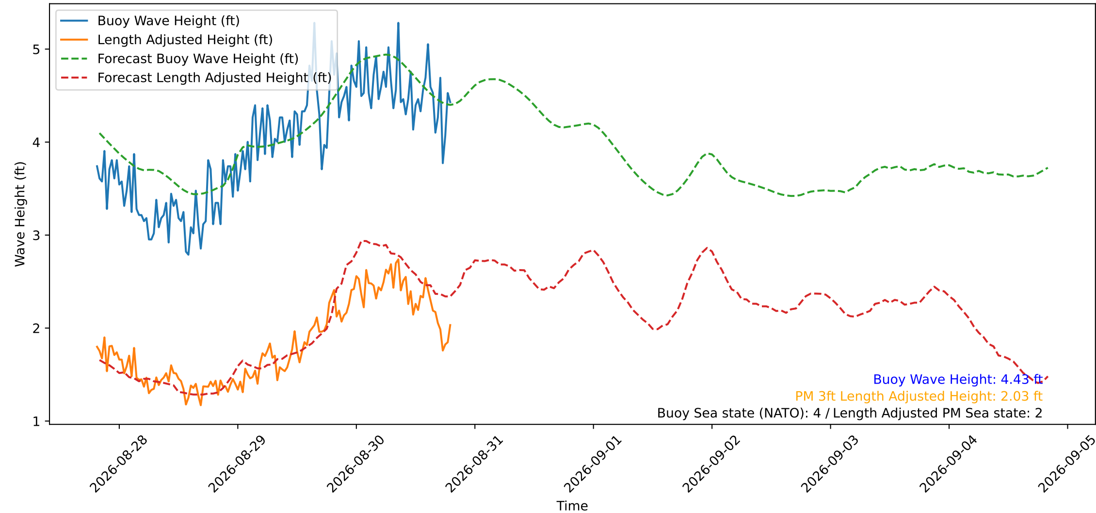
Wave Heights over Time for Oceanside Harbor at 2026-08-30 19:40:29
