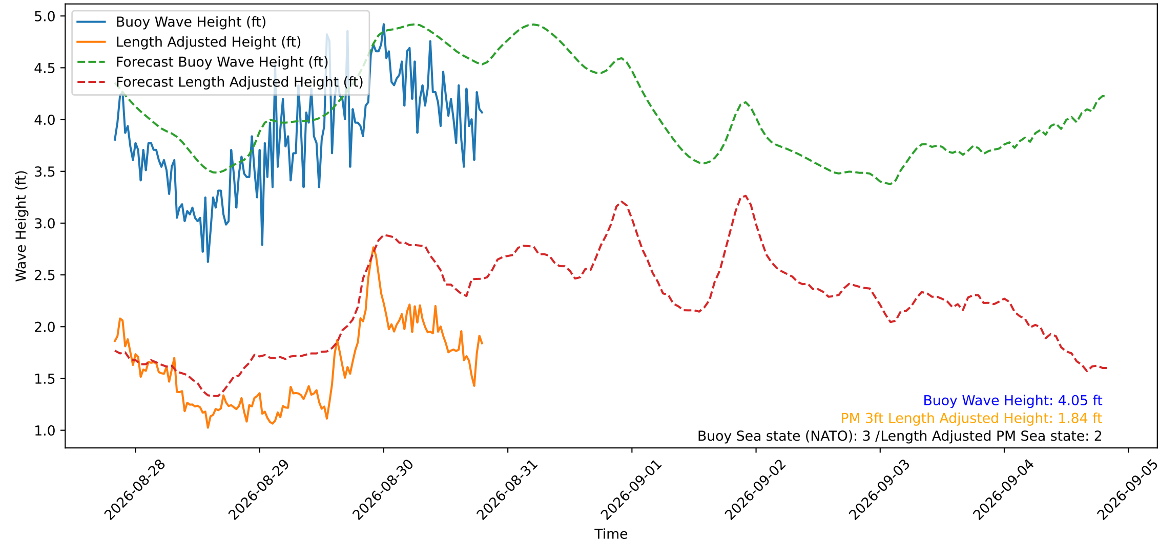
Wave Heights over Time for Green Beach at 2026-08-30 19:41:12
