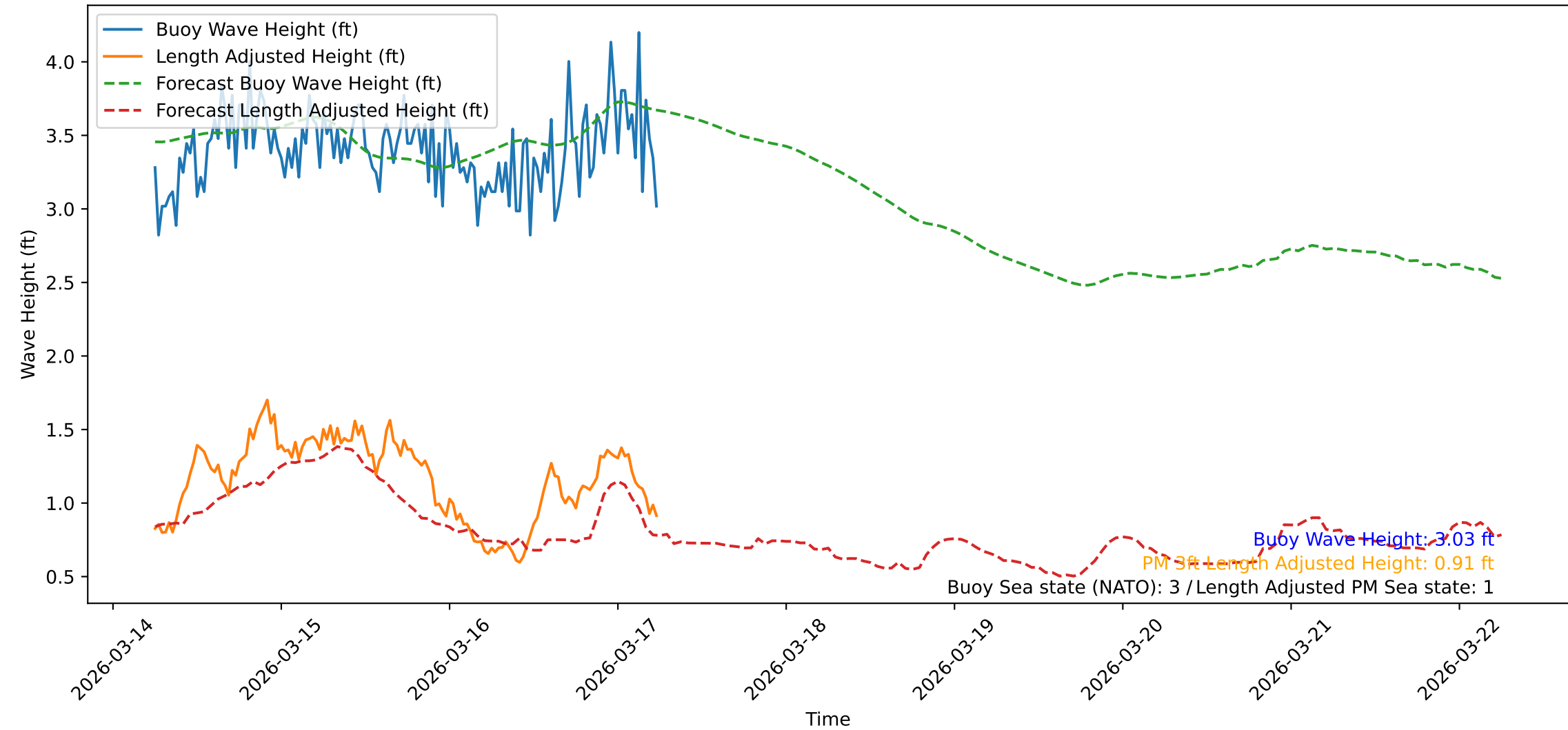
Wave Heights over Time for Green Beach at 2026-03-17 06:11:51
