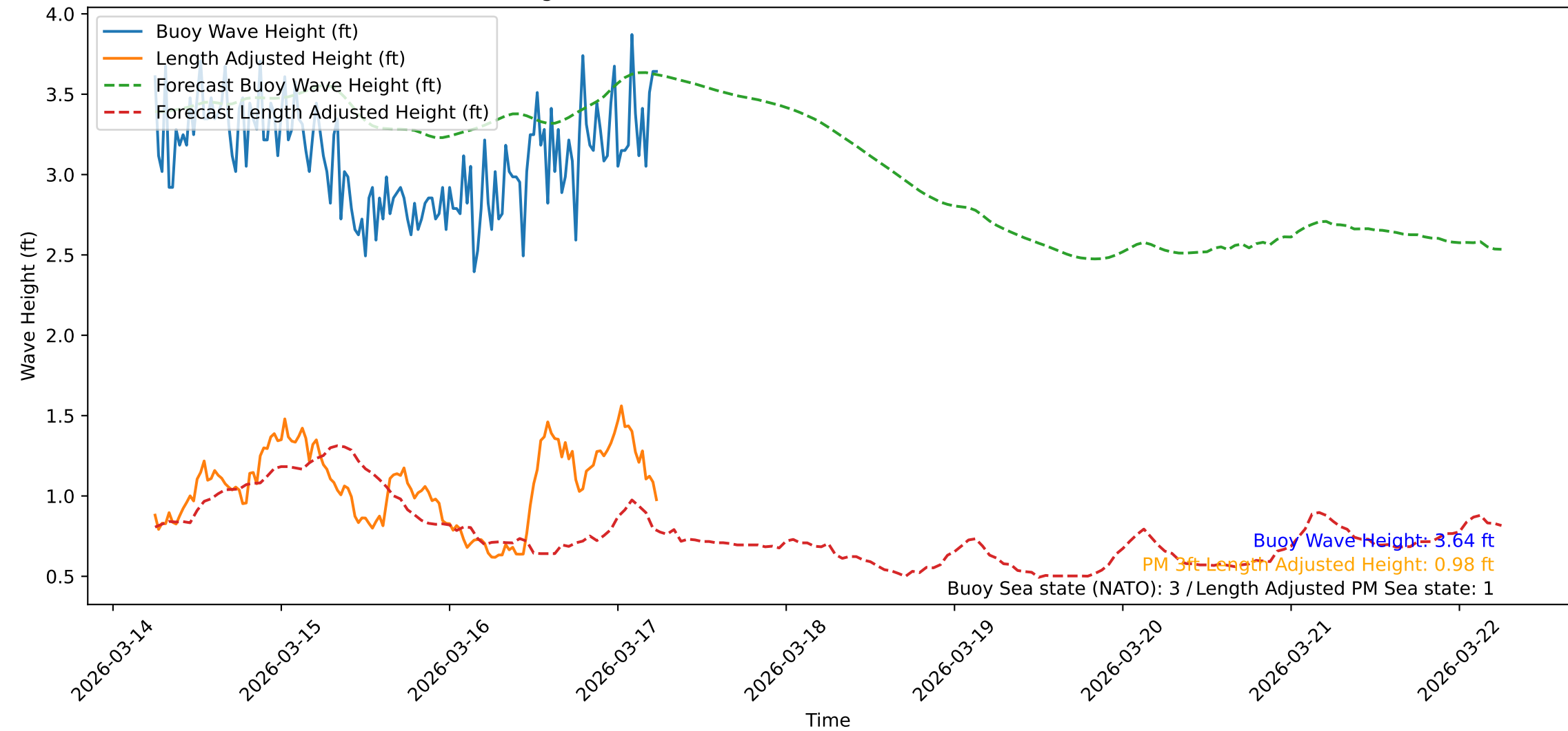
Wave Heights over Time for Oceanside Harbor at 2026-03-17 06:10:49
