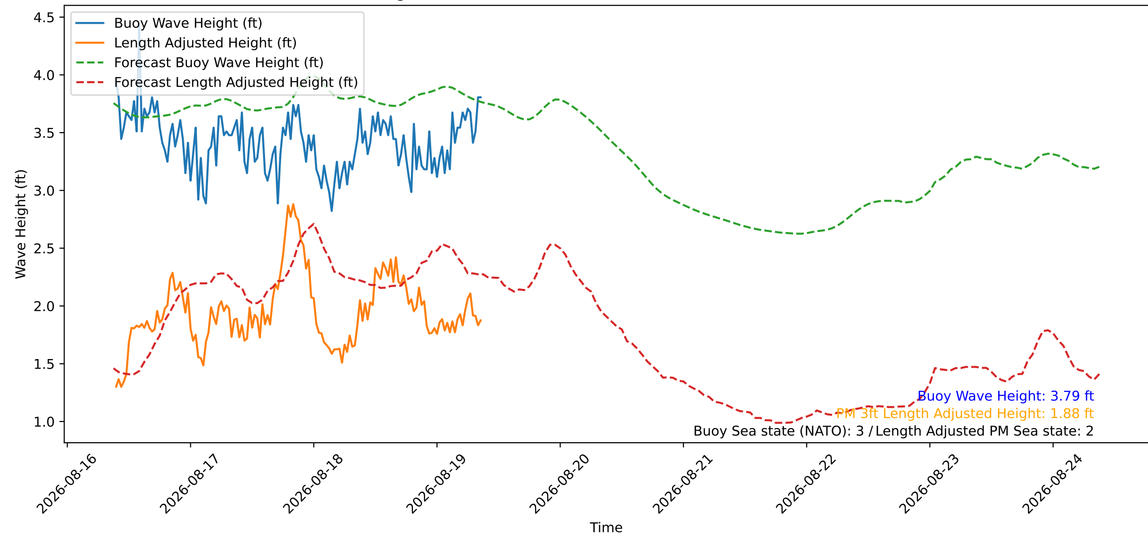
Wave Heights over Time for Oceanside Harbor at 2026-08-19 09:20:26
