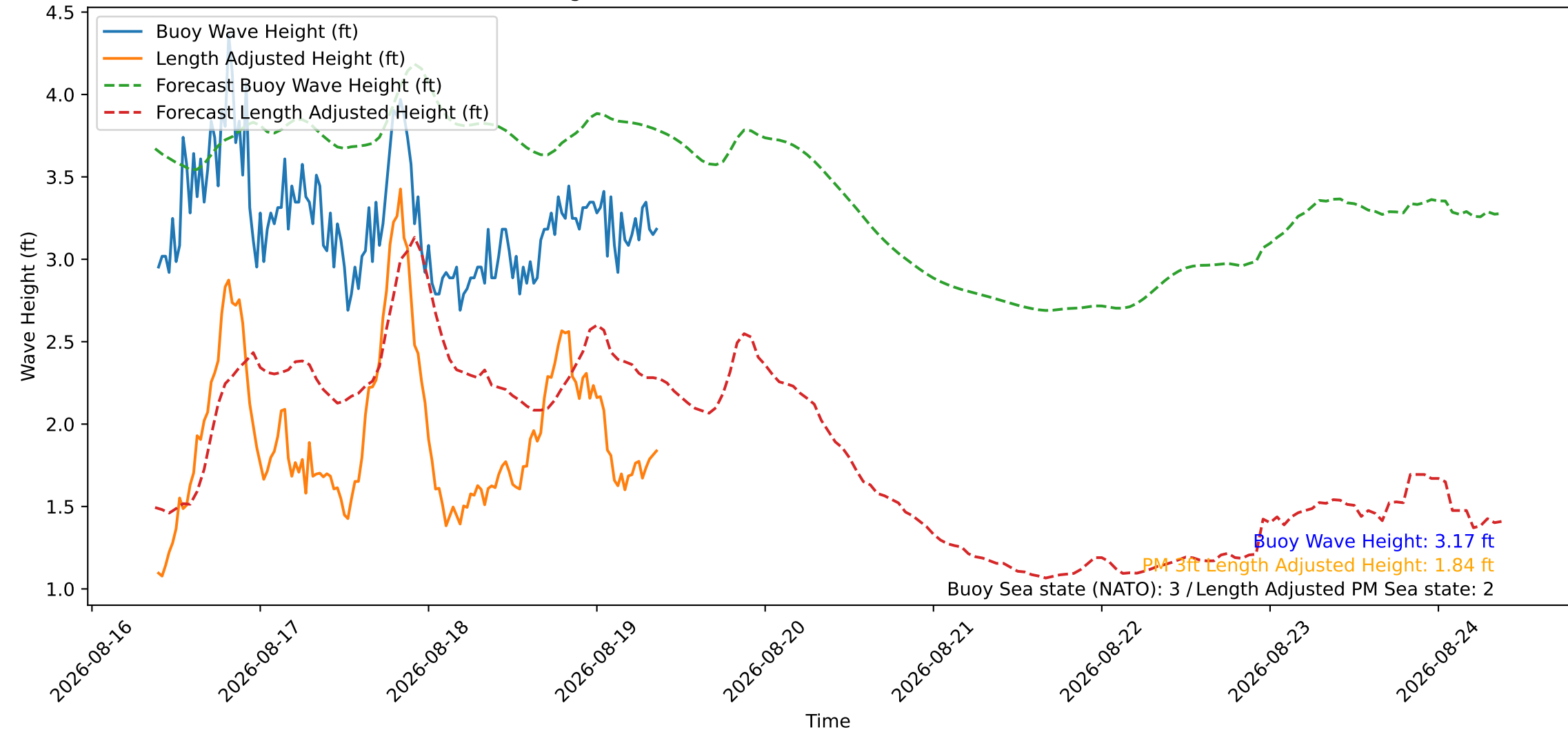
Wave Heights over Time for Green Beach at 2026-08-19 09:21:12
