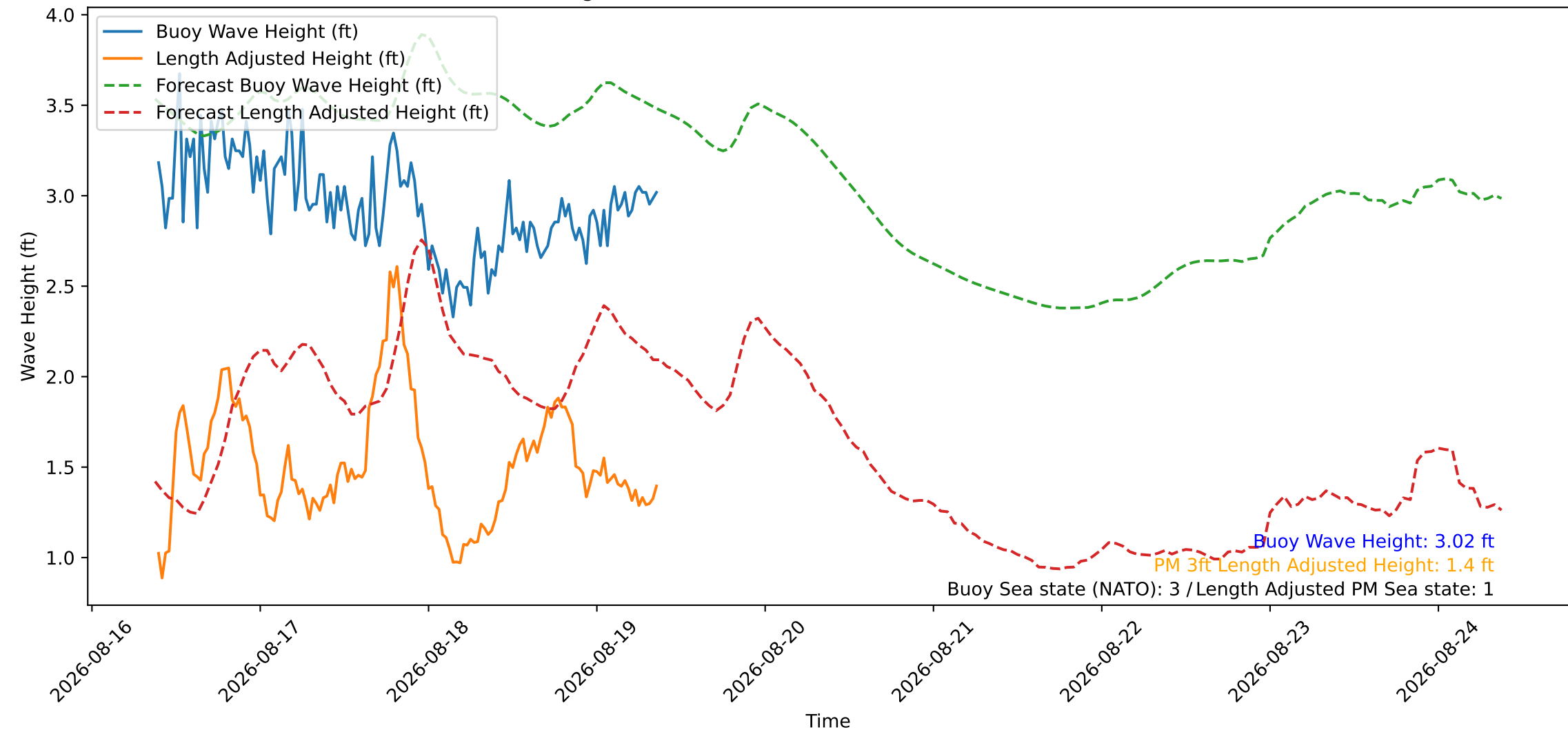
Wave Heights over Time for Red Beach at 2026-08-19 09:20:47
