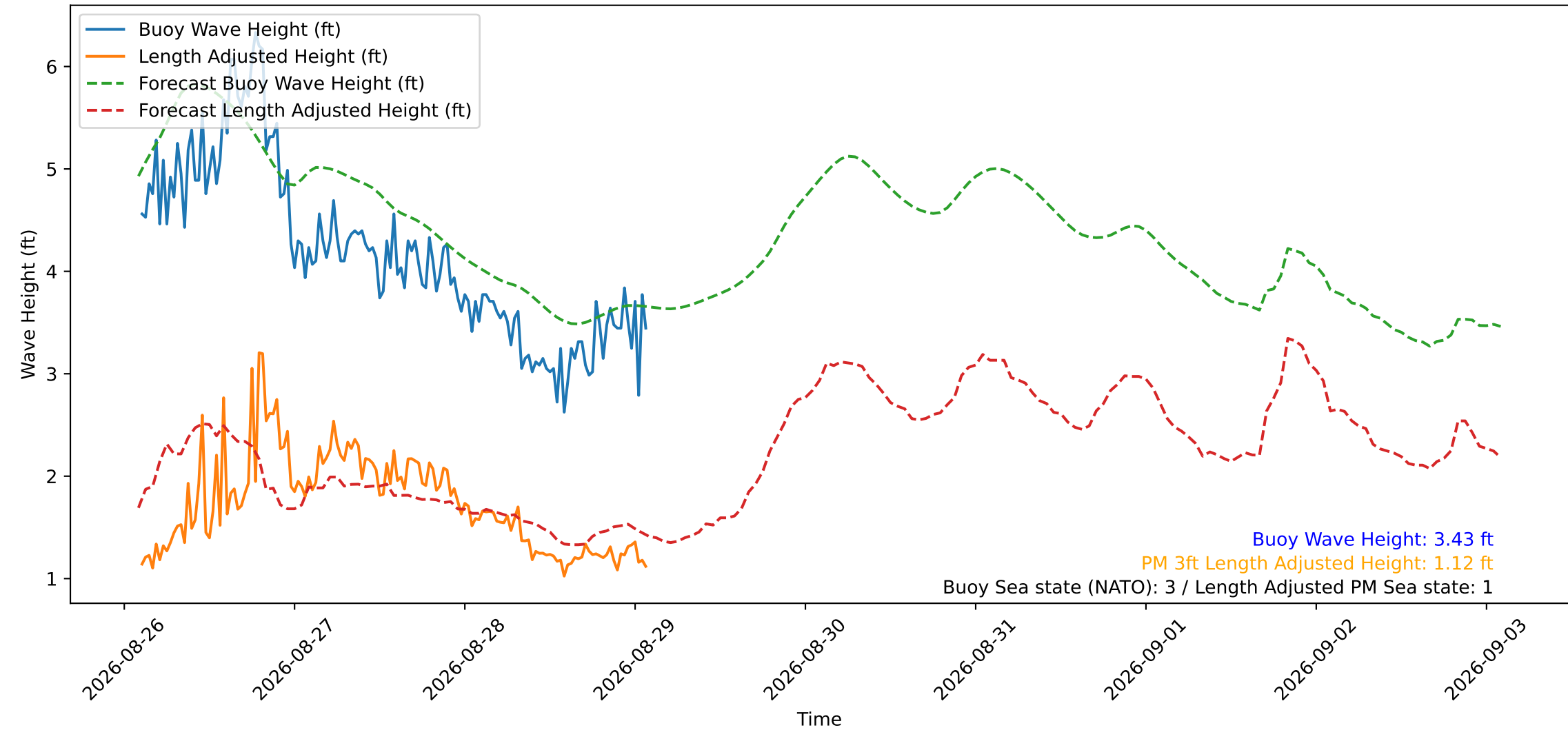
Wave Heights over Time for Green Beach at 2026-08-29 02:11:12
