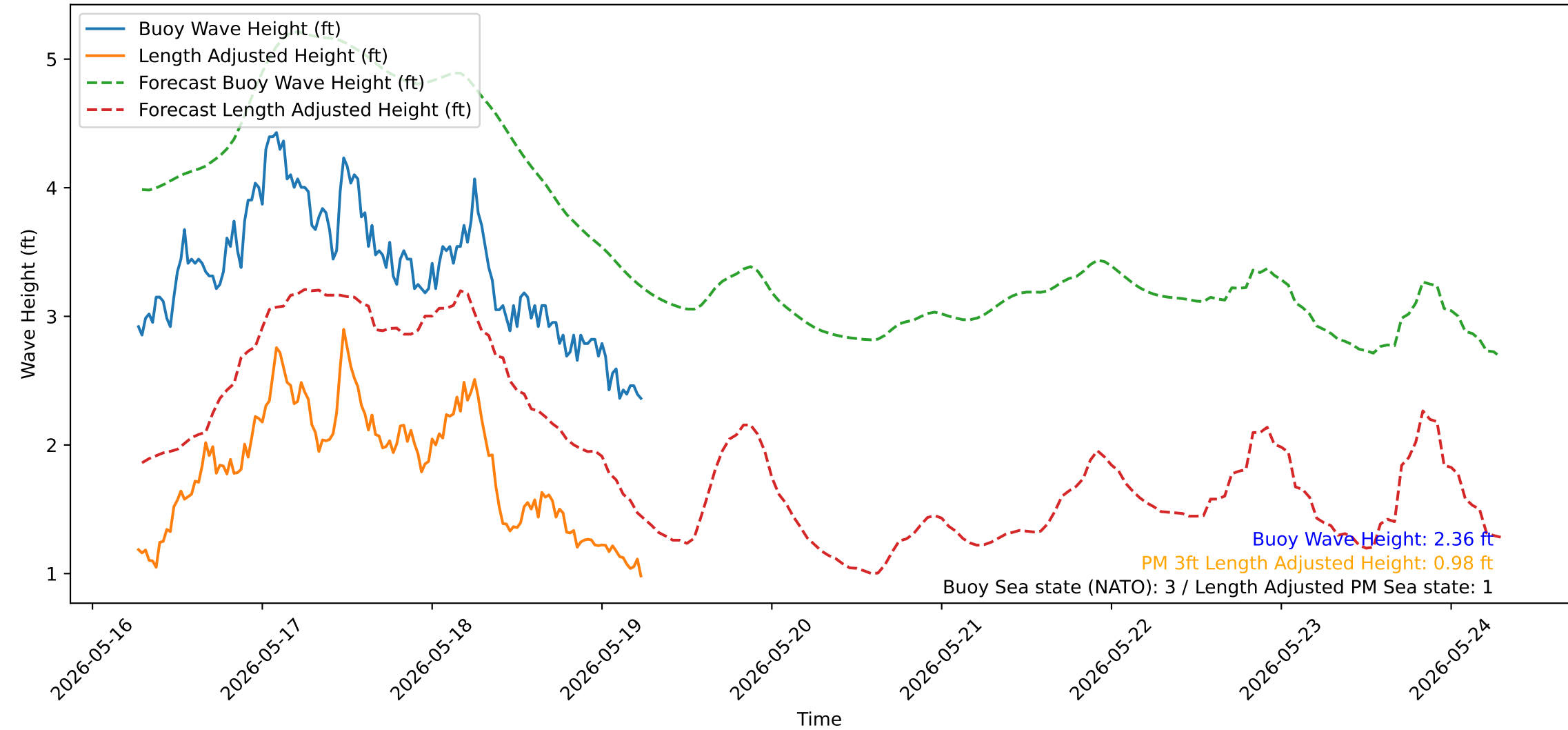
Wave Heights over Time for Green Beach at 2026-05-19 06:31:14
