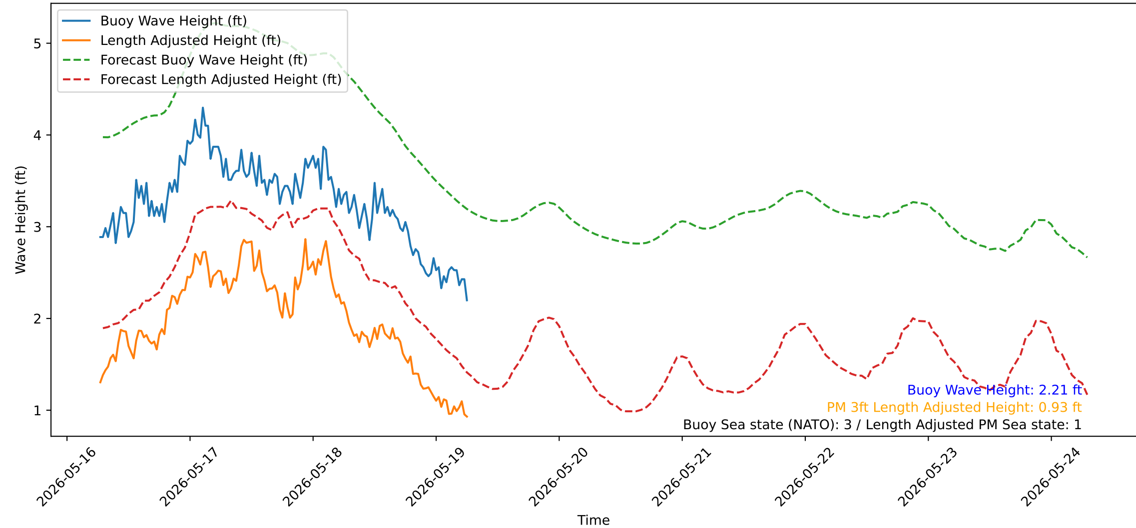
Wave Heights over Time for Oceanside Harbor at 2026-05-19 06:30:31
