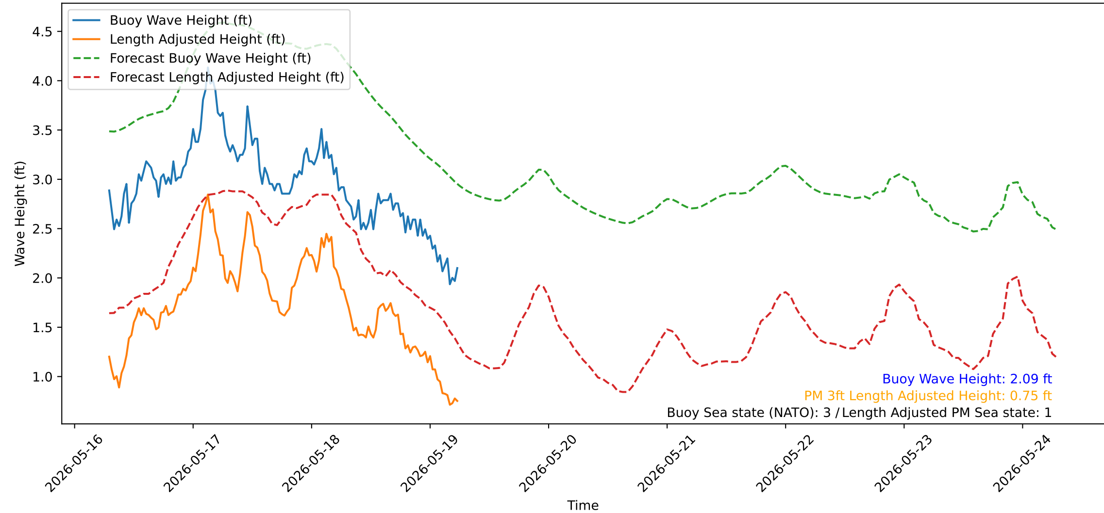
Wave Heights over Time for Red Beach at 2026-05-19 06:30:50
