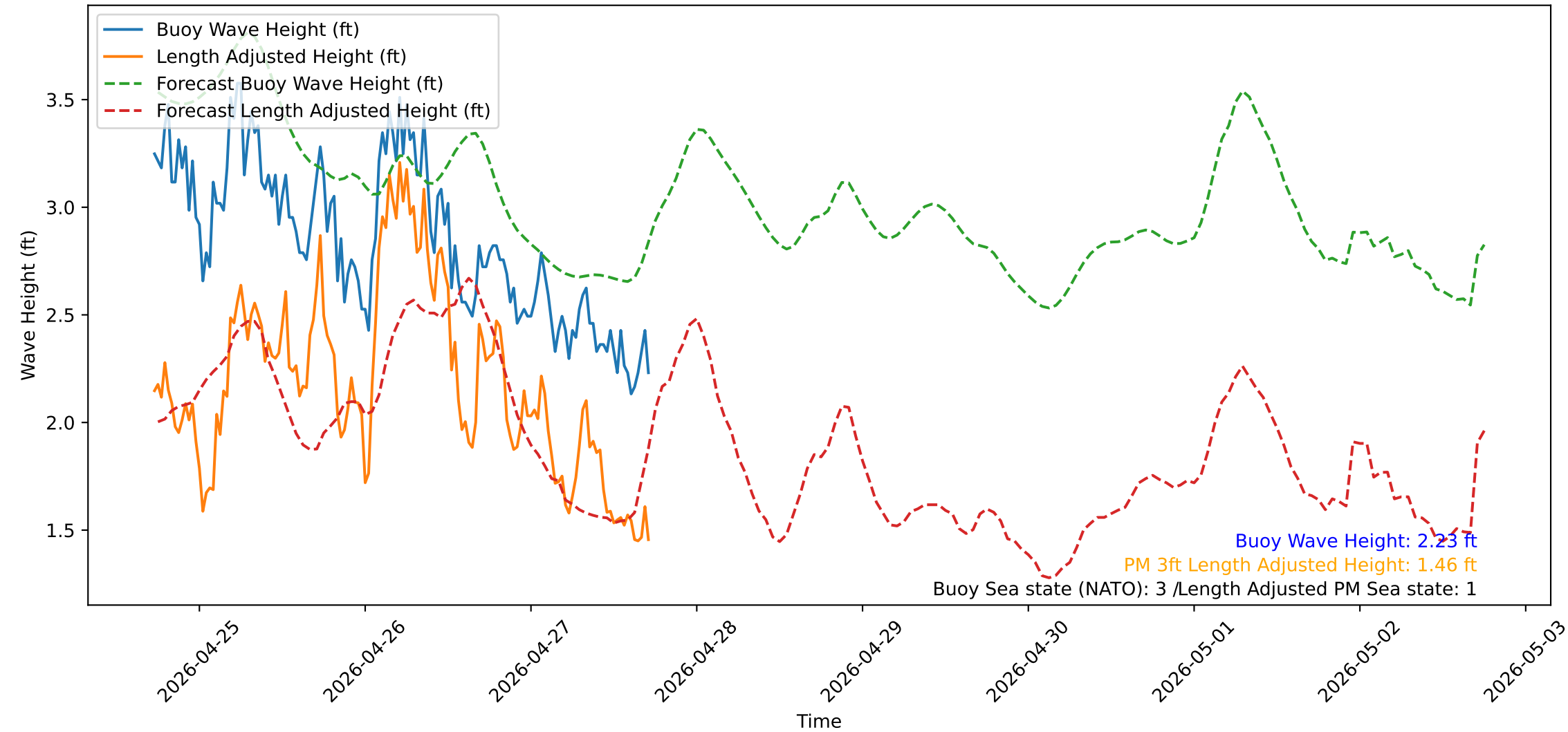
Wave Heights over Time for Green Beach at 2026-04-27 17:41:13
