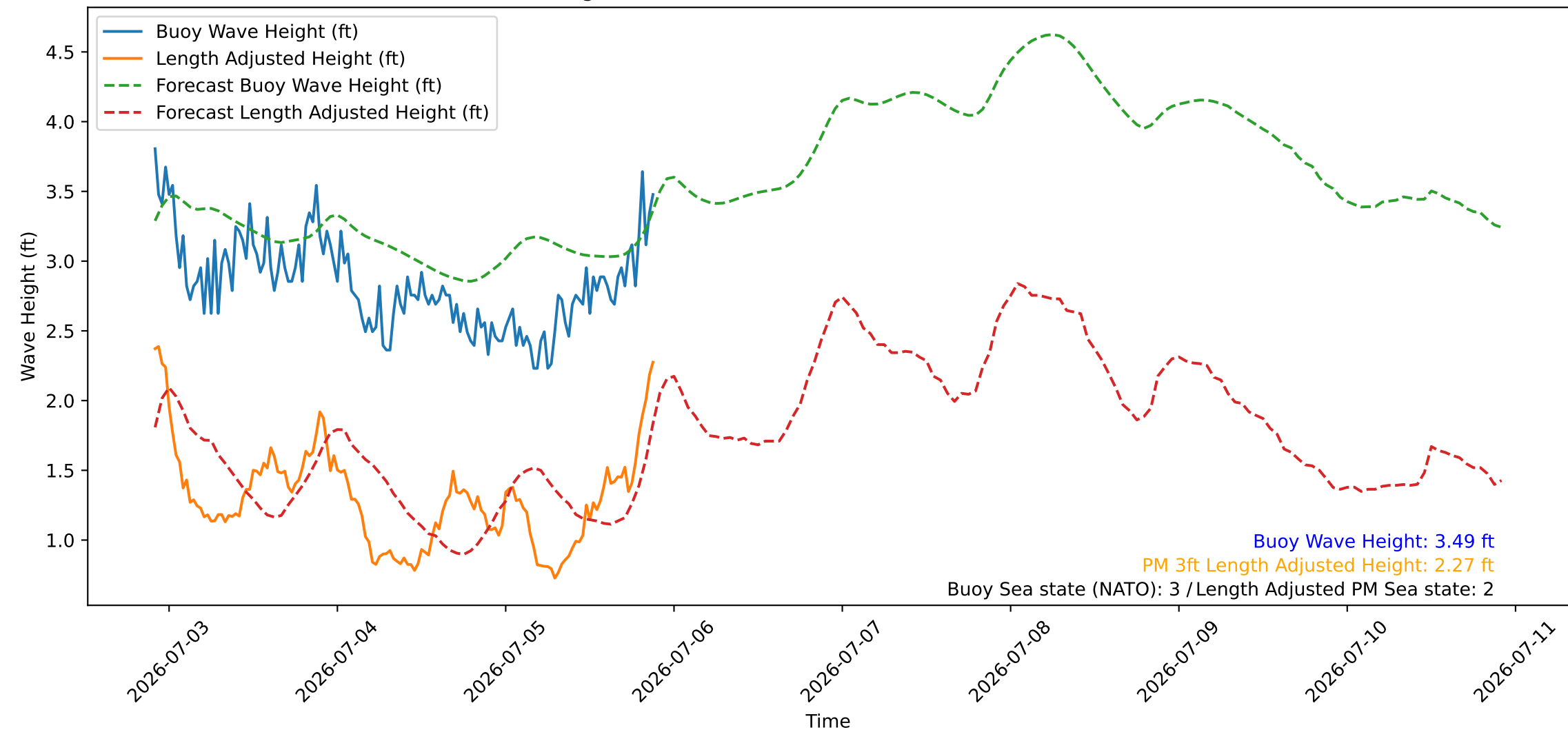
Wave Heights over Time for Red Beach at 2026-07-05 21:40:47
