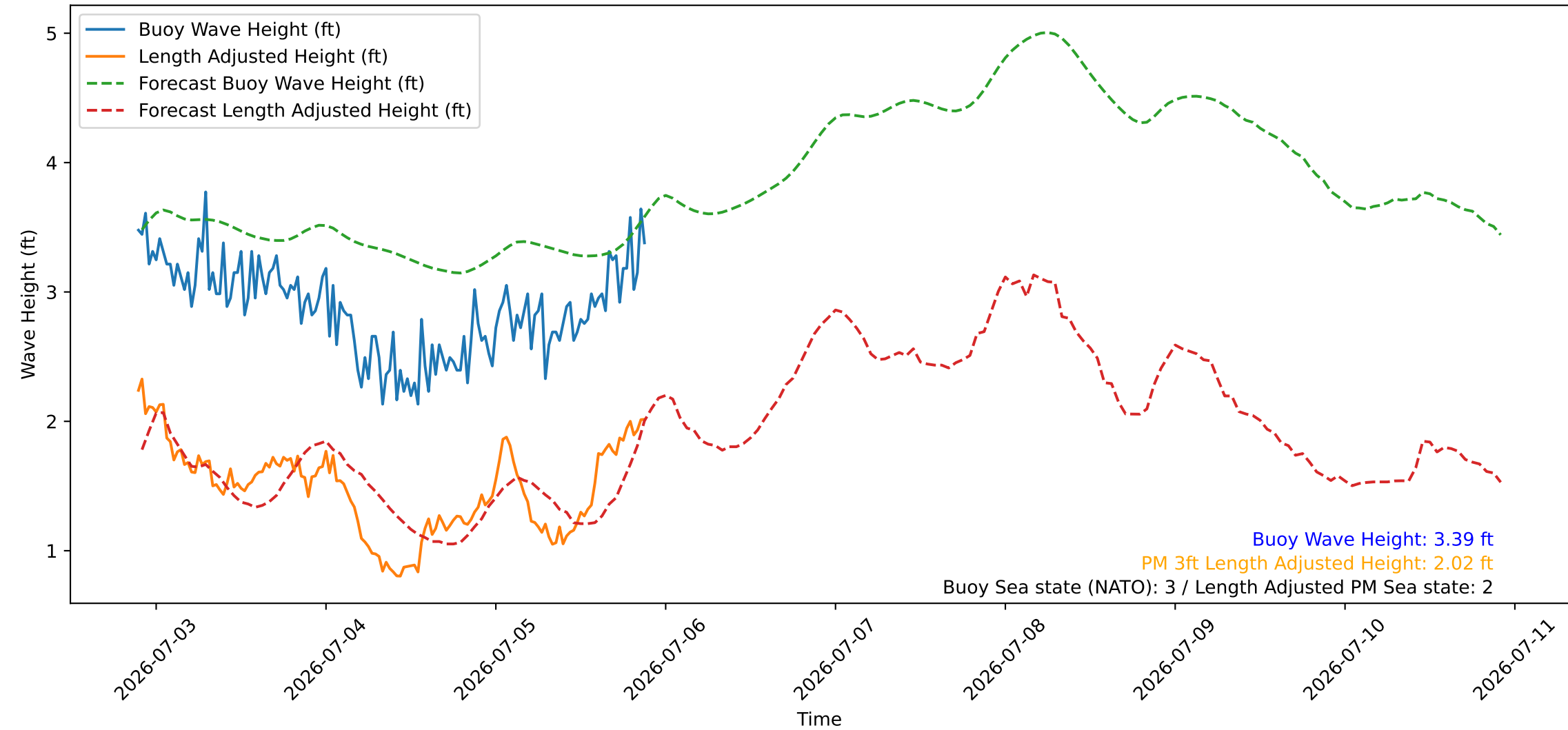
Wave Heights over Time for Oceanside Harbor at 2026-07-05 21:40:27
