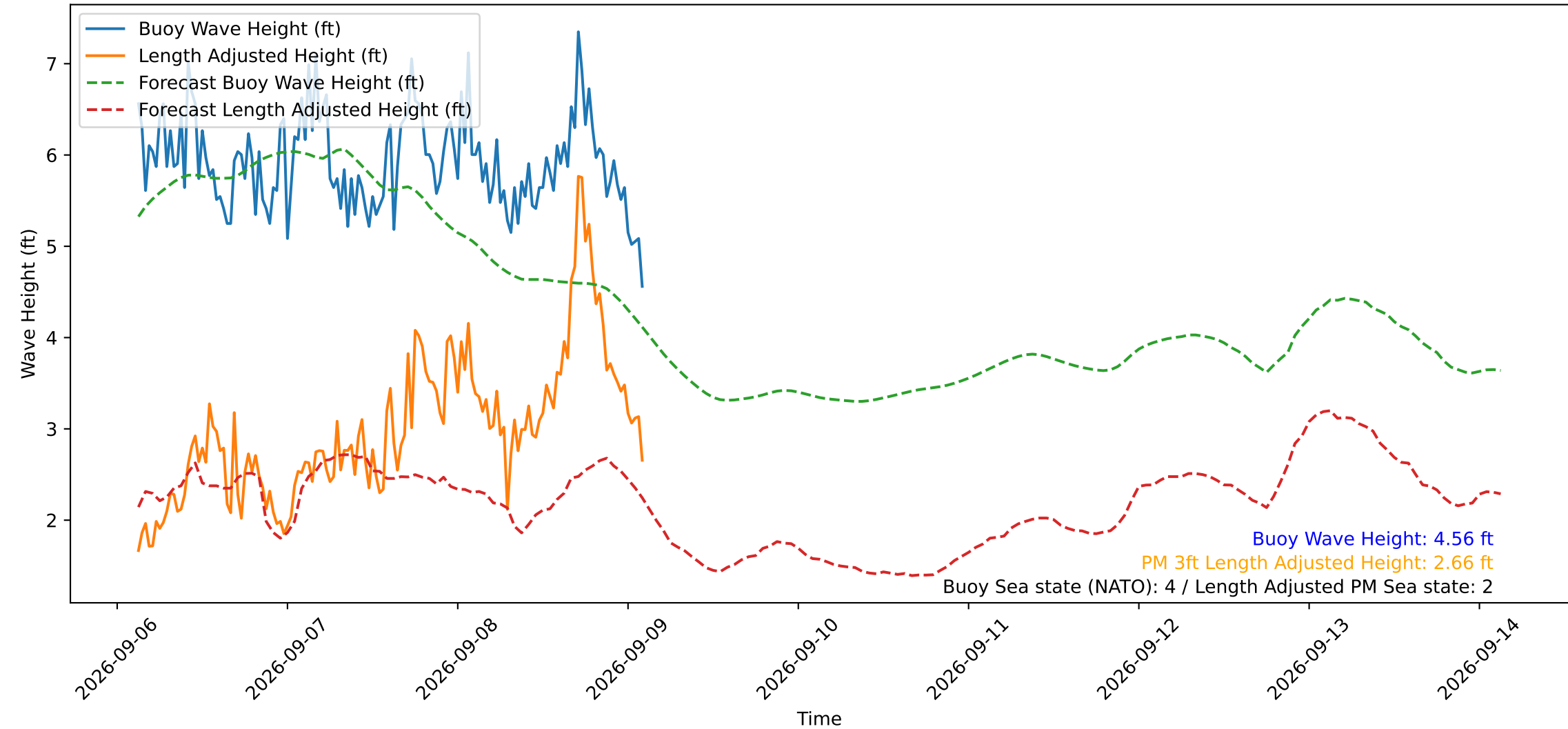
Wave Heights over Time for Oceanside Harbor at 2026-09-09 02:50:29
