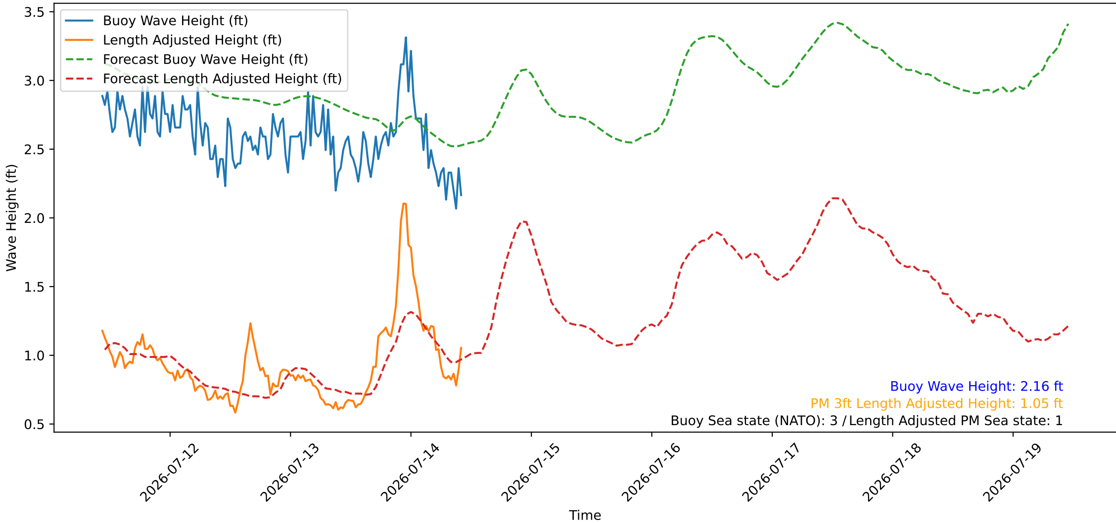
Wave Heights over Time for Green Beach at 2026-07-14 10:41:09
