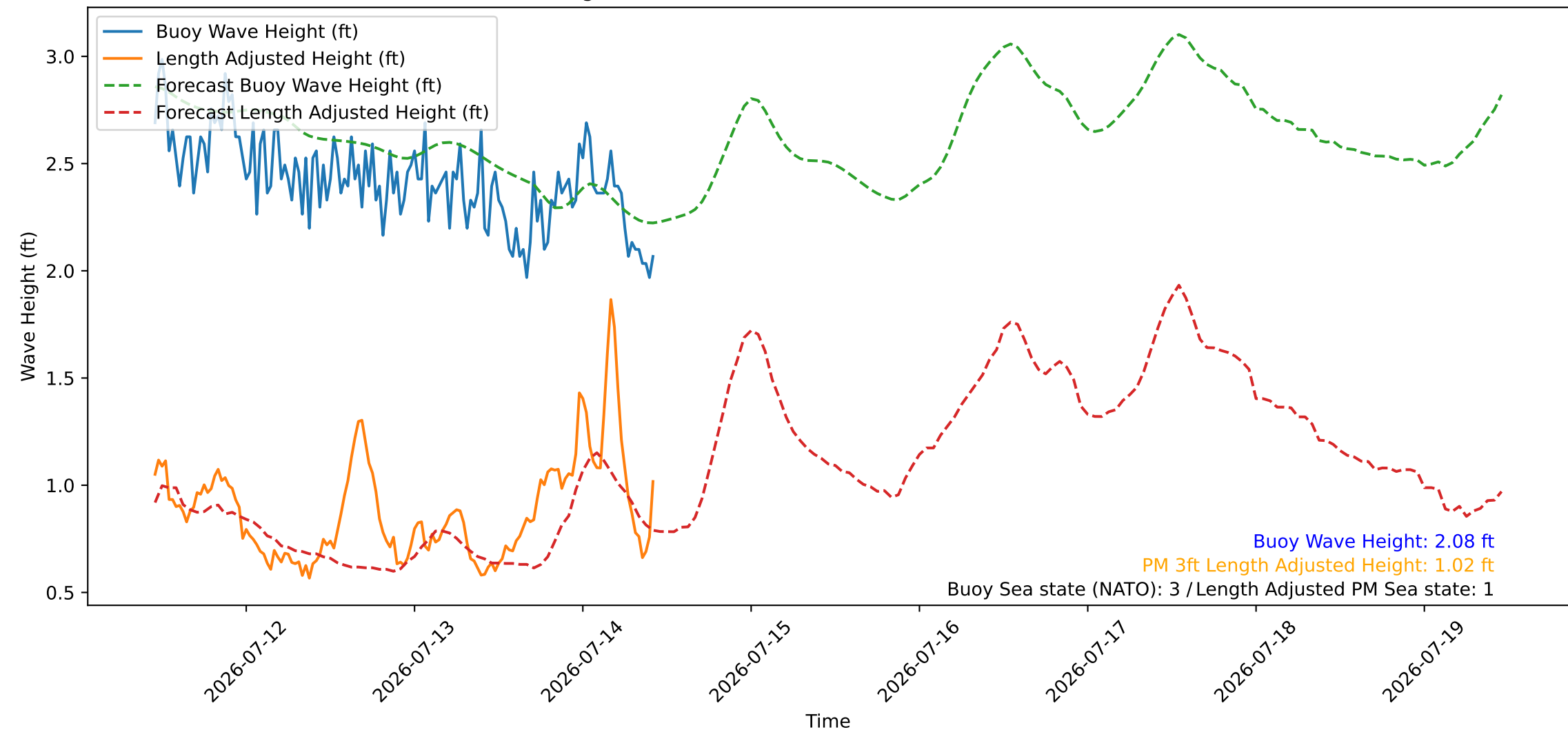
Wave Heights over Time for Red Beach at 2026-07-14 10:40:46
