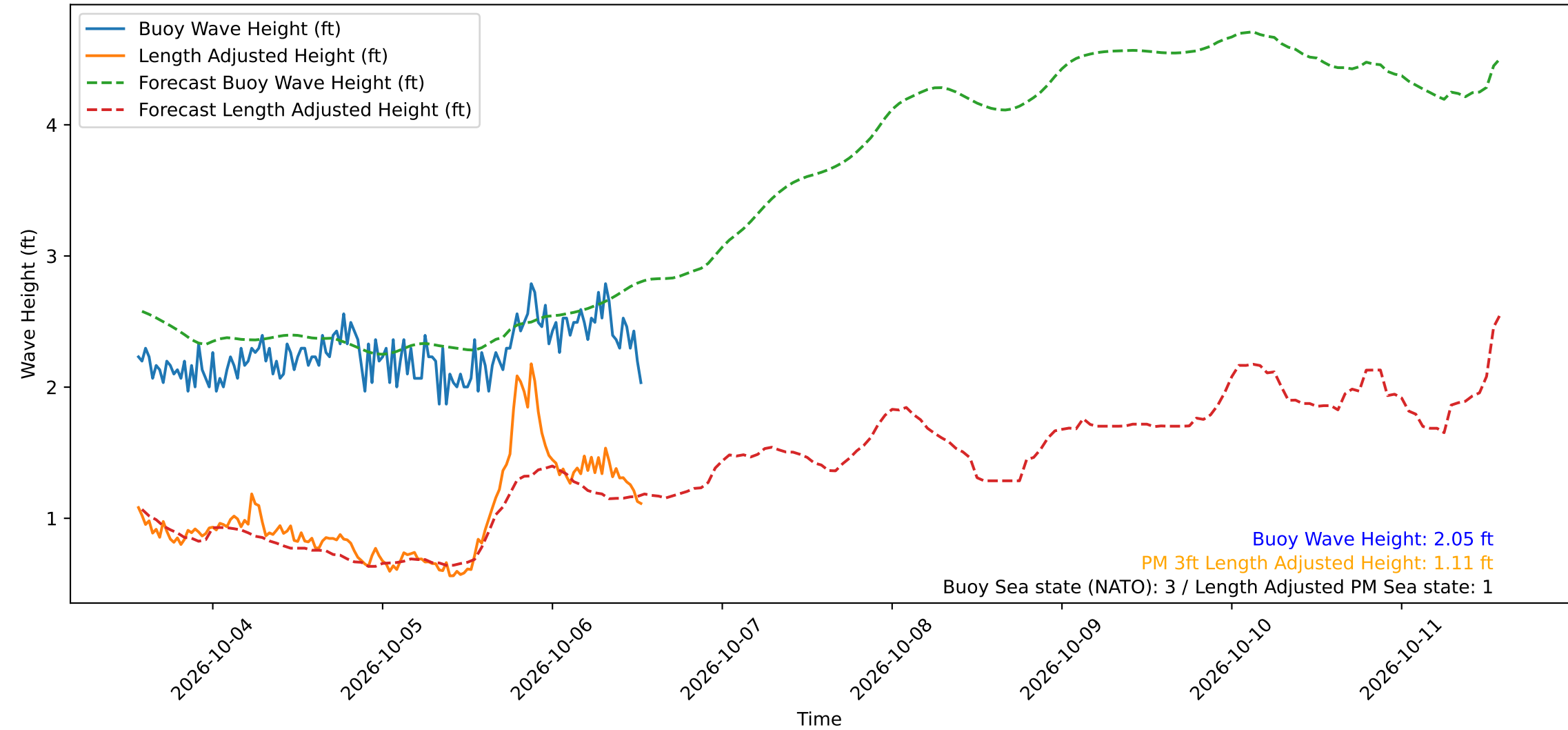
Wave Heights over Time for Oceanside Harbor at 2026-10-06 13:30:30
