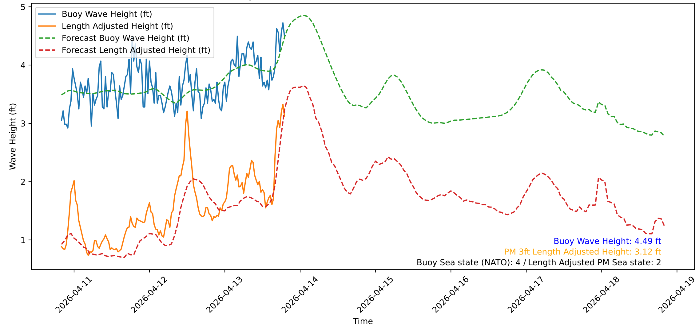
Wave Heights over Time for Green Beach at 2026-04-13 19:51:13
