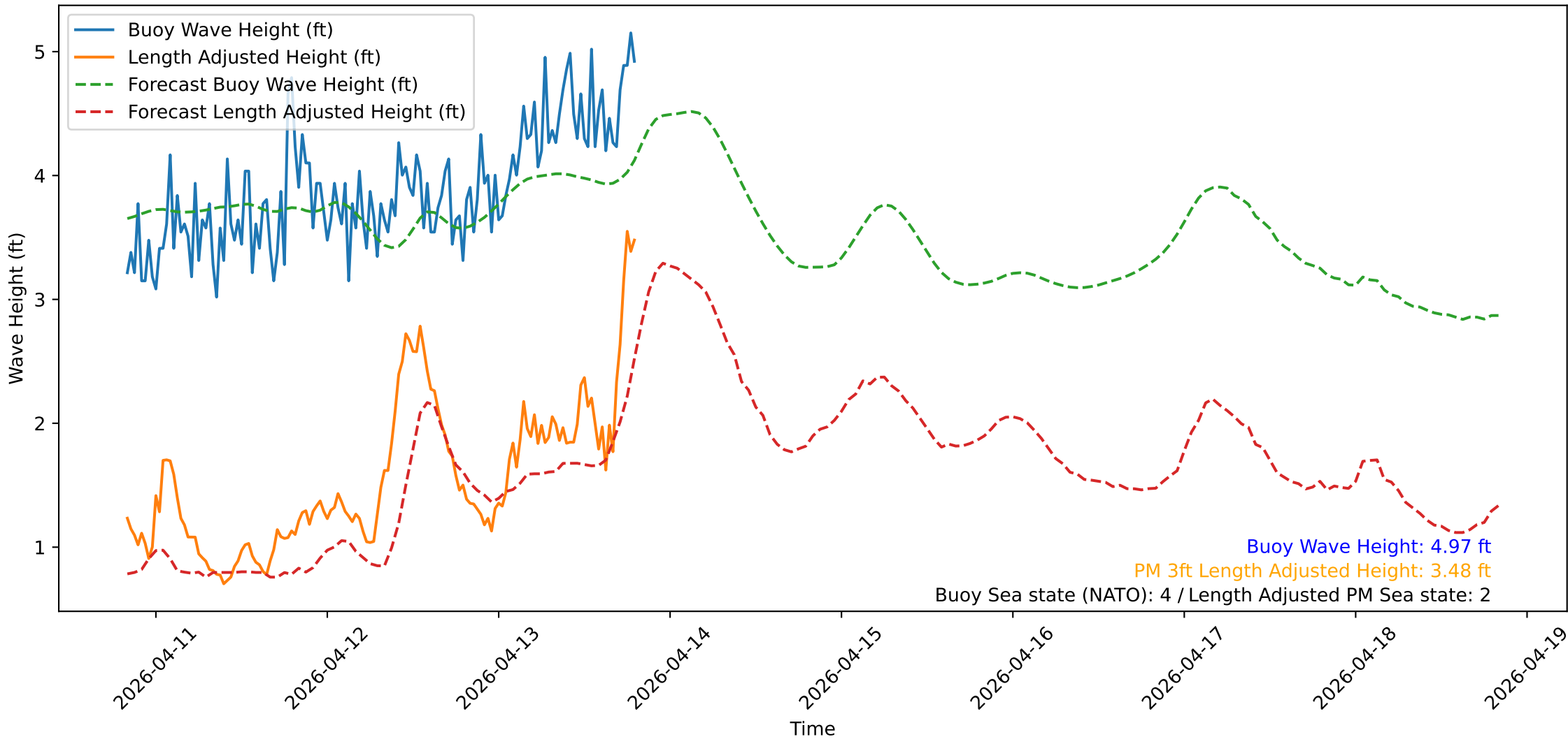
Wave Heights over Time for Oceanside Harbor at 2026-04-13 19:50:32
