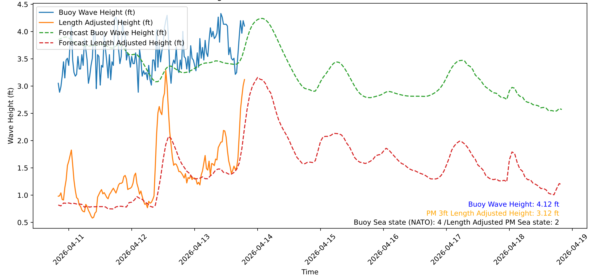
Wave Heights over Time for Red Beach at 2026-04-13 19:50:51
