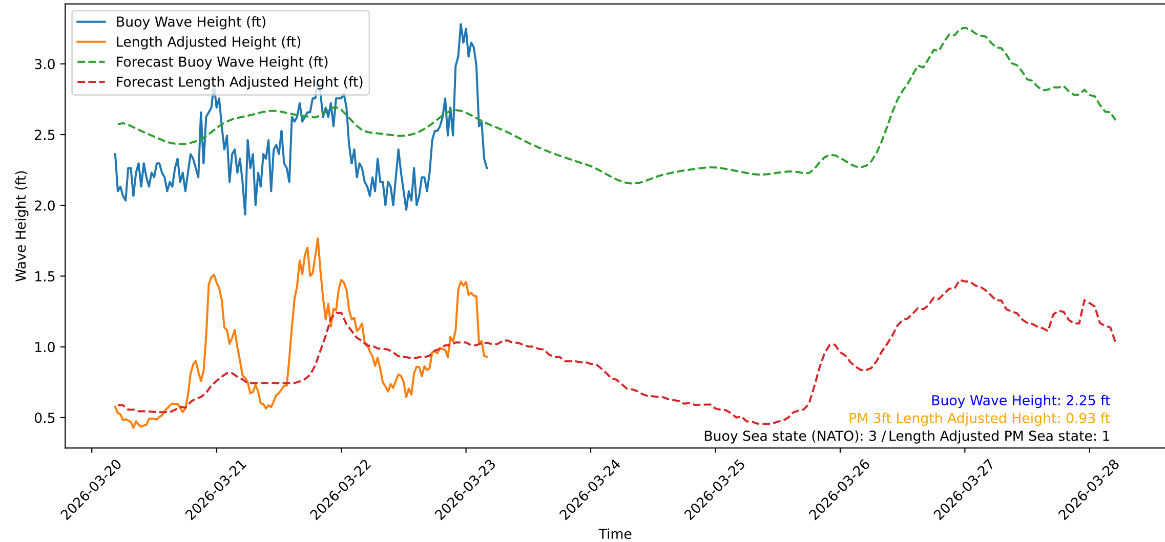
Wave Heights over Time for Green Beach at 2026-03-23 04:41:11
