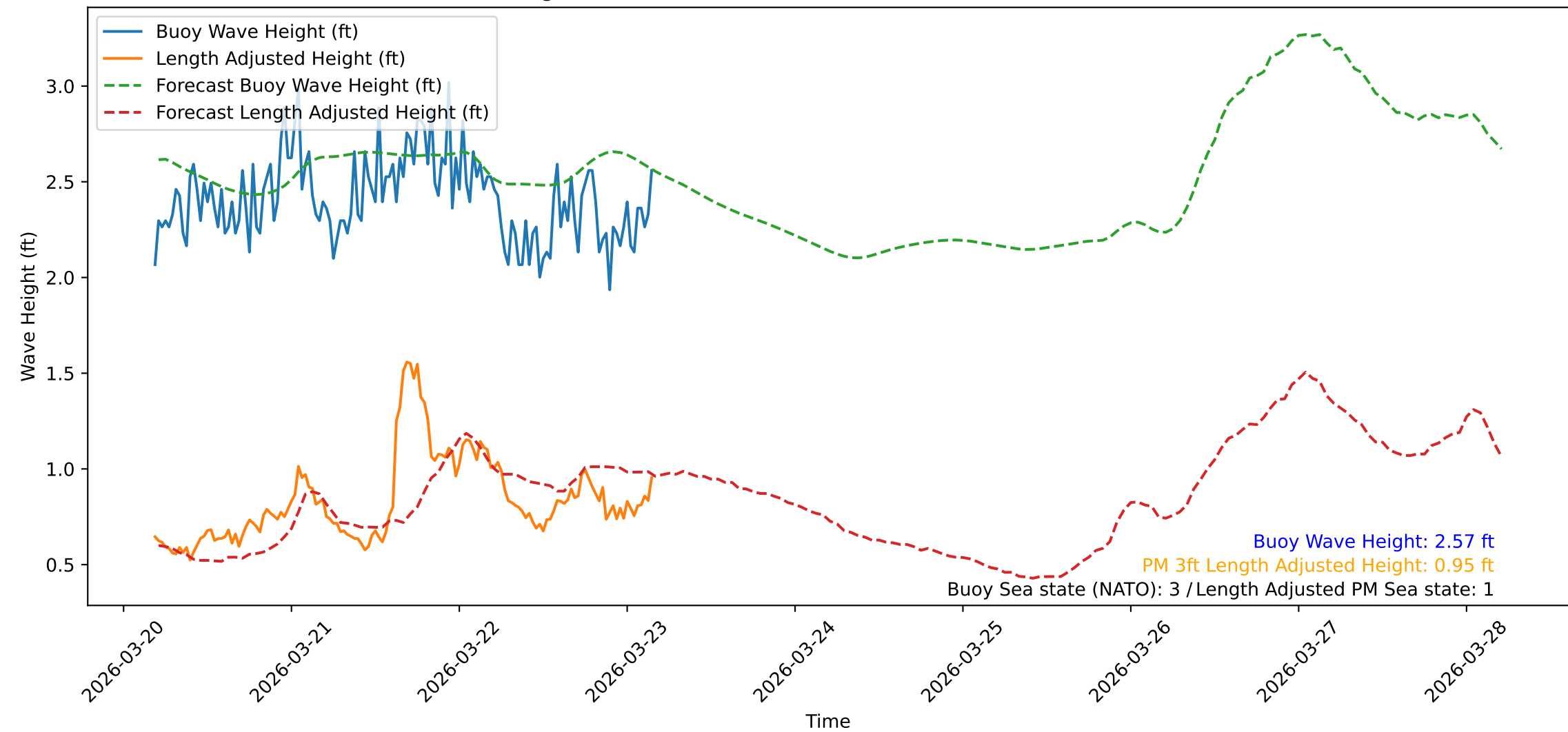
Wave Heights over Time for Oceanside Harbor at 2026-03-23 04:40:32
