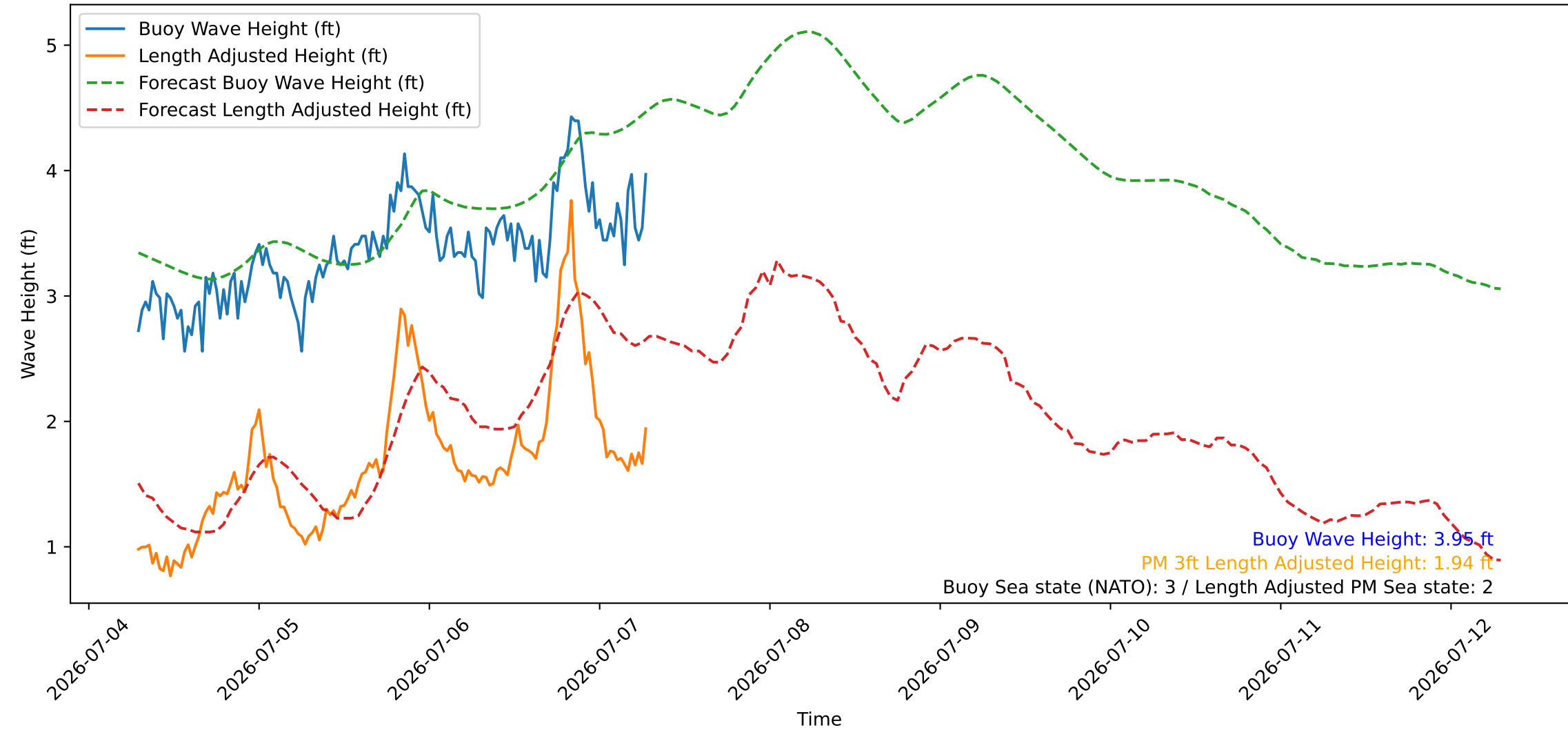
Wave Heights over Time for Green Beach at 2026-07-07 07:11:09
