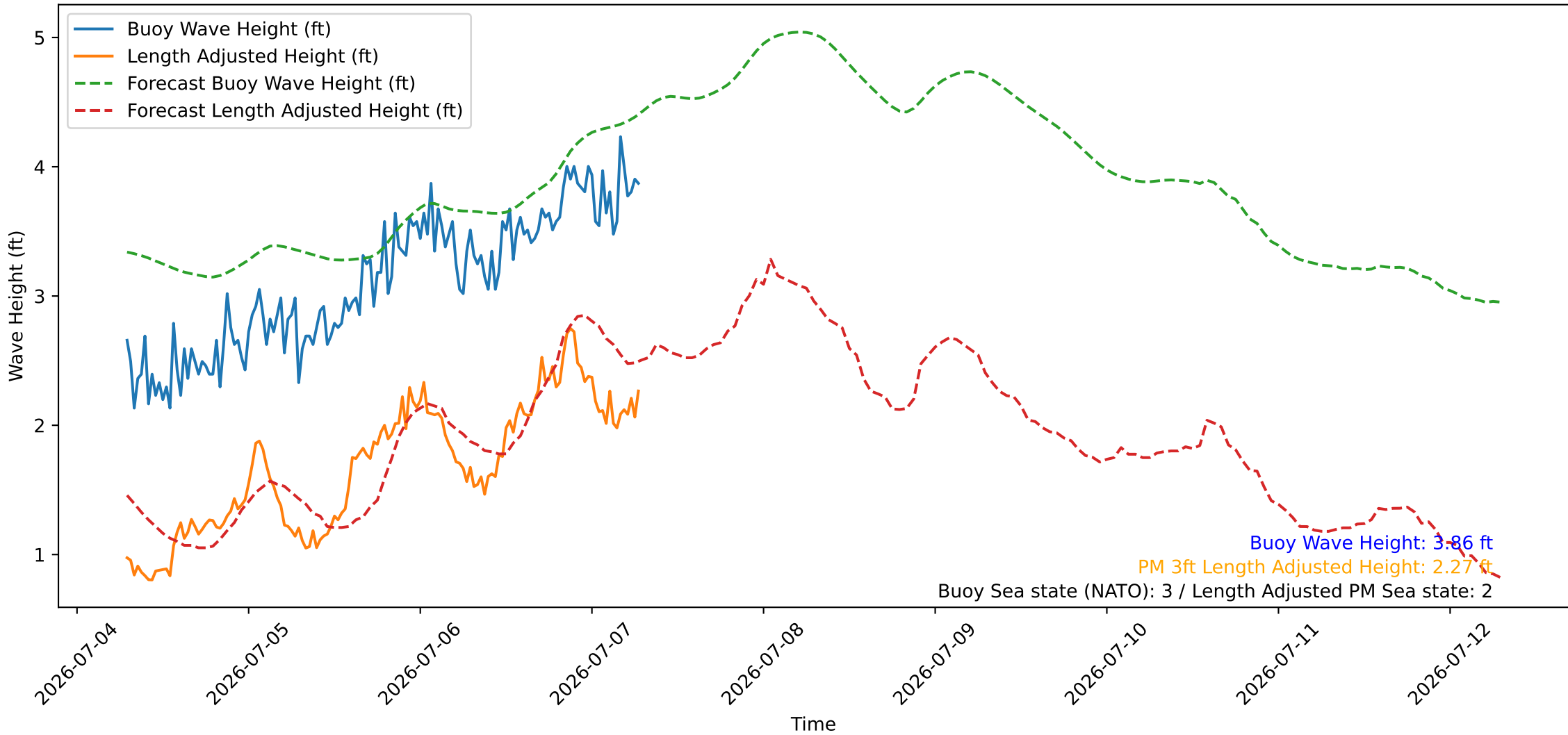
Wave Heights over Time for Oceanside Harbor at 2026-07-07 07:10:26
