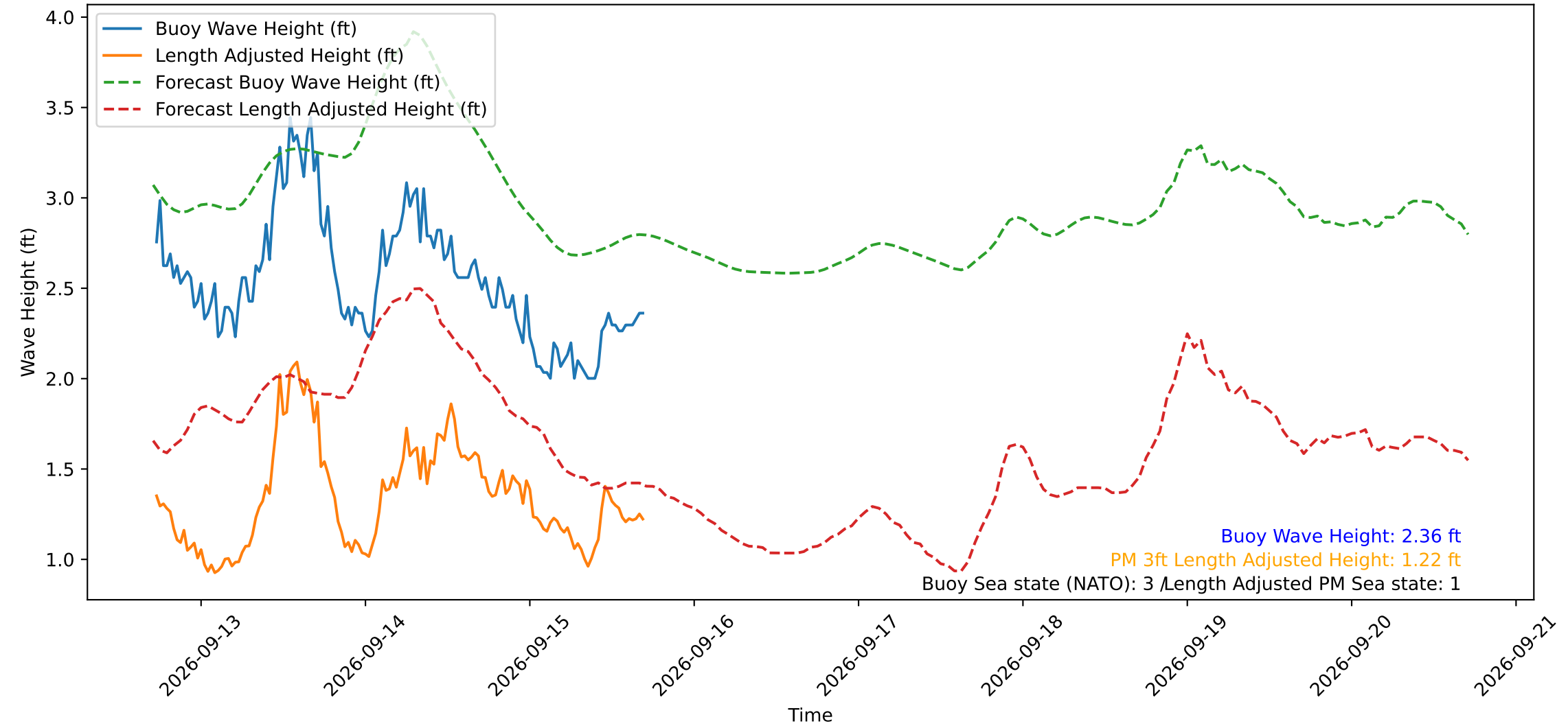
Wave Heights over Time for Red Beach at 2026-09-15 17:10:49
