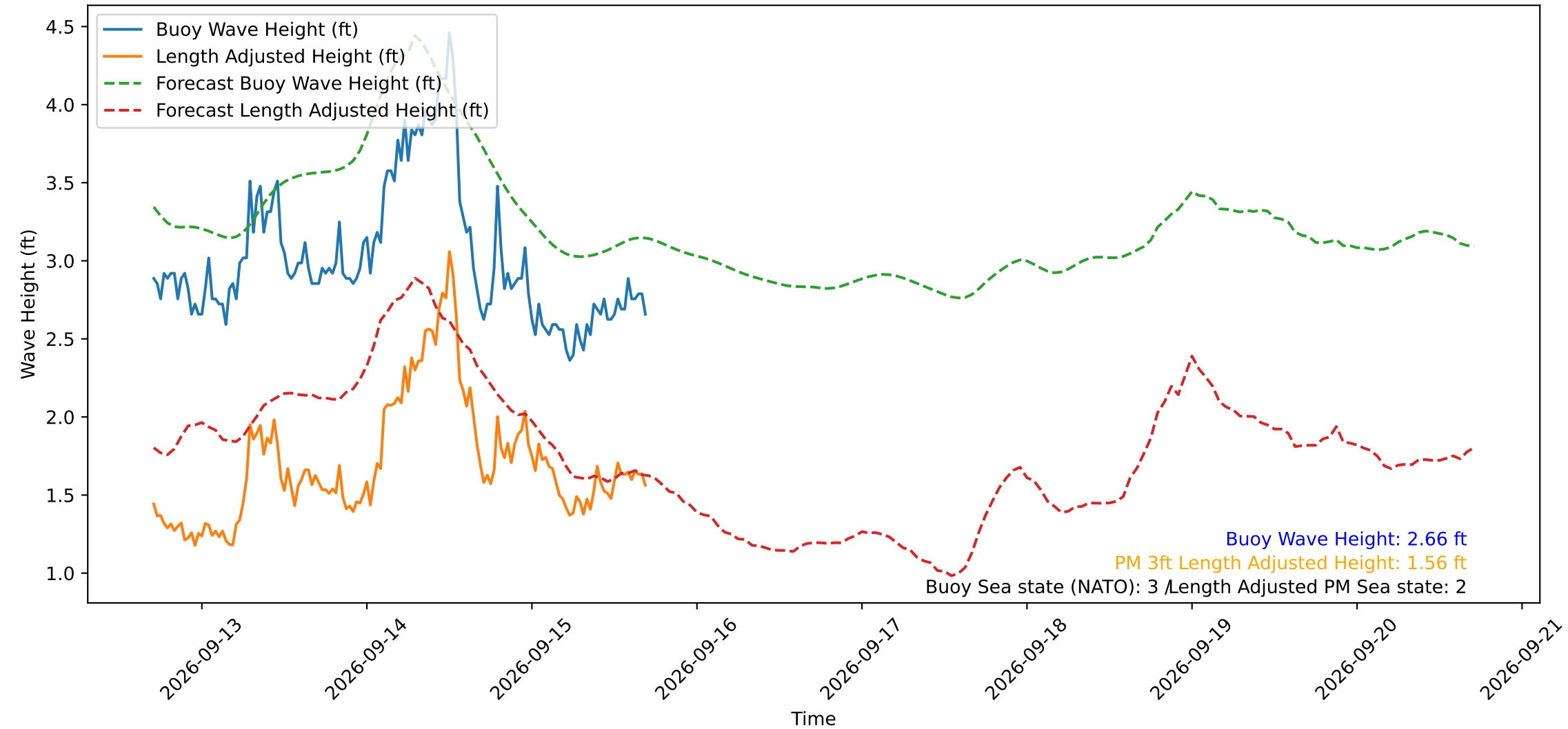
Wave Heights over Time for Oceanside Harbor at 2026-09-15 17:10:30
