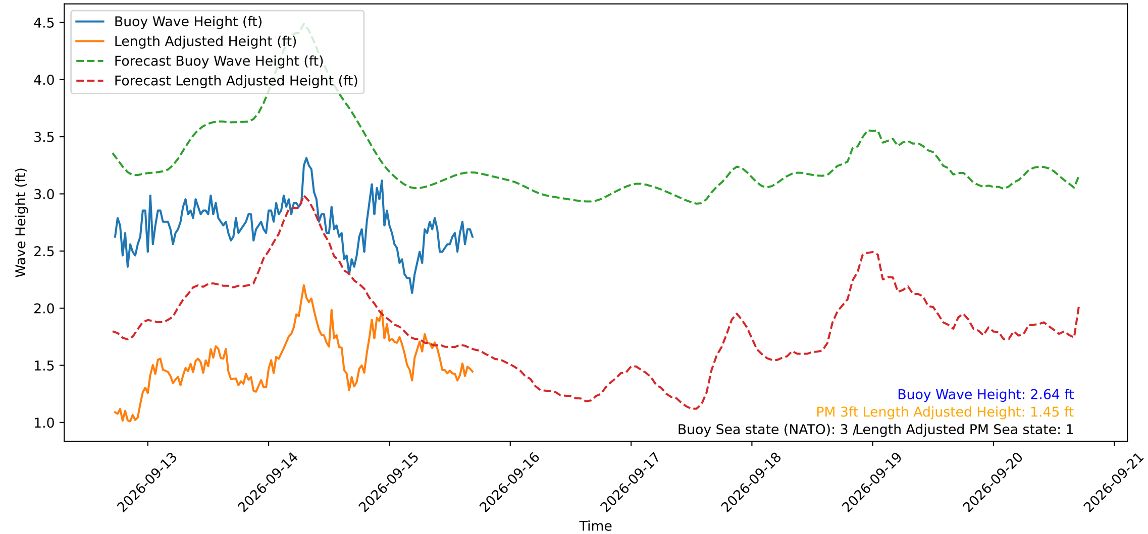
Wave Heights over Time for Green Beach at 2026-09-15 17:11:12
