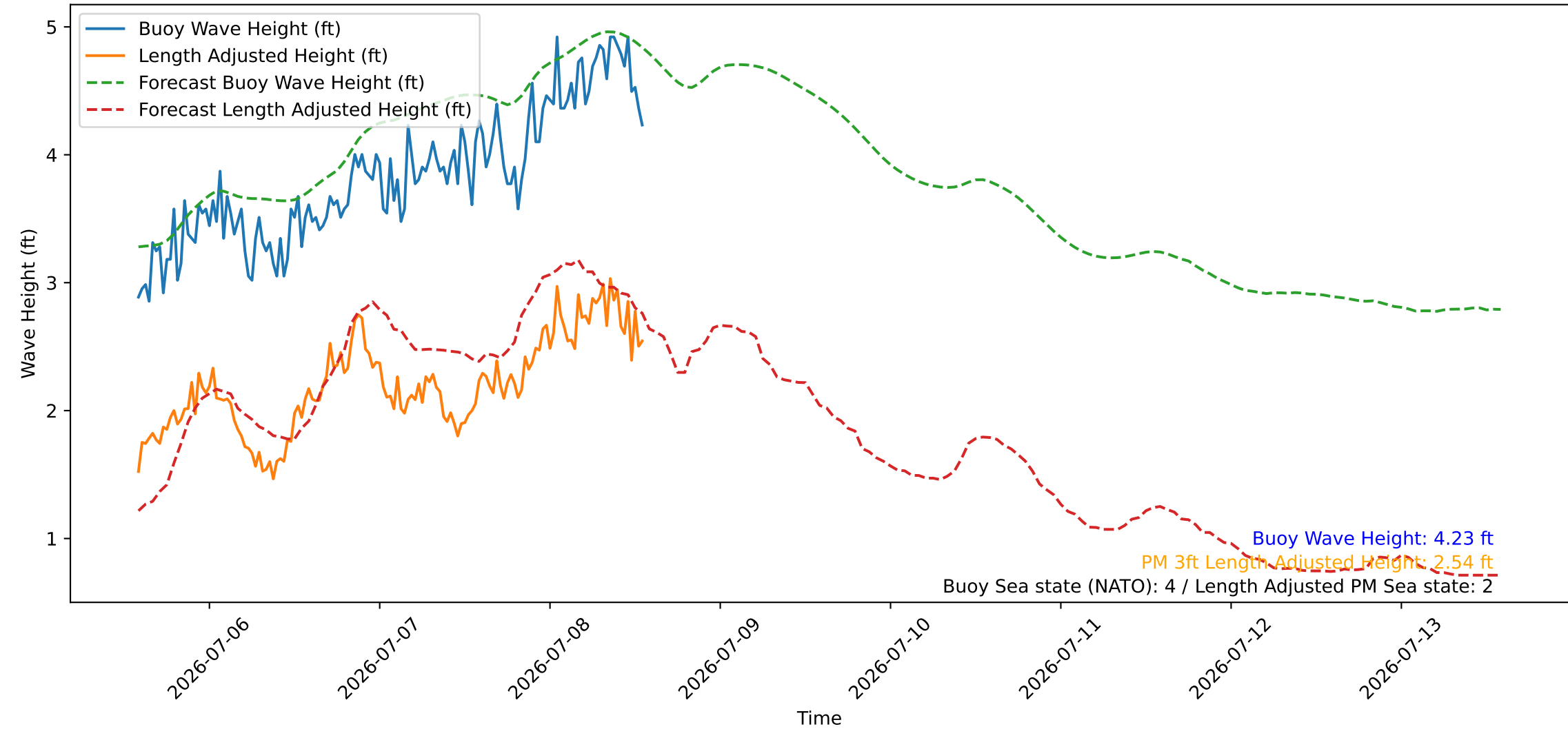
Wave Heights over Time for Oceanside Harbor at 2026-07-08 13:50:26
