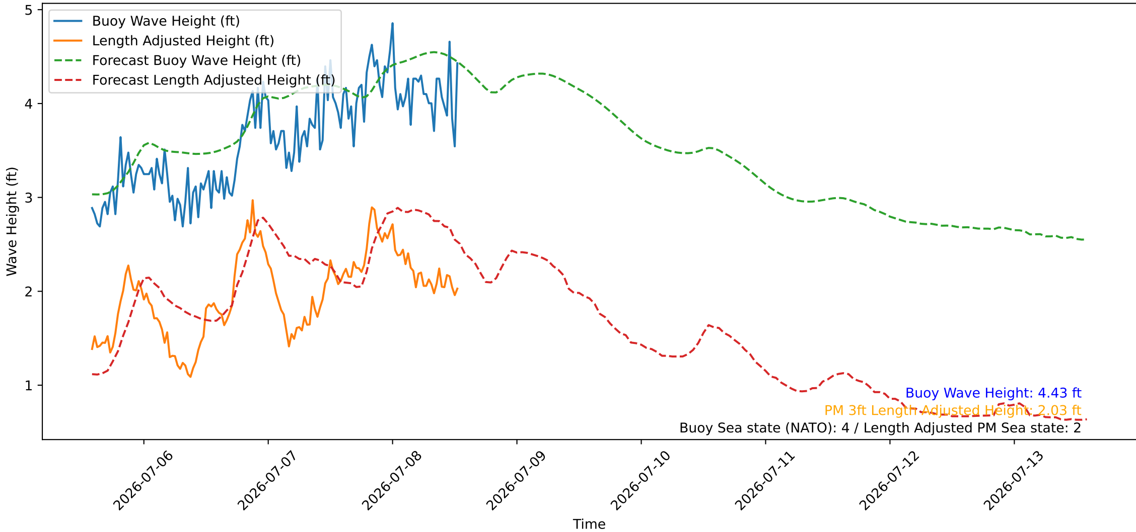
Wave Heights over Time for Red Beach at 2026-07-08 13:50:47
