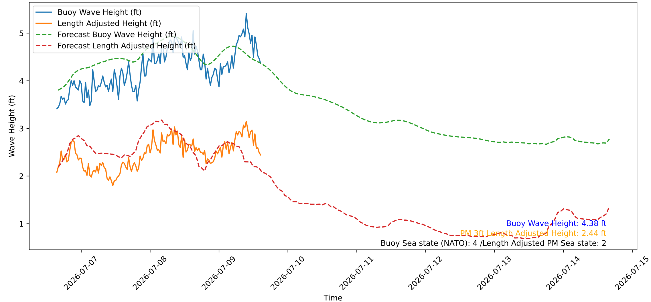
Wave Heights over Time for Oceanside Harbor at 2026-07-09 15:30:26
