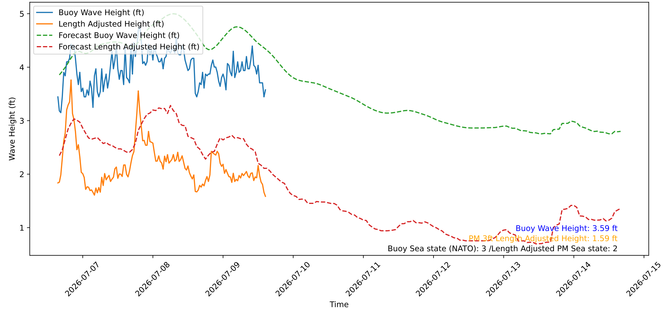
Wave Heights over Time for Green Beach at 2026-07-09 15:31:08
