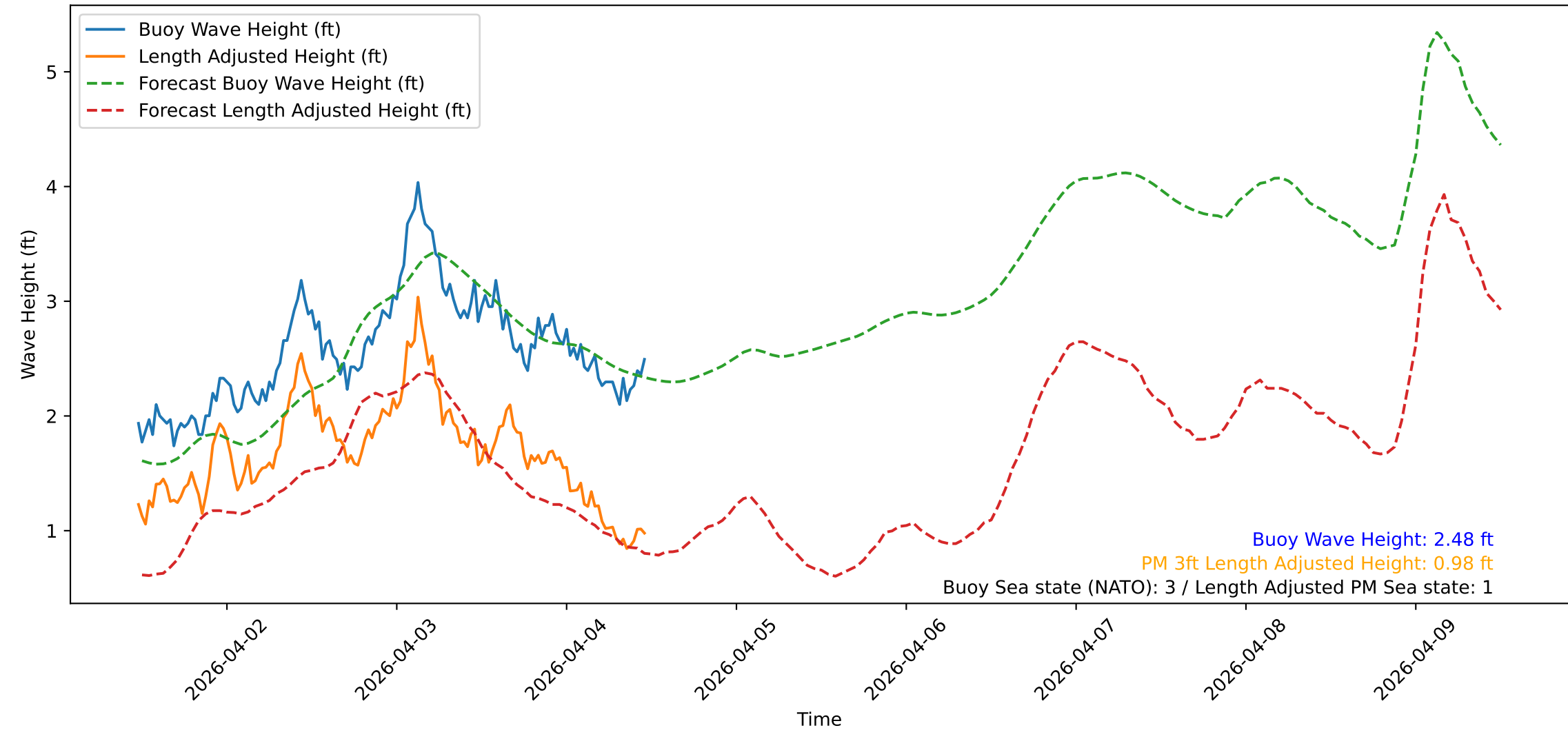
Wave Heights over Time for Oceanside Harbor at 2026-04-04 11:40:31
