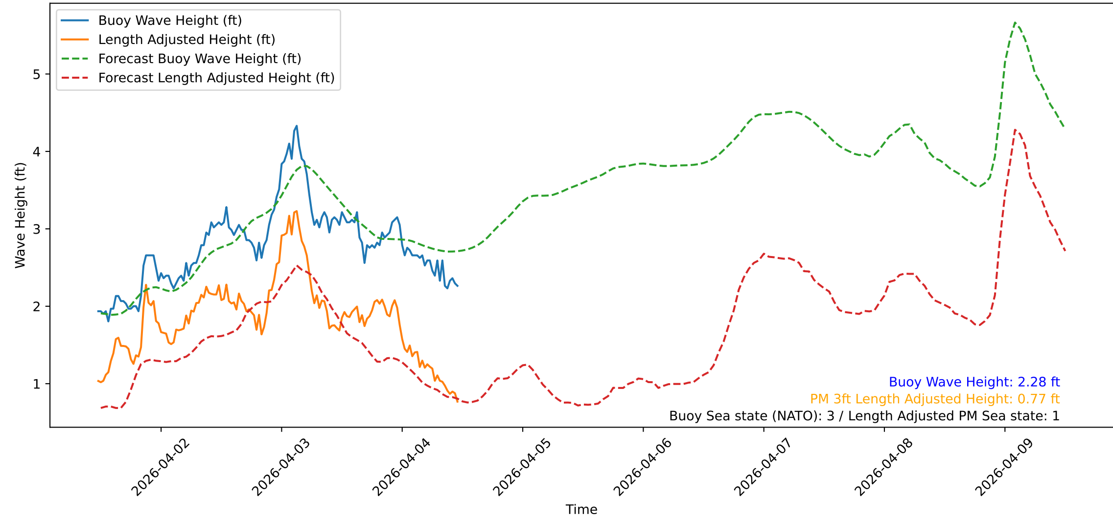
Wave Heights over Time for Green Beach at 2026-04-04 11:41:09
