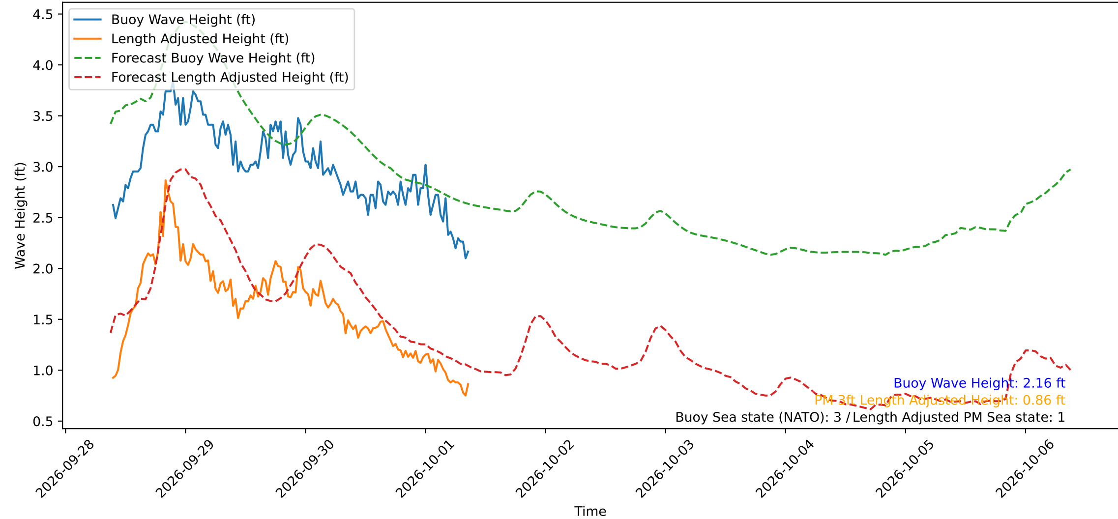
Wave Heights over Time for Red Beach at 2026-10-01 09:20:51
