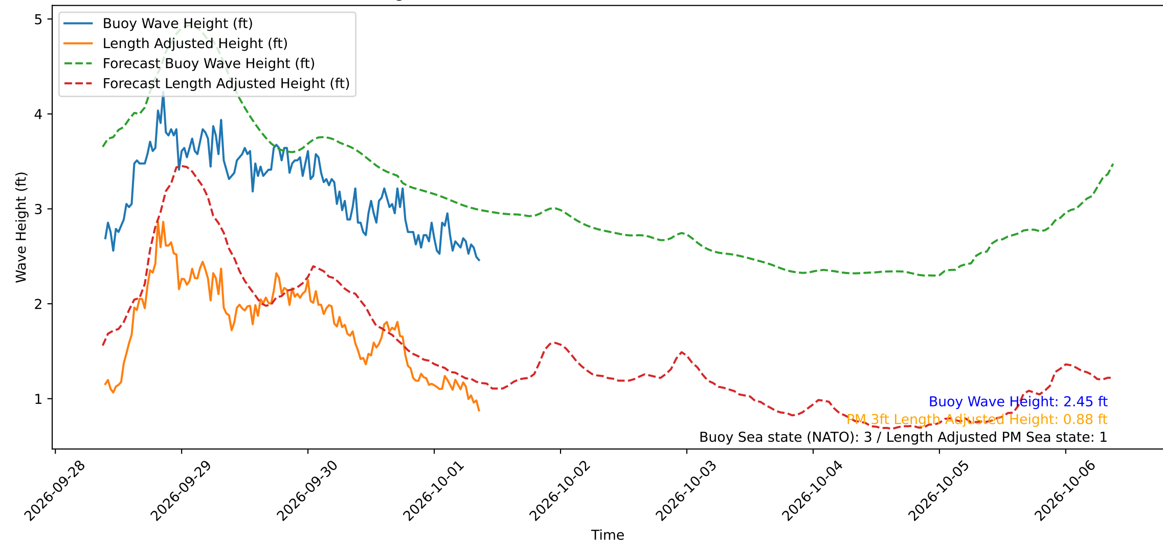
Wave Heights over Time for Oceanside Harbor at 2026-10-01 09:20:30
