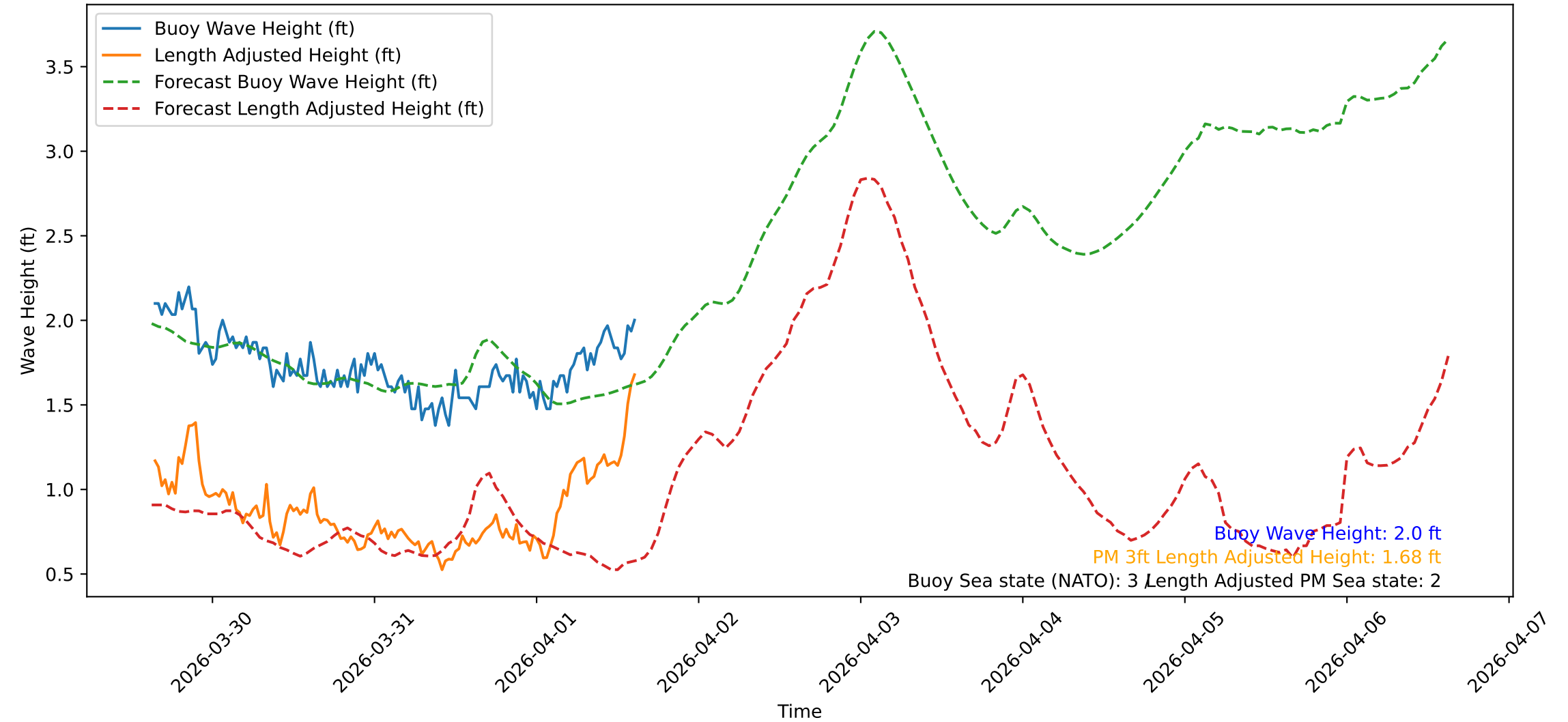
Wave Heights over Time for Red Beach at 2026-04-01 15:10:47
