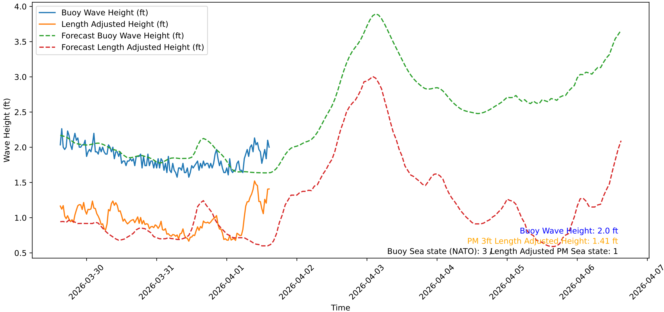
Wave Heights over Time for Oceanside Harbor at 2026-04-01 15:10:31
