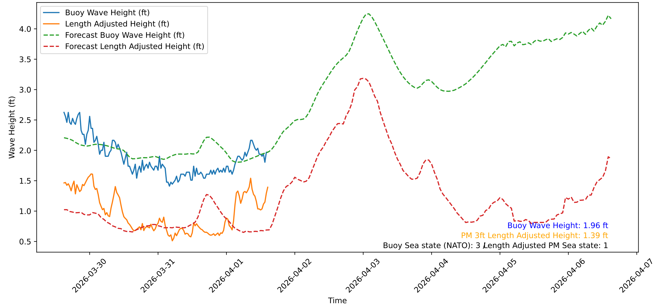
Wave Heights over Time for Green Beach at 2026-04-01 15:11:10
