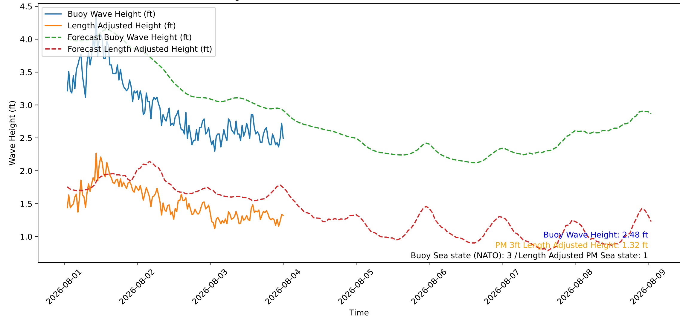
Wave Heights over Time for Oceanside Harbor at 2026-08-04 01:00:26
